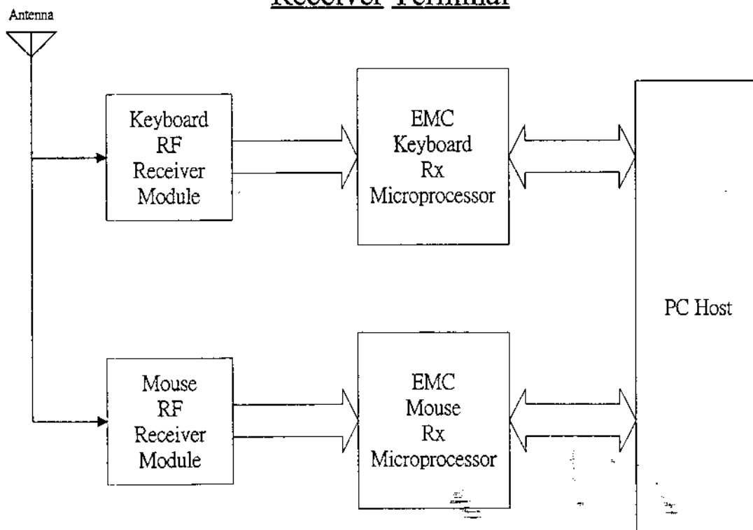
Fig.3 Receiver Block
