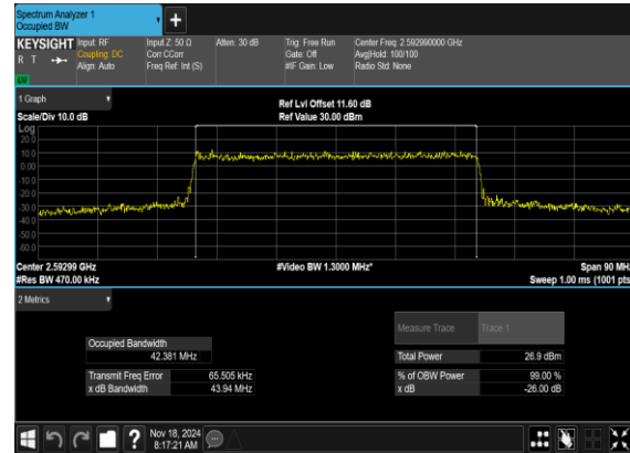
N41(45M)_CP-OFDM_16 QAM_Outer_Full_Mid_CH
