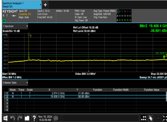
N41(40M)_CP- OFDM_QPSK_Edge_1RB_Left_Mid_CH
