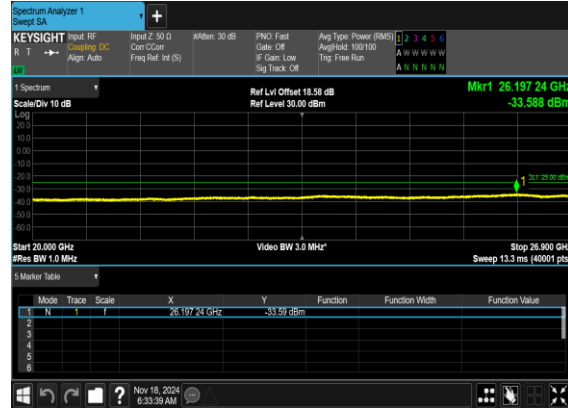
N41(40M)_CP- OFDM_QPSK_Edge_1RB_Left_Mid_CH
