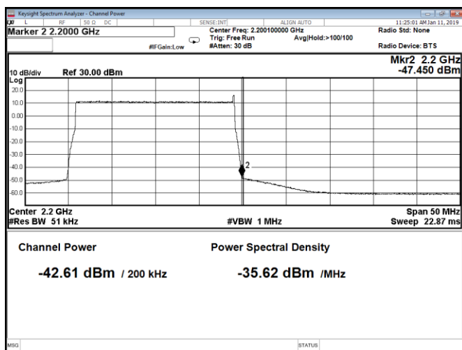
Figure 8.2-51: Conducted band edge emission at 2200 MHz, 20 MHz channel LTE + IoT operation (RBW = 1% of EBW)
