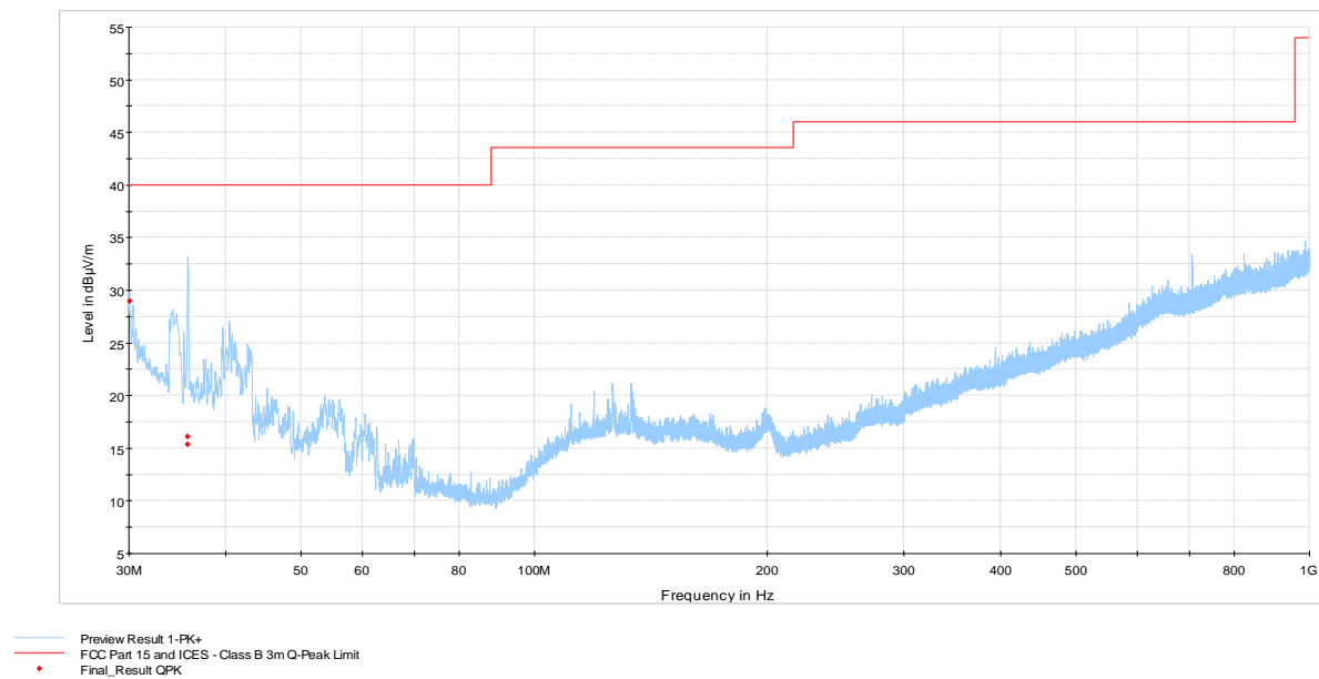
Figure 8.3-1: Radiated spurious emission below 1 GHz
