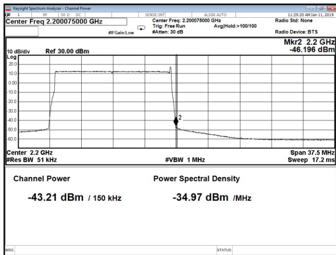
Figure 8.2-49: Conducted band edge emission at 2200 MHz, 15 MHz channel LTE + IoT operation (RBW = 1% of EBW)
