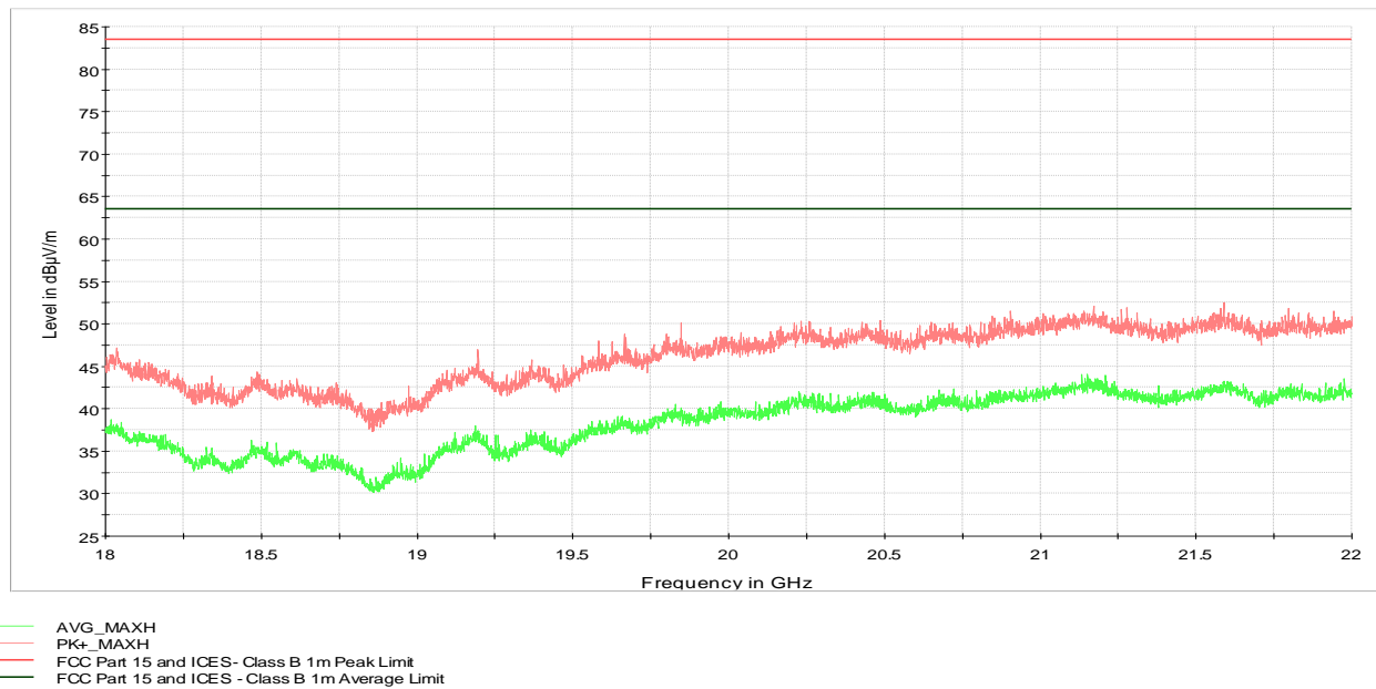
Figure 8.3-4: Radiated emissions spectral plot (18 to 22 GHz)
