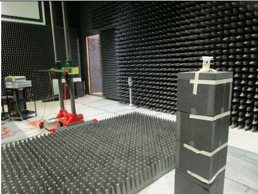
Radiated Emissions Setup Above 1 GHz
