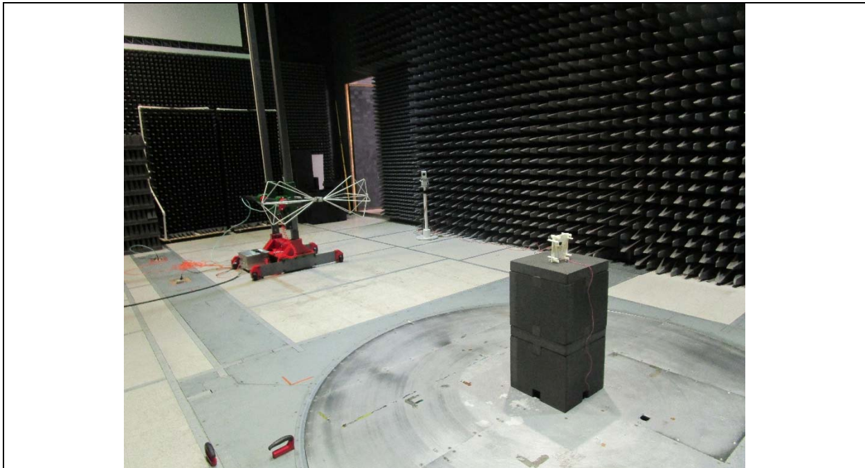
Radiated Emissions Setup Below 1 GHz
