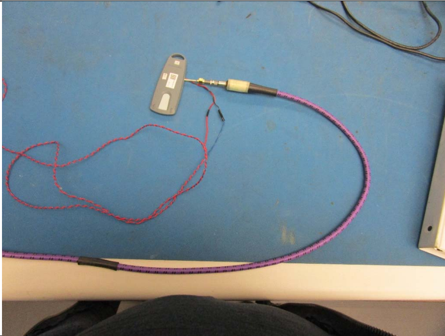
Conducted RF Measurements Setup
