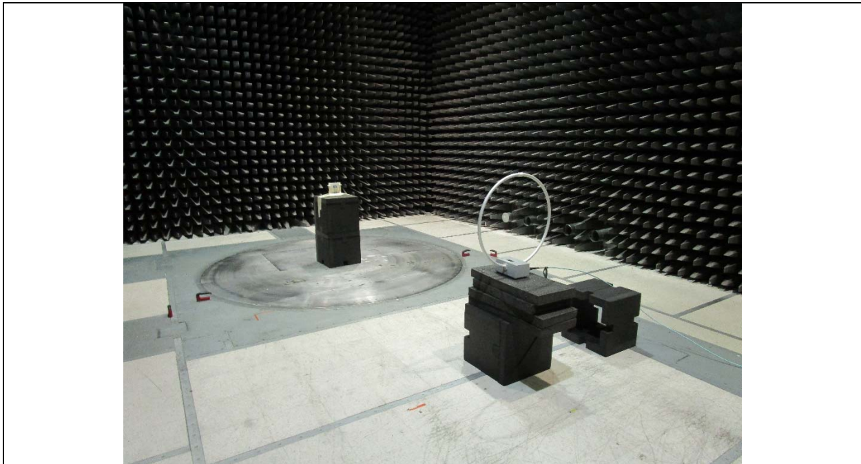
Radiated Emissions Setup Below 30 MHz
