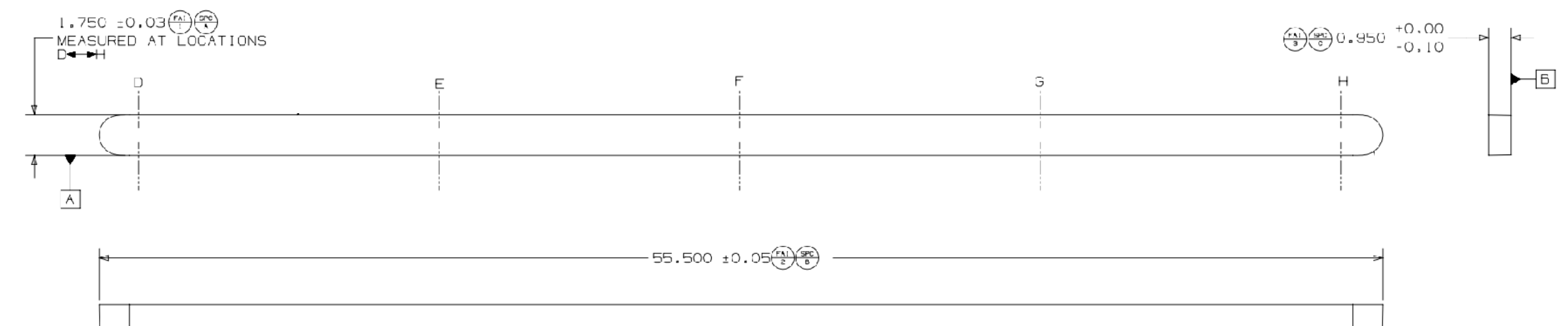
external antenna window dimensions
