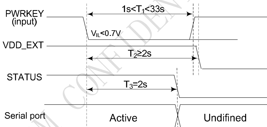
Figure 13: Timing of power off SIM868 by PWRKEY
