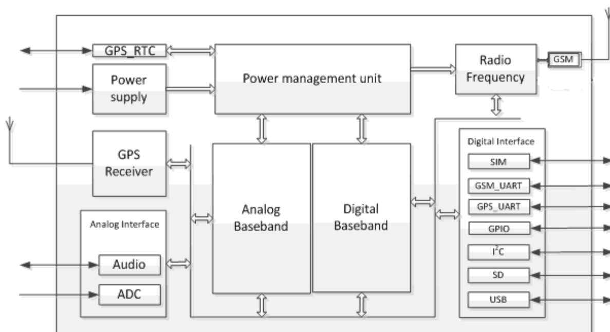
Figure 1: SIM868 functional diagram
