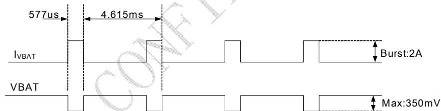
Figure 8: VBAT voltage drop during transmit burst
