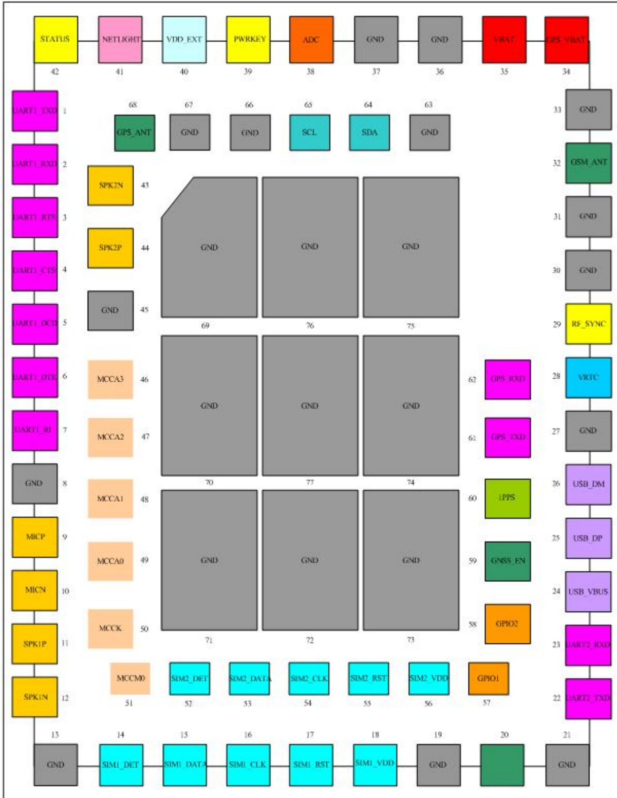
Figure 41: PIN assignment
