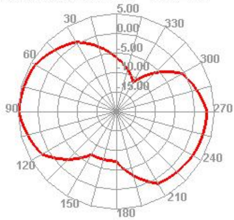
Bluetooth 0 TRP Phi=45
