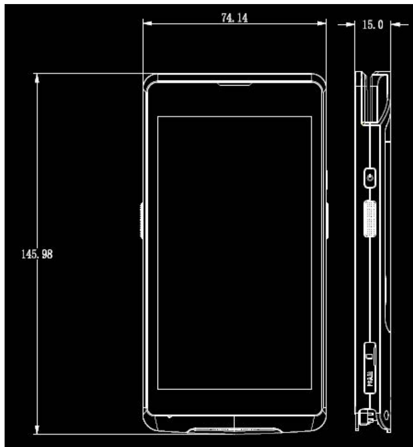
Dimensional drawing: Without scan coder
