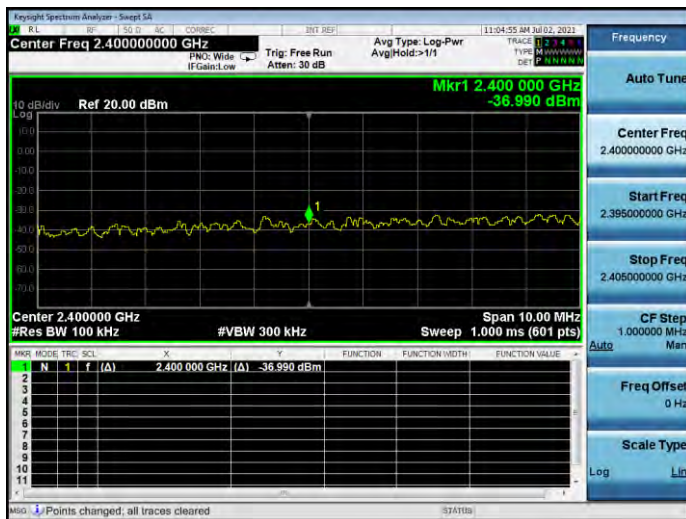
802.11n-40 MHz CHANNEL 5, Carrier level
