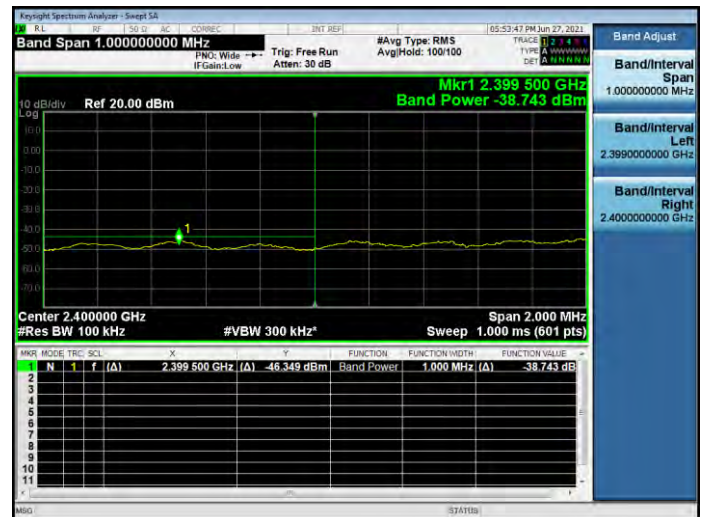
802.11n-40 MHz CHANNEL 3, Reference level
