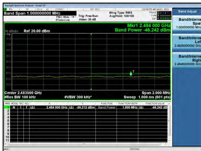
802.11n-20 MHz CHANNEL 8, Reference level
