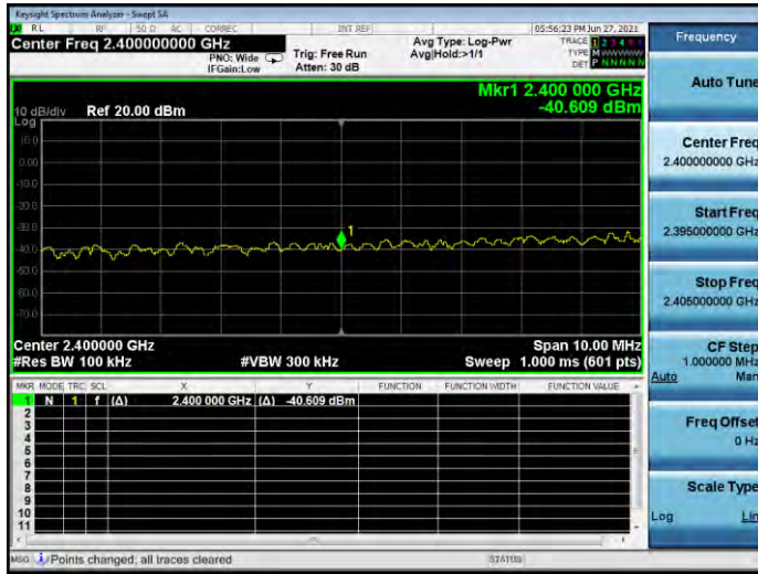
802.11n-40 MHz CHANNEL 4, Carrier level
