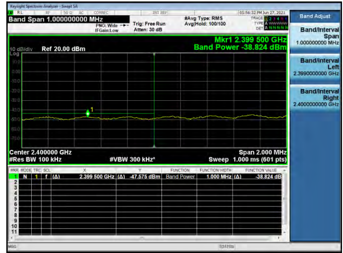
802.11n-40 MHz CHANNEL 4, Reference level
