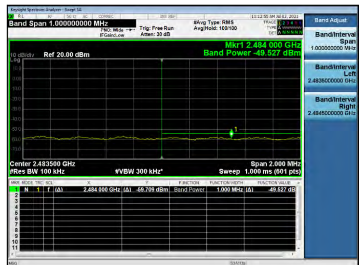
802.11n-40 MHz CHANNEL 7, Reference level
