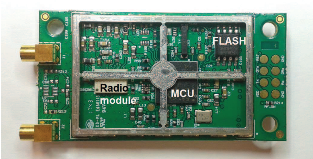
Wireless module TOP "under cover":
