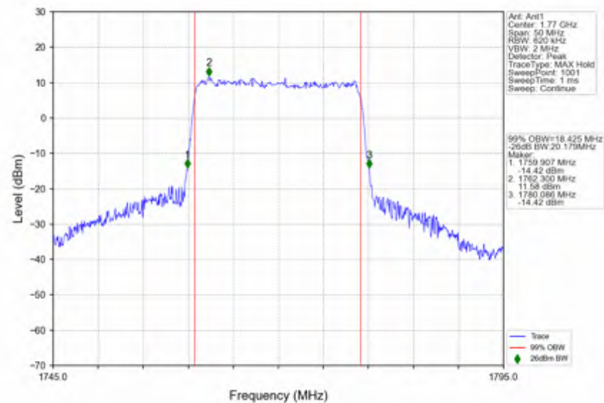
n66_30kHz_SISO_NTNV_20MHz_CP-OFDM_64_QAM_1770MHz_Outer_Full
