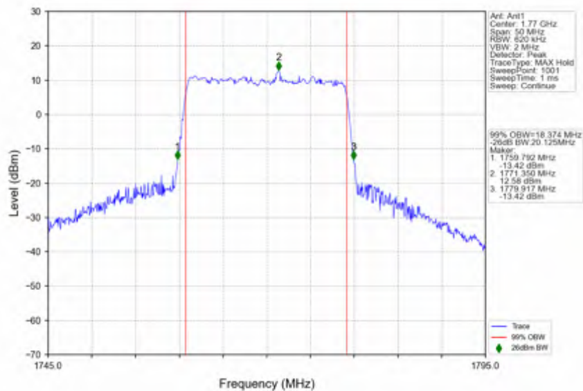
n66_30kHz_SISO_NTNV_20MHz_CP-OFDM QPSK_1770MHz_Outer_Full
