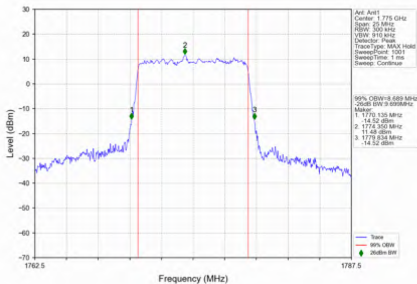
n66 30kHz SISO NTN 10MHz CP-OFDM 64 QAM 1775MHz Outer Full
