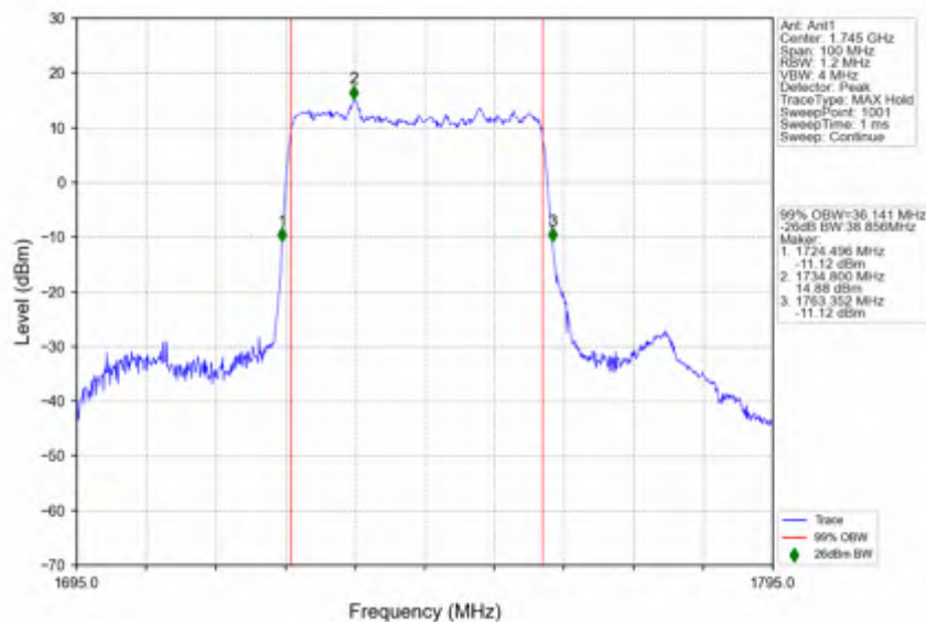
n66 30kHz SISO NTNV 40MHz DFT-s-OFDM PI/2 BPSK 1745MHz Outer Full
