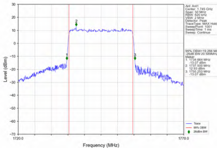
n66_15kHz_SISO_NTNV_20MHz_CP-OFDM_16_QAM_1745MHz_Outer_Full
