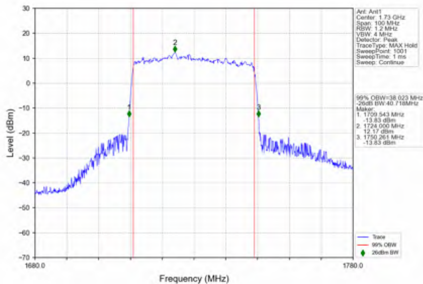
n66_30kHz_SISO_NTNV_40MHz_CP-OFDM_64_QAM_1730MHz_Outer_Full
