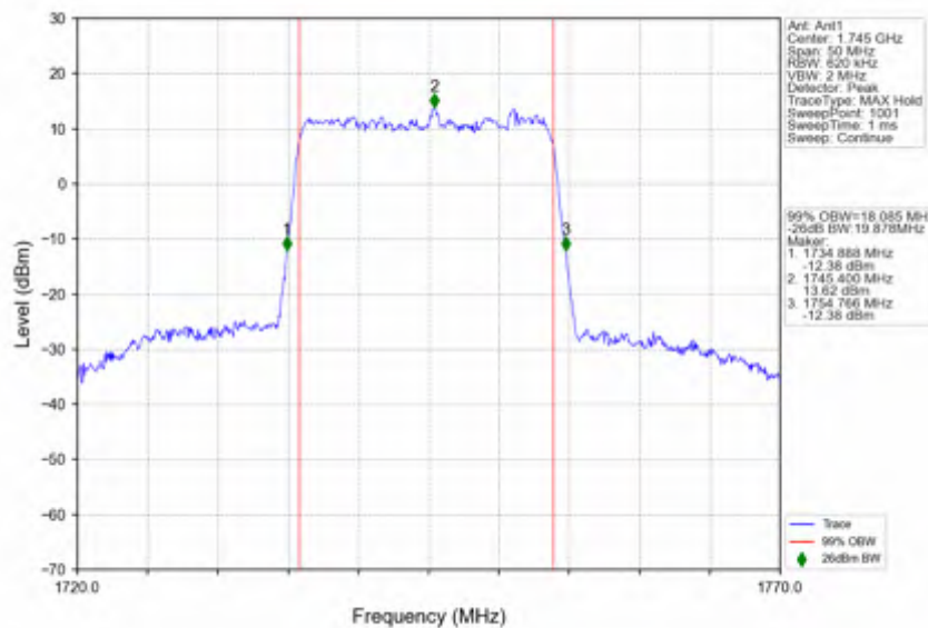
n66_30kHz_SISO_NTNV_20MHz_DFT-s-OFDM_16_QAM_1745MHz_Outer_Full
