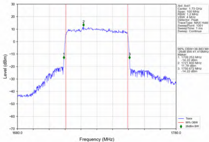
n66_15kHz_SISO_NTNV_40MHz_CP-OFDM 64 QAM_1730MHz_Outer_Full
