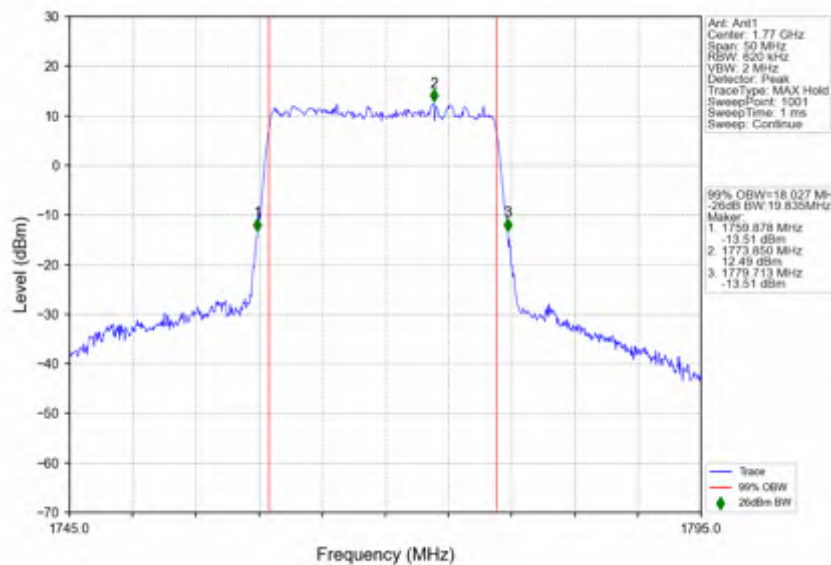
n66_30kHz_SISO_NTNV_20MHz_DFT-s-OFDM_64_QAM_1770MHz_Outer_Full
