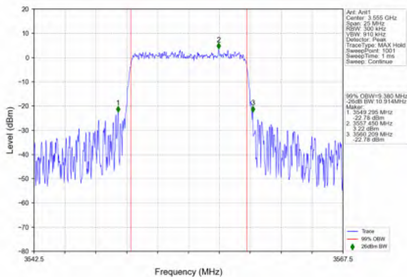
n78d_15kHz_SISO_NTNV_10MHz_CP-OFDM QPSK_3555MHz_Outer_Full
