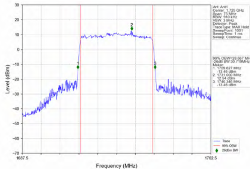
n66_15kHz_SISO_NTNV_30MHz_CP-OFDM 64 QAM_1725MHz_Outer_Full
