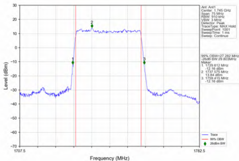
n66_30kHz_SISO_NTNV_30MHz_DFT-s-OFDM_PI/2_BPSK_1745MHz_Outer_Full
