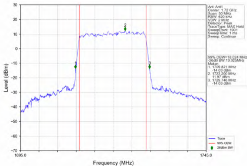
n66_30kHz_SISO_NTNV_20MHz_DFT-s-OFDM 64 QAM_1720MHz_Outer_Full
