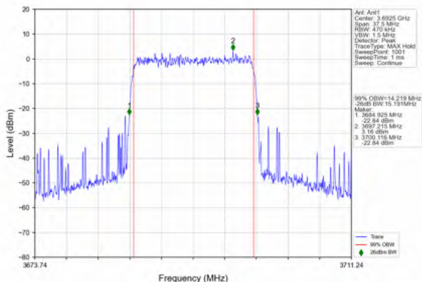
n78d_15kHz_SISO_NTNV_15MHz_CP-OFDM QPSK_3692.49MHz_Outer_Full
