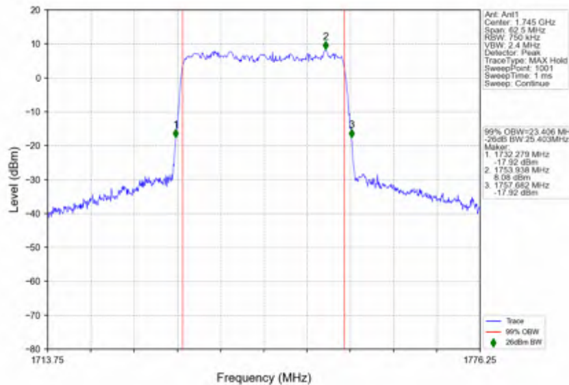
n66_30kHz_SISO_NTNV_25MHz_CP-OFDM_256_QAM_1745MHz_Outer_Full
