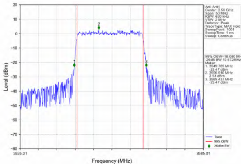
n78d_15kHz_SISO_NTNV_20MHz_DFT-s-OFDM QPSK_3560.01MHz_Outer_Full
