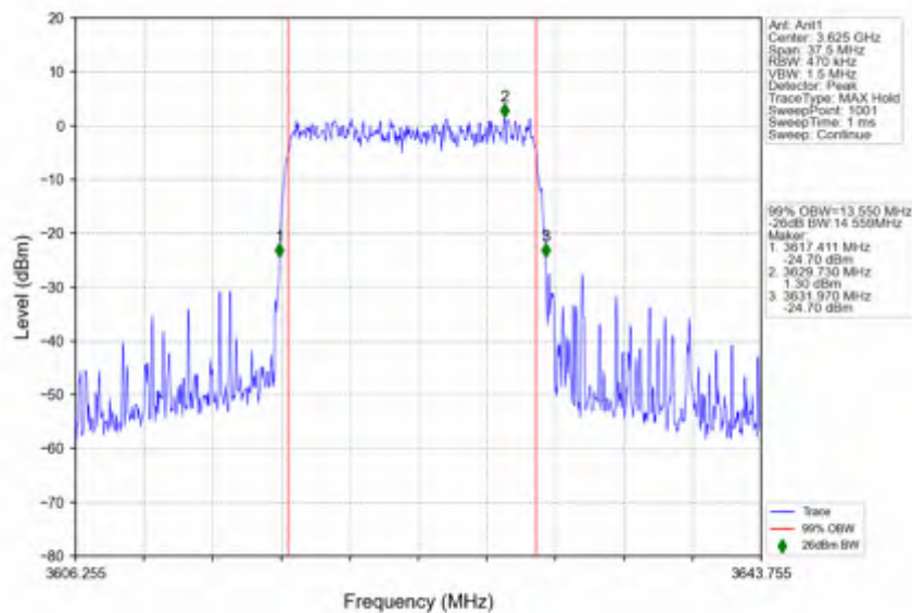
n78d_15kHz_SISO_NTNV_15MHz_DFT-s-OFDM 256 QAM_3625.005MHz_Outer_Full
