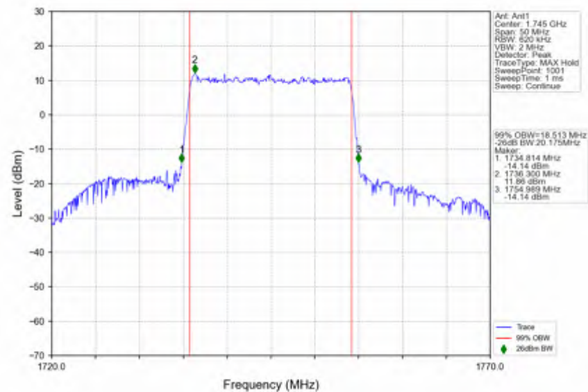
n66_30kHz_SISO_NTNV_20MHz_CP-OFDM_16_QAM_1745MHz_Outer_Full
