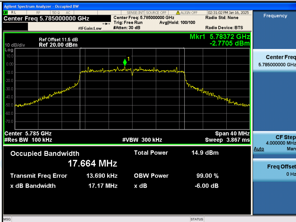
11N20SISO-Ant1-5785-PASS
