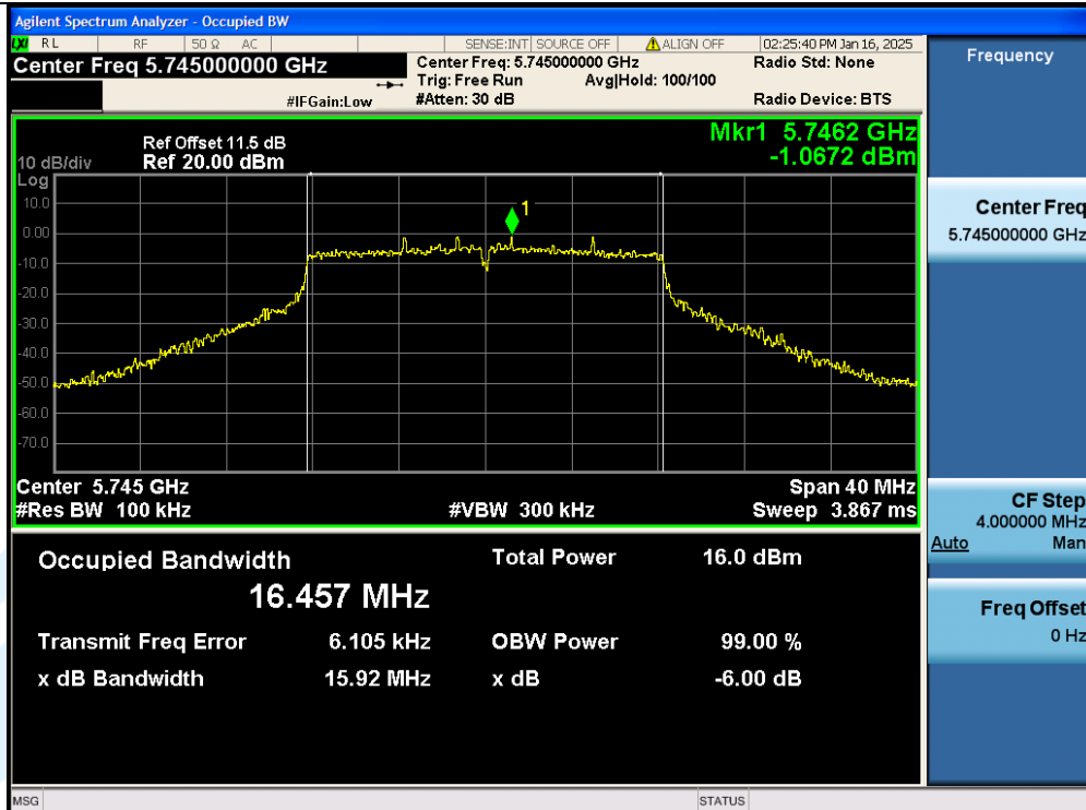
11A-Ant1-5745-PASS
