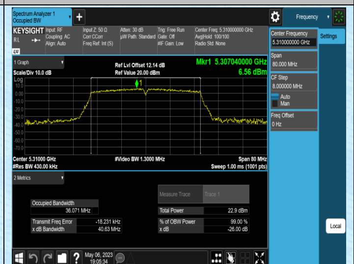
11AC40SISO-Ant2-5310
