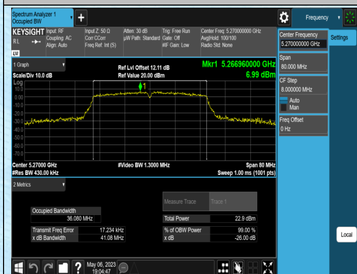
11AC40SISO-Ant2-5270
