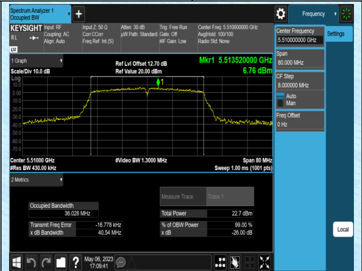
11AC40SISO-Ant1-5510
