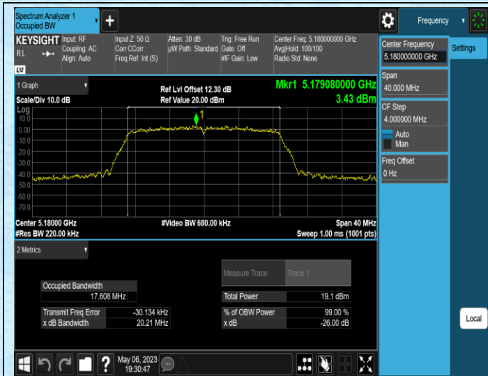
11N20MIMO-Ant1-5180
