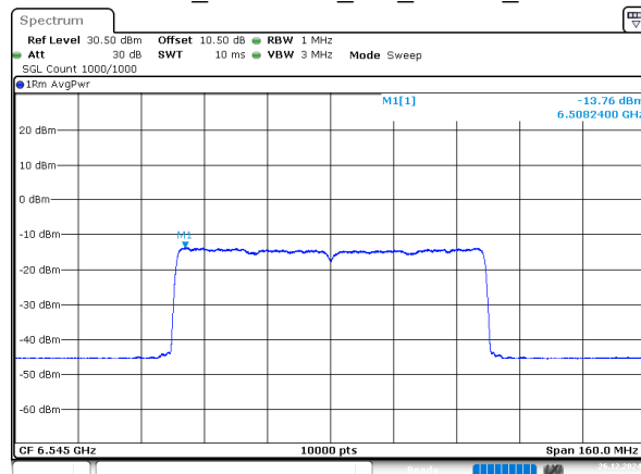
802.11ax80_6545MHz_RU_996/67_Chain 3
