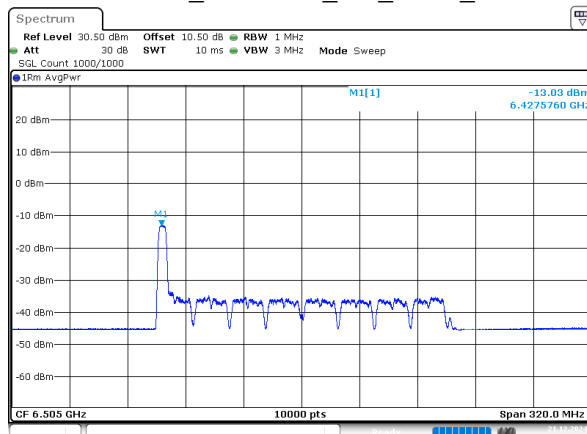
802.11ax160_6505MHz_RU_52/37_Chain 0
