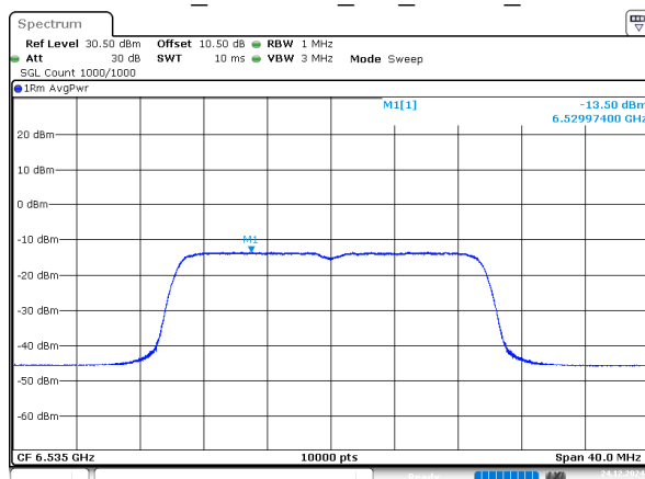
802.11ax20_6535MHz_RU_242/61_Chain 0
