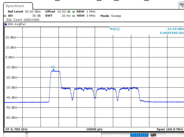
802.11ax80_6705MHz_RU_106/53_Chain 1
