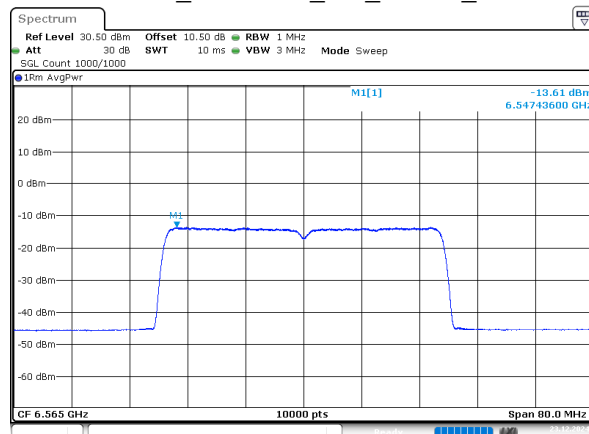
802.11ax40_6565MHz_RU_484/65_Chain 0
