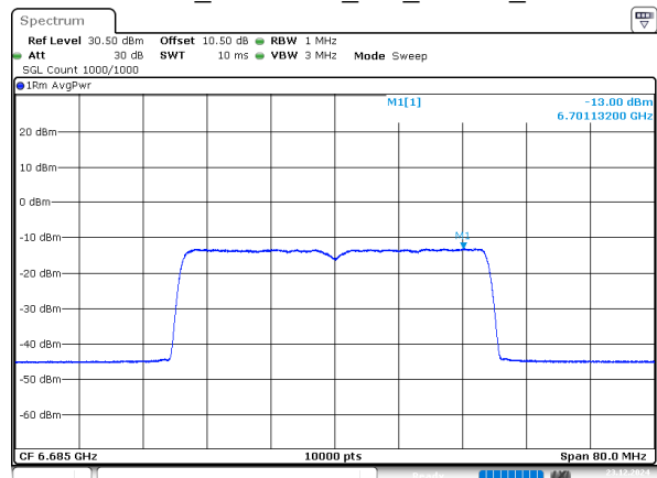
802.11ax40_6685MHz_RU_484/65_Chain 0
