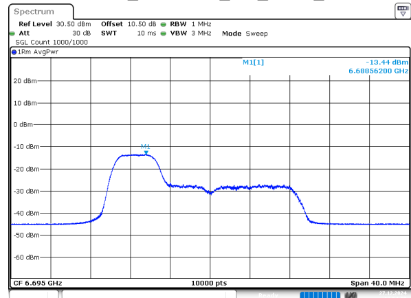
802.11ax20_6695MHz_RU_52/37_Chain 1
