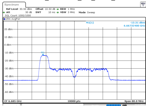
802.11ax40_6685MHz_RU_52/37_Chain 0
