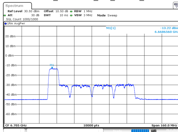
802.11ax80_6705MHz_RU_106/53_Chain 2
