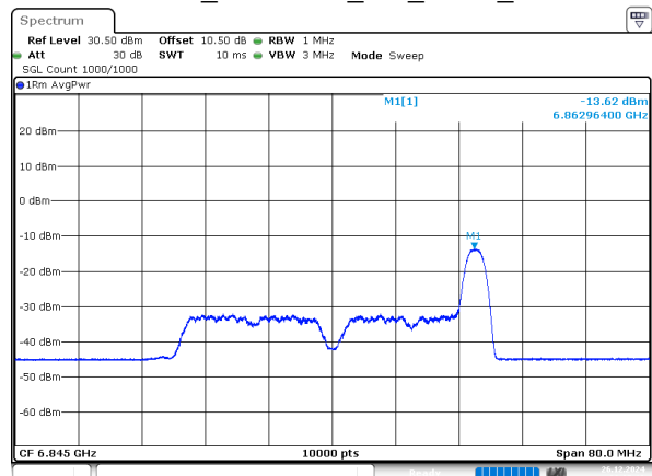
802.11ax40_6845MHz_RU_26/17_Chain 3
