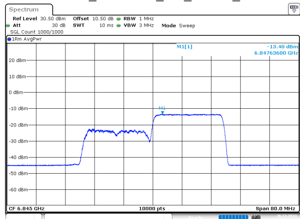
802.11ax40_6845MHz_RU_242/62_Chain 3
