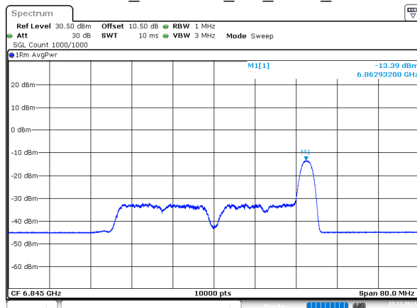
802.11ax40_6845MHz_RU_26/17_Chain 2
