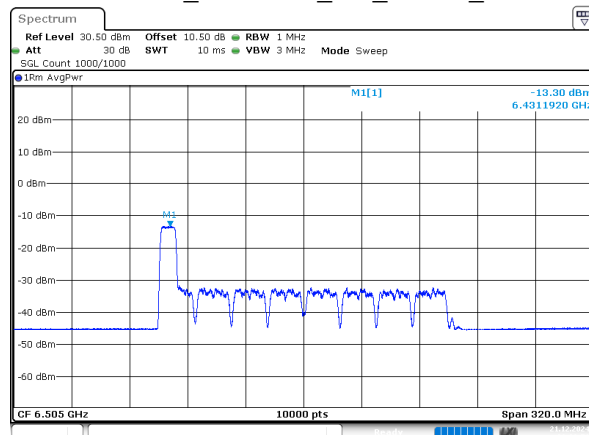
802.11ax160_6505MHz_RU_106/53_Chain 0
