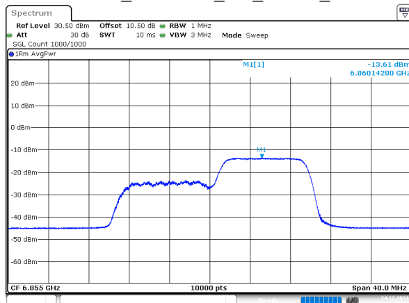
802.11ax20_6855MHz_RU_106/54_Chain 0
