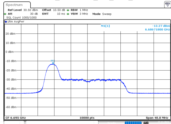
802.11ax20_6695MHz_RU_26/0_Chain 1
