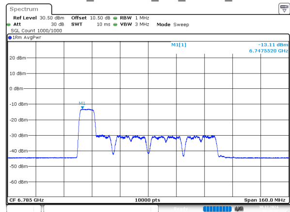
802.11ax80_6785MHz_RU_106/53_Chain 1
