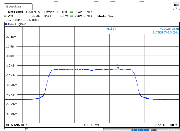
802.11ax20_6695MHz_RU_242/61_Chain 0
