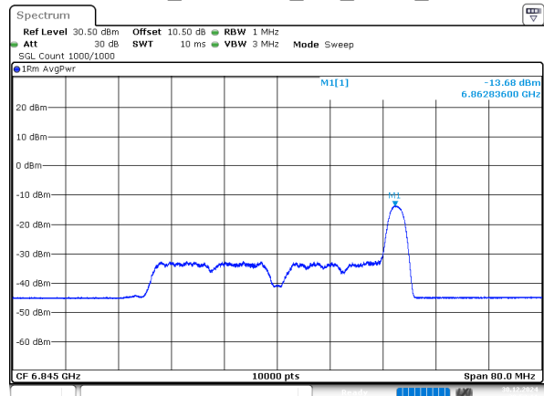
802.11ax40_6845MHz_RU_26/17_Chain 1
