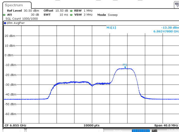
802.11ax20_6855MHz_RU_52/40_Chain 0
