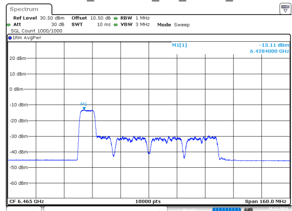
802.11ax80_6465MHz_RU_106/53_Chain 3
