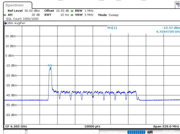
802.11ax160_6505MHz_RU_52/37_Chain 2
