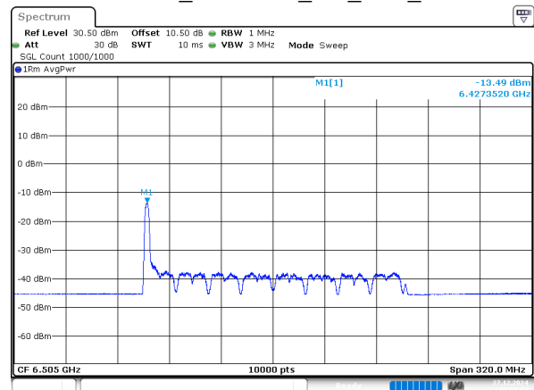
802.11ax160_6505MHz_RU_26/0_Chain 3
