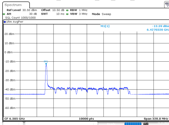
802.11ax160_6505MHz_RU_26/0_Chain 0
