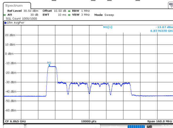
802.11ax80_6865MHz_RU_106/53_Chain 2
