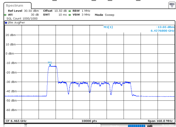
802.11ax80_6465MHz_RU_106/53_Chain 2
