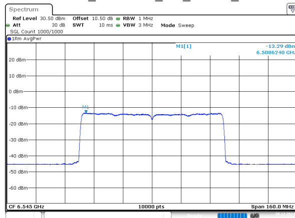
802.11ax80_6545MHz_RU_996/67_Chain 2
