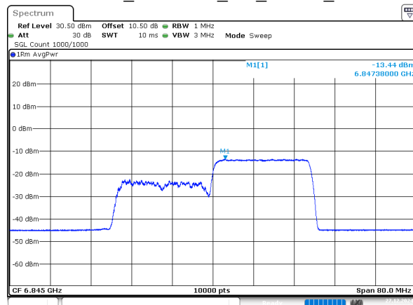
802.11ax40_6845MHz_RU_242/62_Chain 2
