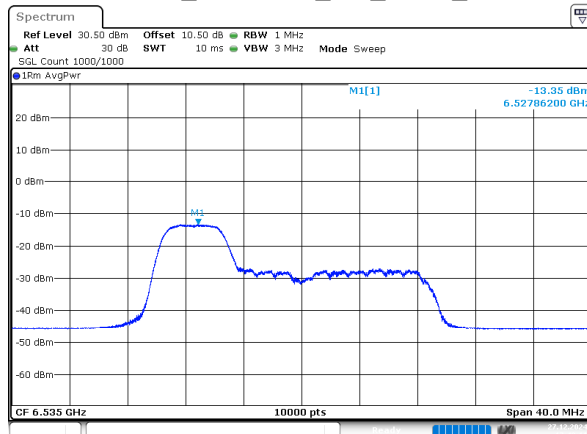
802.11ax20_6535MHz_RU_52/37_Chain 1
