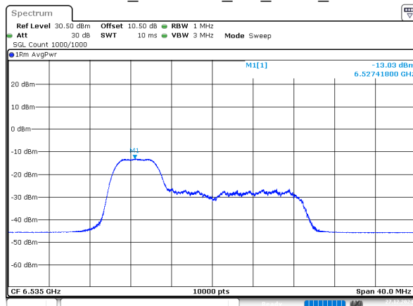
802.11ax20_6535MHz_RU_52/37_Chain 2
