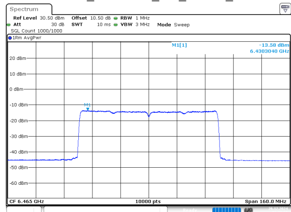
802.11ax80_6465MHz_RU_996/67_Chain 3
