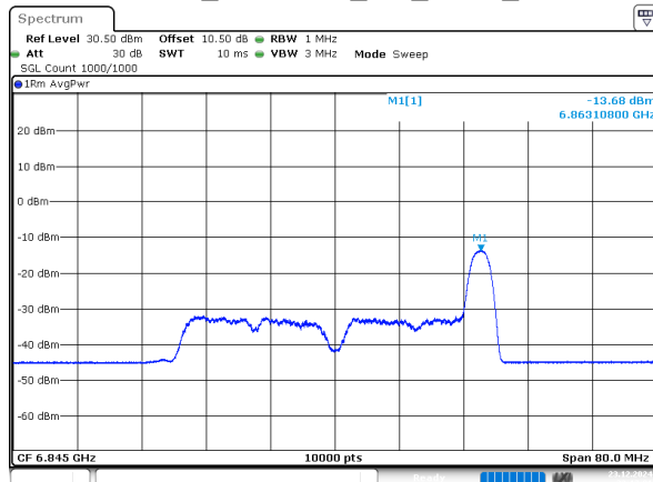
802.11ax40_6845MHz_RU_26/17_Chain 0
