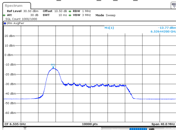
802.11ax20_6535MHz_RU_26/0_Chain 3
