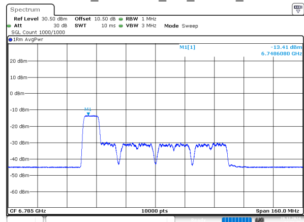
802.11ax80_6785MHz_RU_106/53_Chain 2
