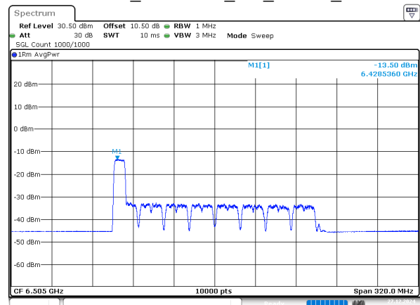
802.11ax160_6505MHz_RU_106/53_Chain 3
