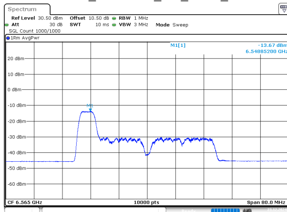
802.11ax40_6565MHz_RU_52/37_Chain 0
