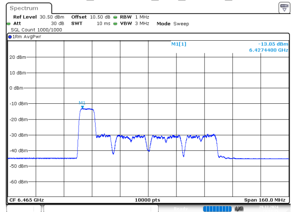
802.11ax80_6465MHz_RU_106/53_Chain 1
