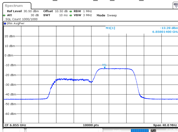
802.11ax20_6855MHz_RU_106/54_Chain 2
