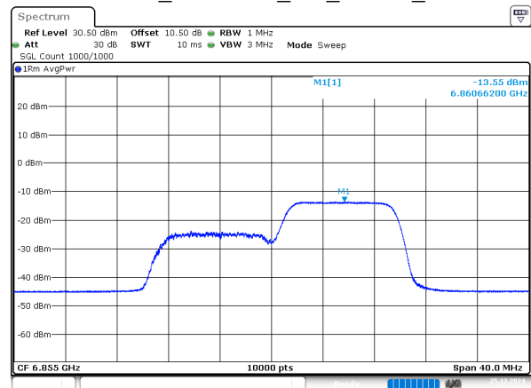
802.11ax20_6855MHz_RU_106/54_Chain 3
