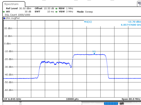
802.11ax40_6845MHz_RU_242/62_Chain 0
