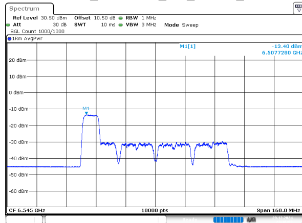
802.11ax80_6545MHz_RU_106/53_Chain 1
