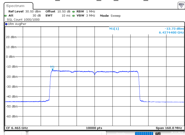
802.11ax80_6465MHz_RU_996/67_Chain 2
