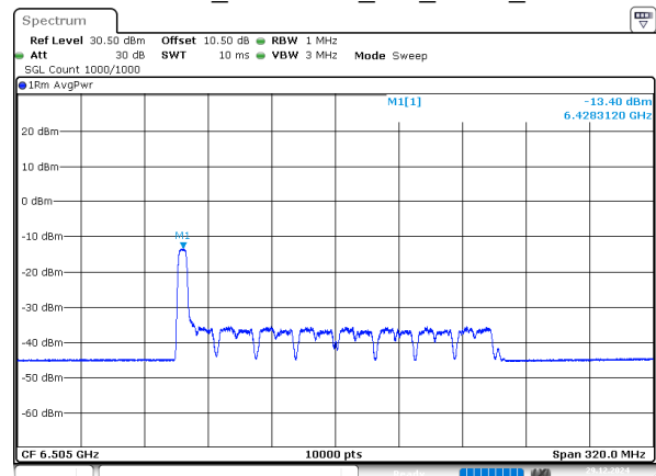
802.11ax160_6505MHz_RU_52/37_Chain 1
