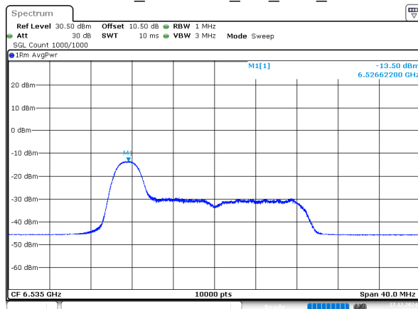
802.11ax20_6535MHz_RU_26/0_Chain 2
