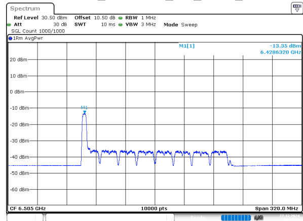
802.11ax160_6505MHz_RU_52/37_Chain 3
