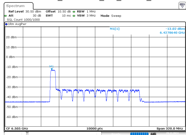
802.11ax160_6505MHz_RU_106/53_Chain 1
