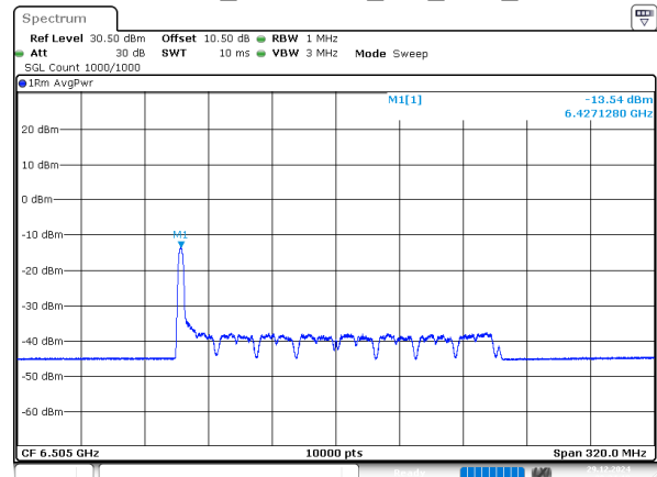
802.11ax160_6505MHz_RU_26/0_Chain 1
