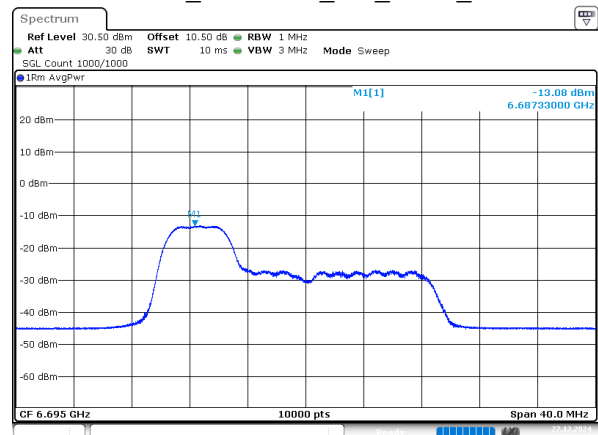
802.11ax20_6695MHz_RU_52/37_Chain 2
