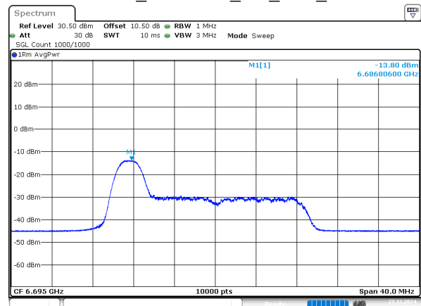
802.11ax20_6695MHz_RU_26/0_Chain 2
