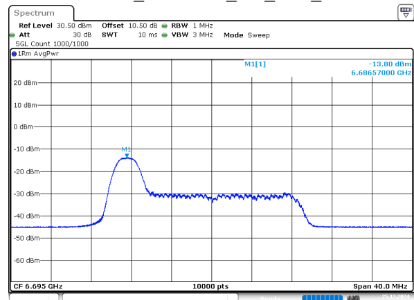
802.11ax20_6695MHz_RU_26/0_Chain 3
