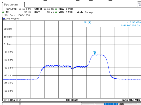
802.11ax20_6855MHz_RU_52/40_Chain 2
