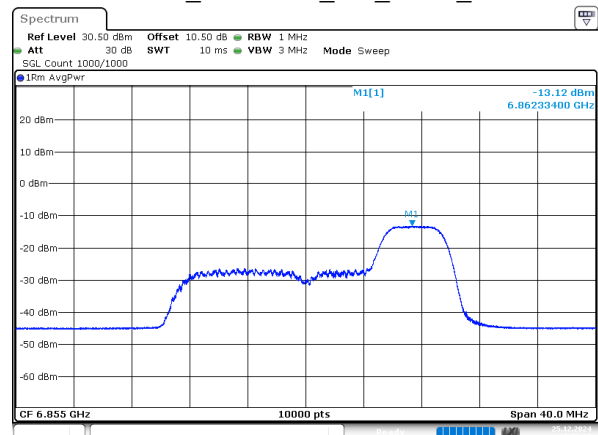
802.11ax20_6855MHz_RU_52/40_Chain 3
