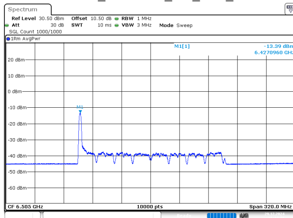
802.11ax160_6505MHz_RU_26/0_Chain 2
