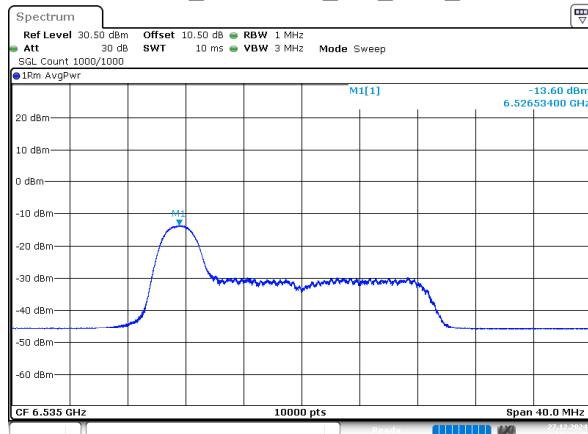
802.11ax20_6535MHz_RU_26/0_Chain 1
