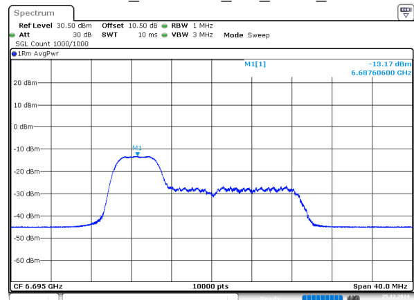
802.11ax20_6695MHz_RU_52/37_Chain 3
