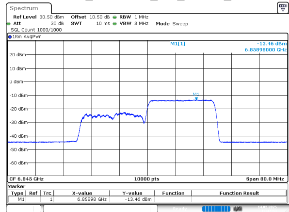
802.11ax40_6845MHz_RU_242/62_Chain 1
