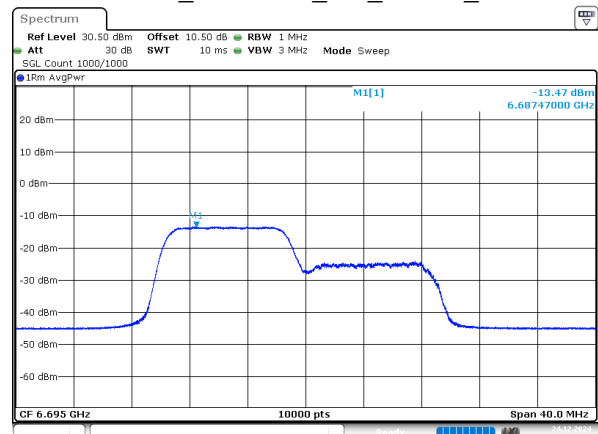
802.11ax20_6695MHz_RU_106/53_Chain 0
