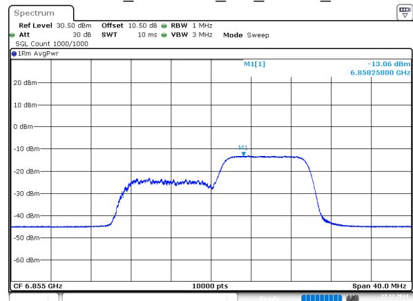
802.11ax20_6855MHz_RU_106/54_Chain 1
