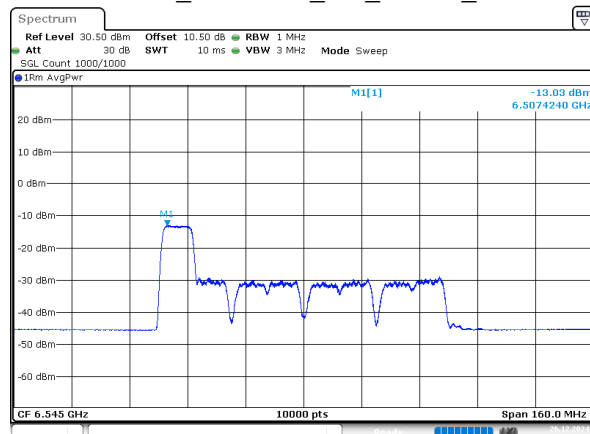
802.11ax80_6545MHz_RU_106/53_Chain 3
