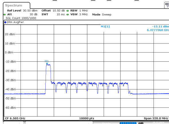
802.11ax160_6505MHz_RU_106/53_Chain 2
