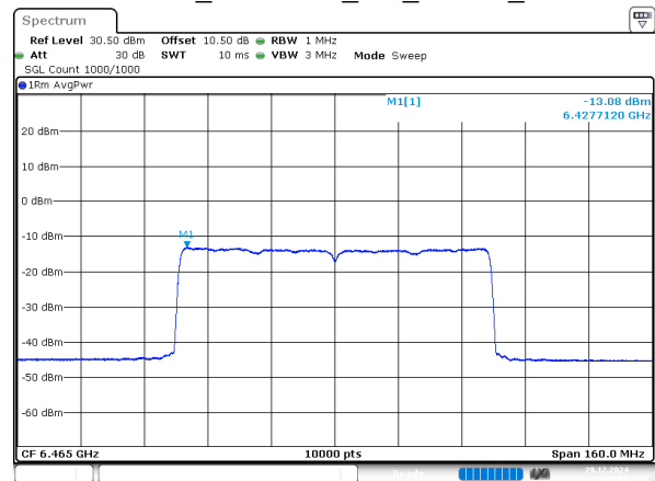
802.11ax80_6465MHz_RU_996/67_Chain 1
