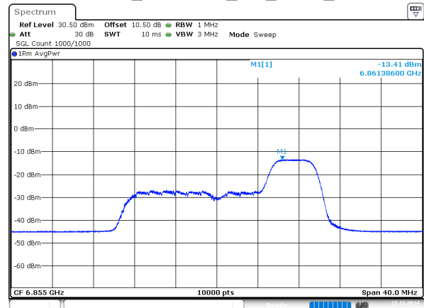
802.11ax20_6855MHz_RU_52/40_Chain 1
