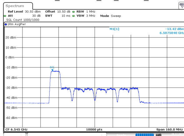
802.11ax80_6545MHz_RU_106/53_Chain 2
