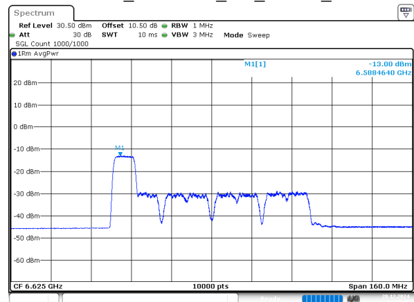
802.11ax80_6625MHz_RU_106/53_Chain 2
