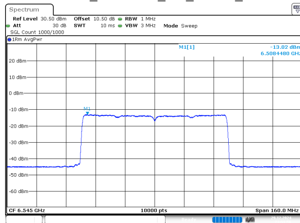
802.11ax80_6545MHz_RU_996/67_Chain 1
