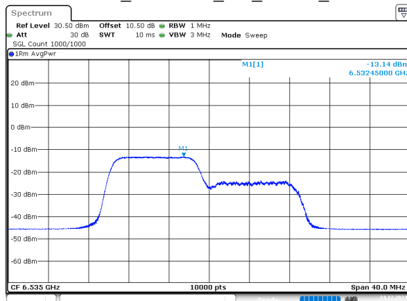
802.11ax20_6535MHz_RU_106/53_Chain 0
