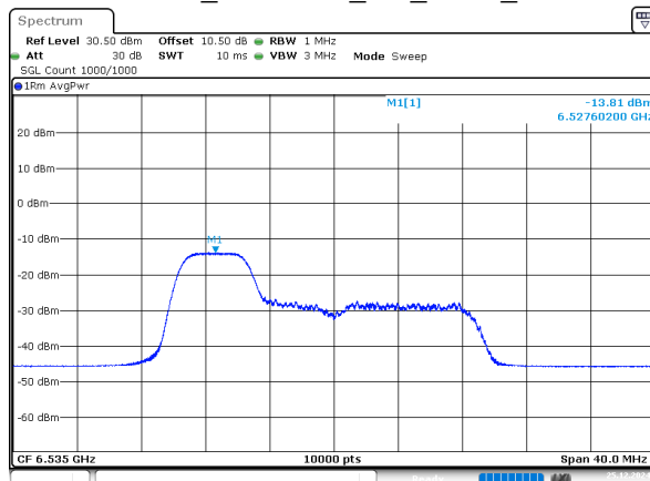
802.11ax20_6535MHz_RU_52/37_Chain 3
