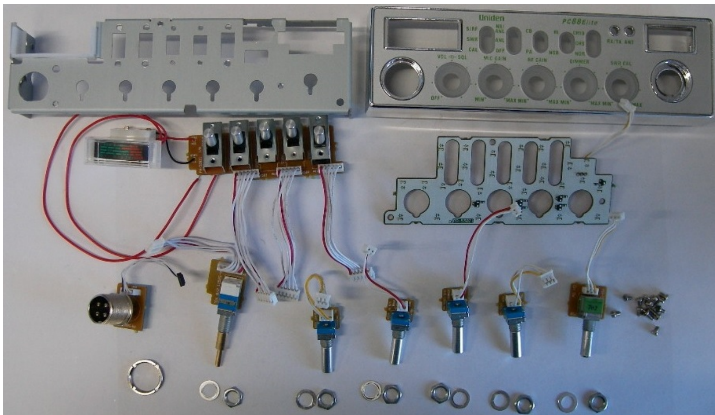
Figure E13.5 – Internal Photo – Front Control Assembly – Component View
