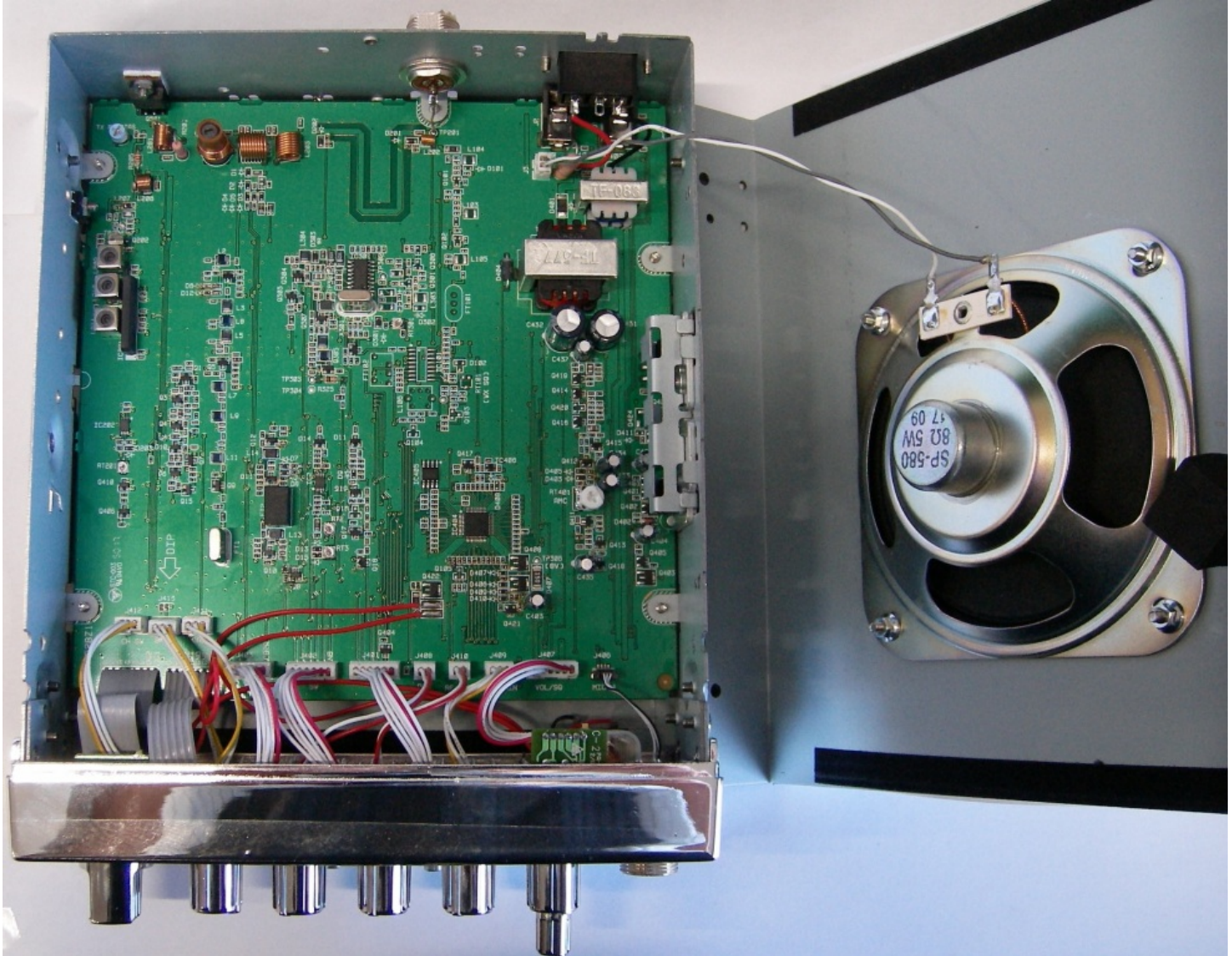
Figure E13.1 – Internal Photo - DUT w/ Bottom Cover Removed
