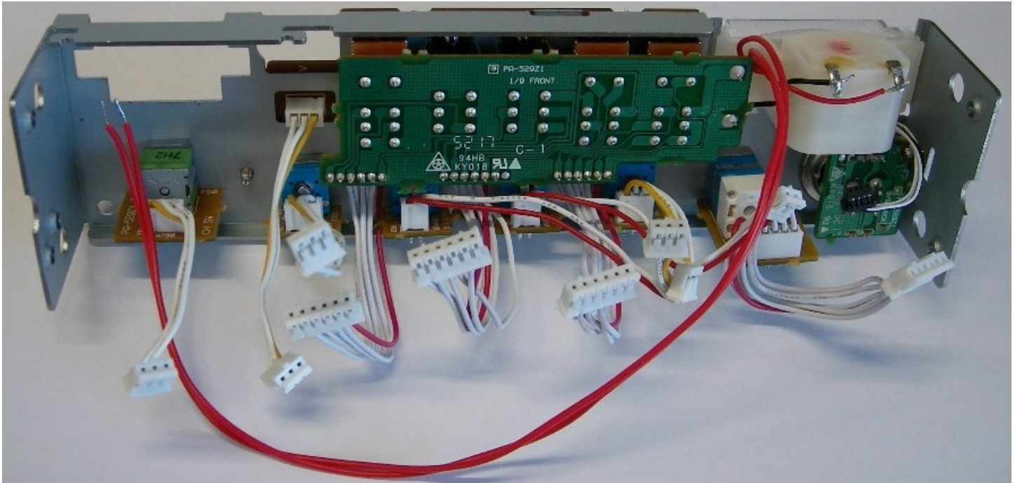
Figure E13.3 – Internal Photo – Front Control Assembly – Rear View
