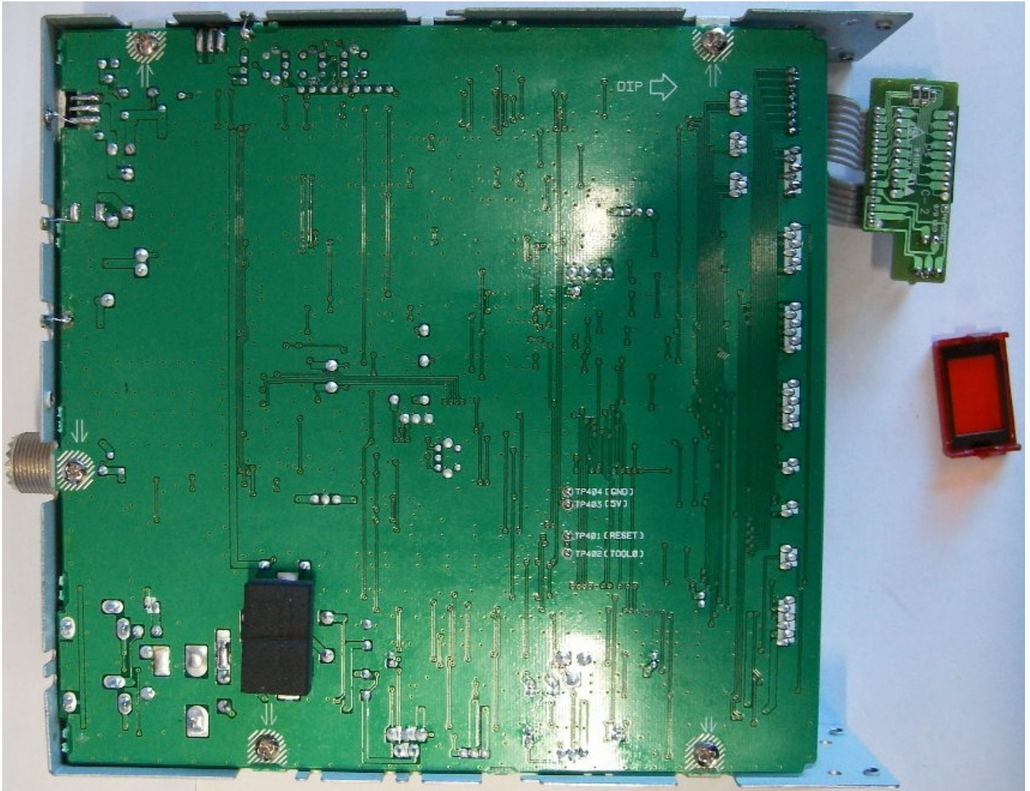
Figure E13.7 – Internal Photo – PCB – Bottom View
