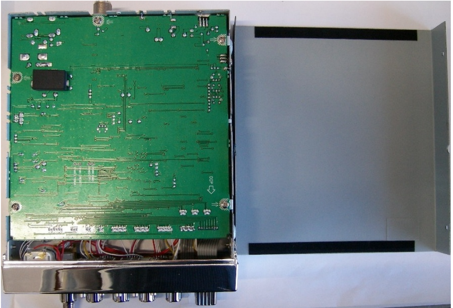
Figure E13.2 – Internal Photo – DUT w/ Top Cover Removed
