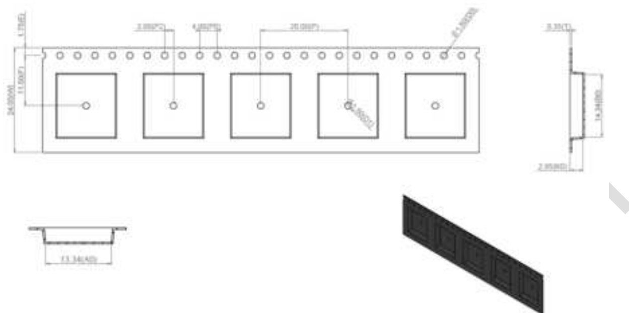
Figure 14: RM126x Carrier Tape Specifications
