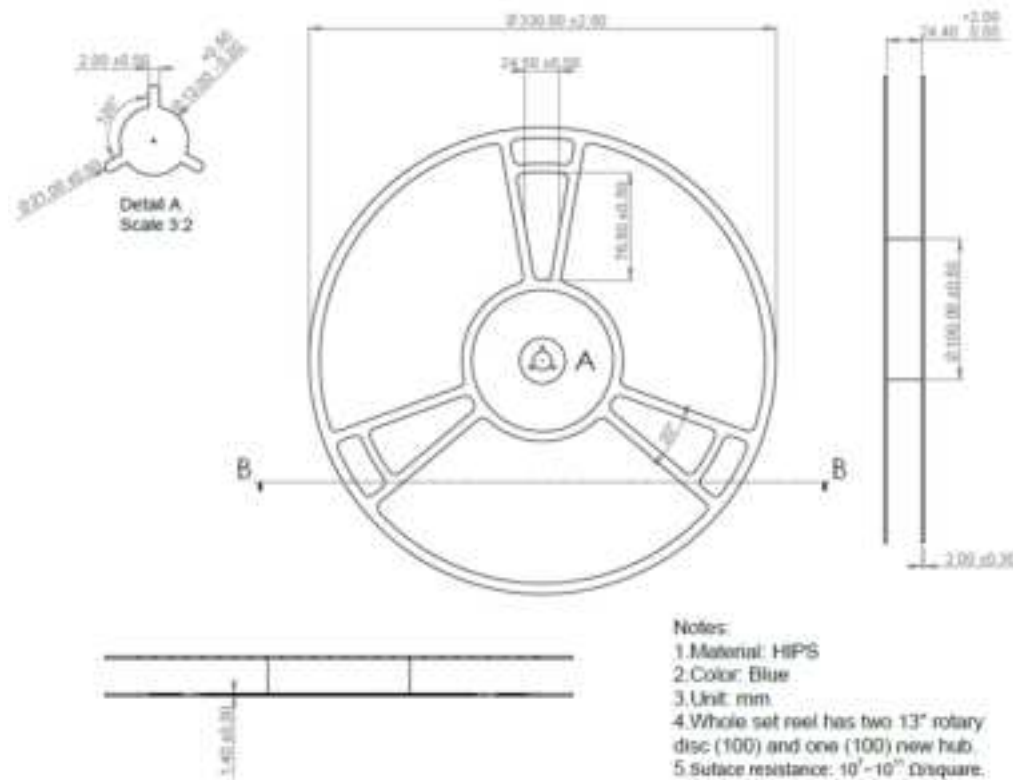
Figure 13 Reel Specifications
