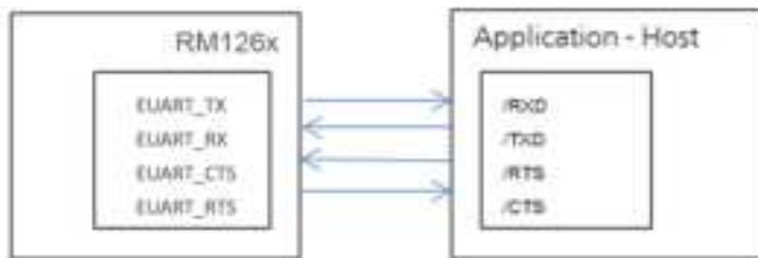
Figure 5: EUART Signals
