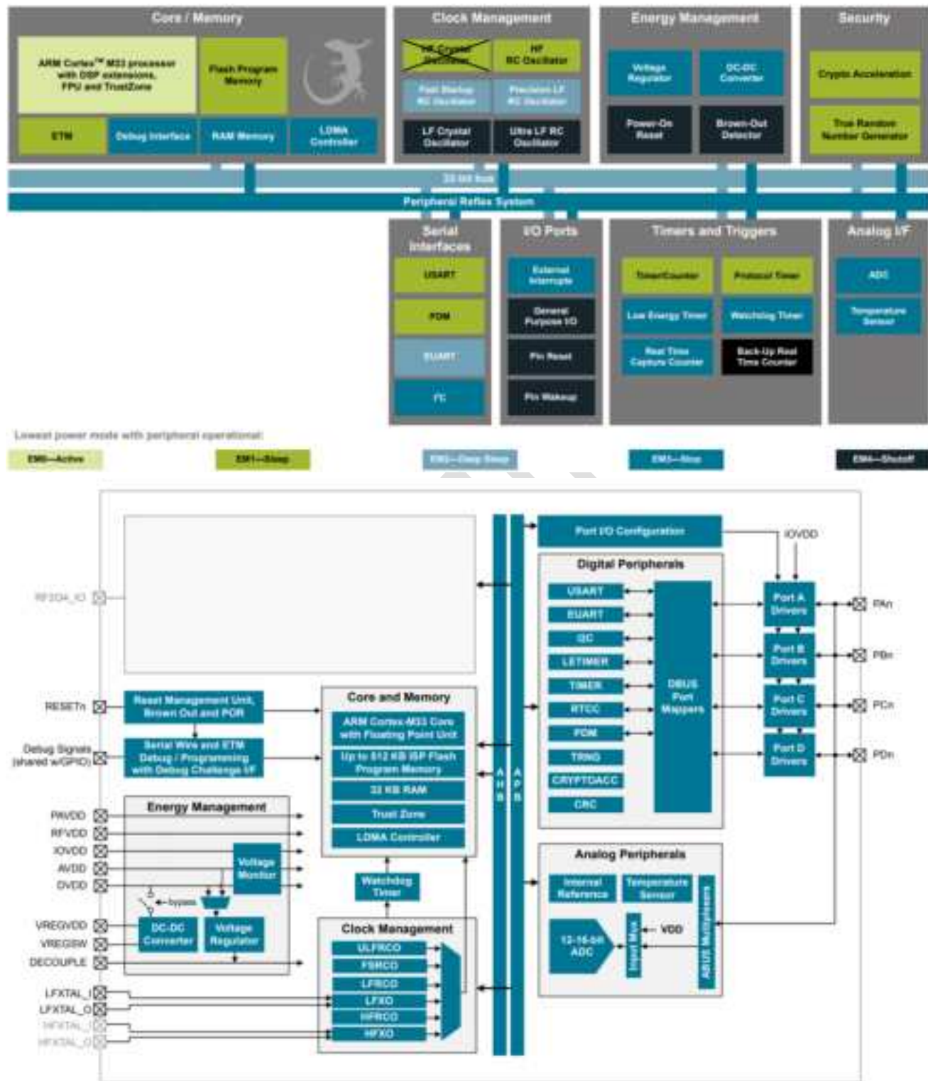
Figure 4: EFR32BG22 microcontroller peripherals and block diagram (from EFR32 datasheet)
