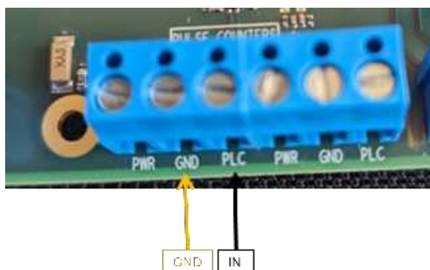
Figure 9 Pulse meter WO power
