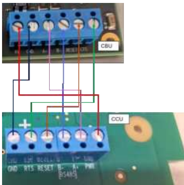
Figure 1 CCU-CBU Wiring diagram
