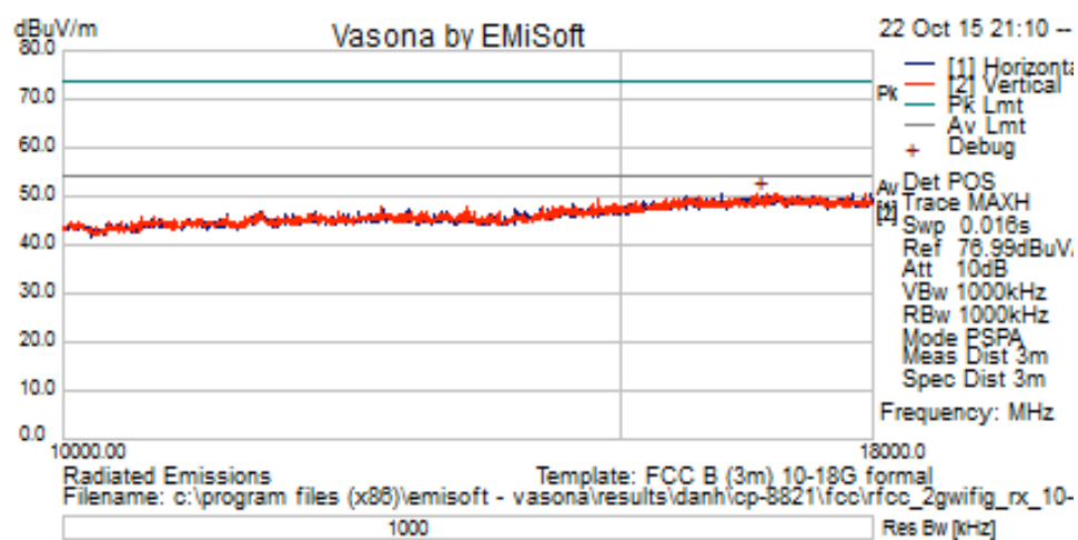
Title: Rx Spurious Emissions from 10-18GHz
