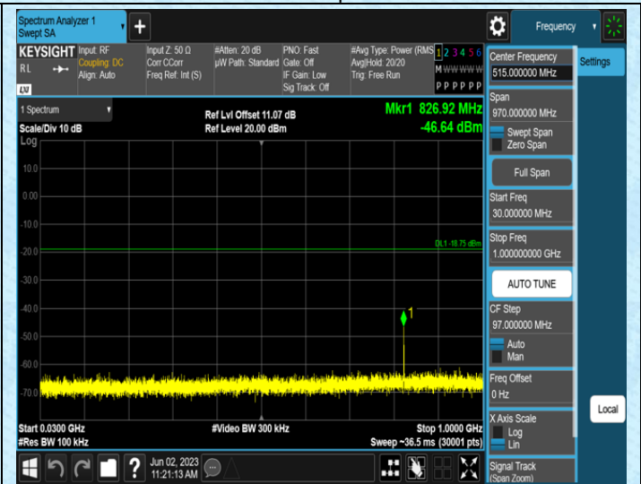
BLE_1M-Ant1-2480-30-1000
