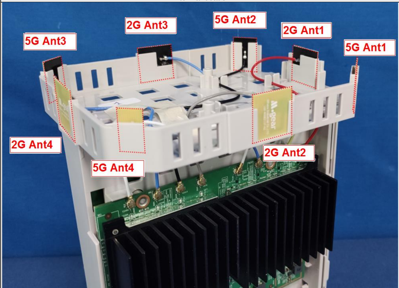
Antenna location
