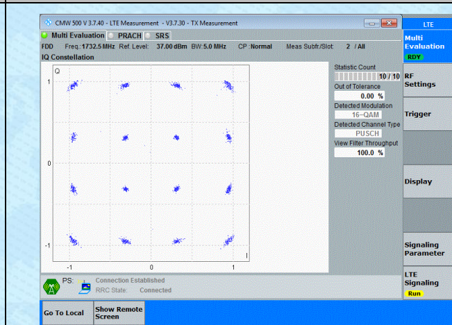
Band4-5MHz-16QAM-20175-25RB#0-PASS
