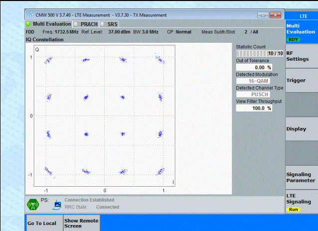
Band4-3MHz-16QAM-20175-15RB#0-PASS
