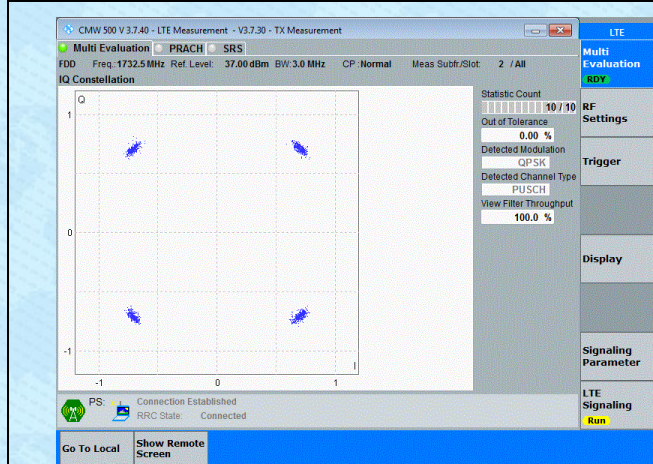
Band4-3MHz-QPSK-20175-15RB#0-PASS
