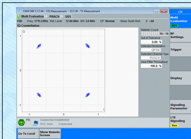
Band4-3MHz-QPSK-19965-15RB#0-PASS
