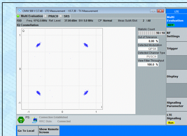
Band4-5MHz-QPSK-19975-25RB#0-PASS
