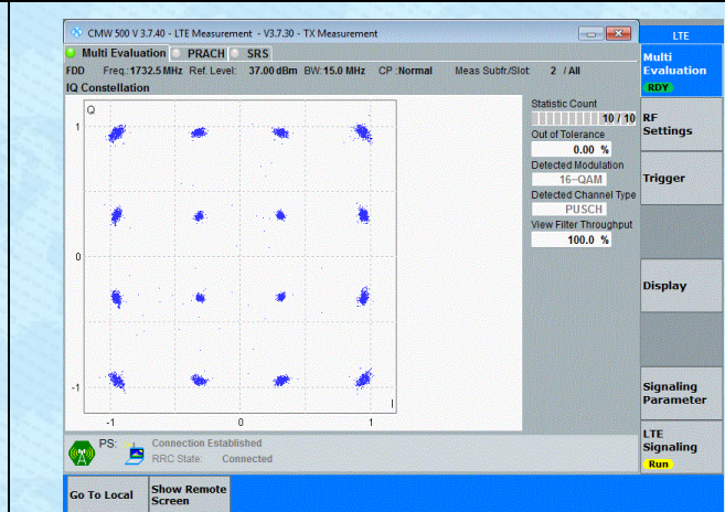
Band4-15MHz-16QAM-20175-75RB#0-PASS
