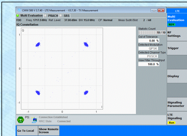
Band4-15MHz-QPSK-20025-75RB#0-PASS
