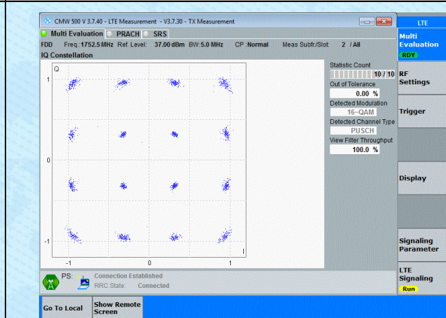
Band4-5MHz-16QAM-20375-25RB#0-PASS
