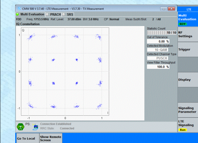
Band4-3MHz-16QAM-20385-15RB#0-PASS
