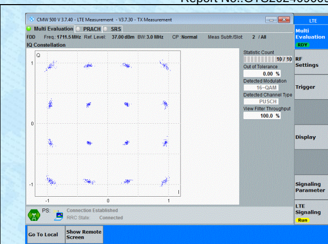
Band4-3MHz-16QAM-19965-15RB#0-PASS
