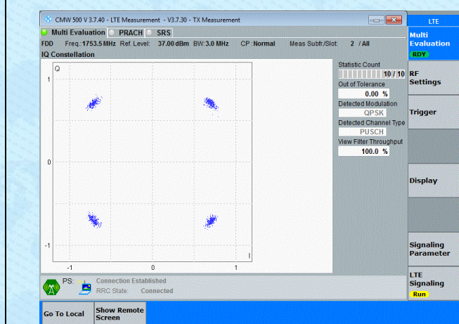
Band4-3MHz-QPSK-20385-15RB#0-PASS
