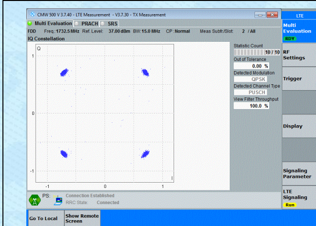
Band4-15MHz-QPSK-20175-75RB#0-PASS
