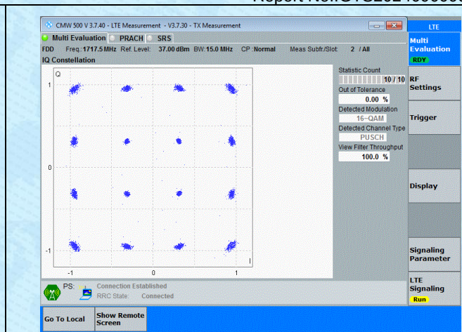
Band4-15MHz-16QAM-20025-75RB#0-PASS
