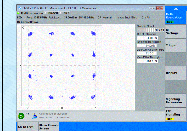
Band4-15MHz-16QAM-20325-75RB#0-PASS
