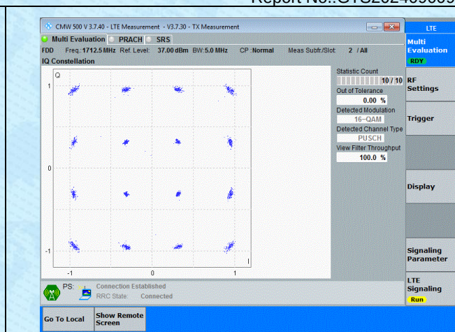
Band4-5MHz-16QAM-19975-25RB#0-PASS
