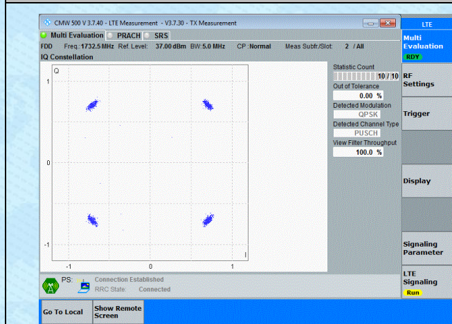
Band4-5MHz-QPSK-20175-25RB#0-PASS
