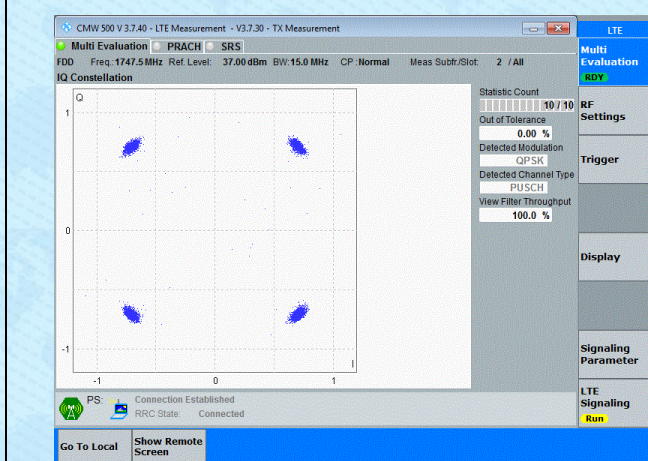
Band4-15MHz-QPSK-20325-75RB#0-PASS
