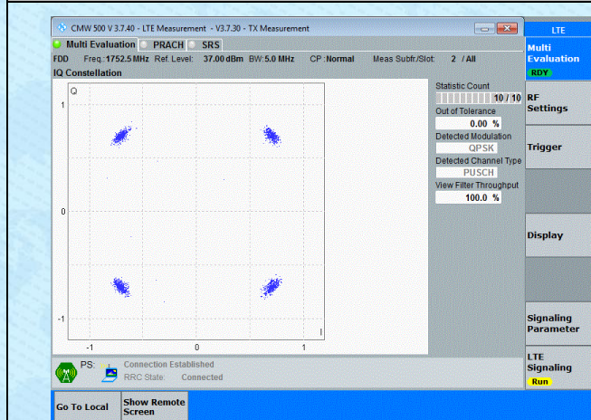
Band4-5MHz-QPSK-20375-25RB#0-PASS
