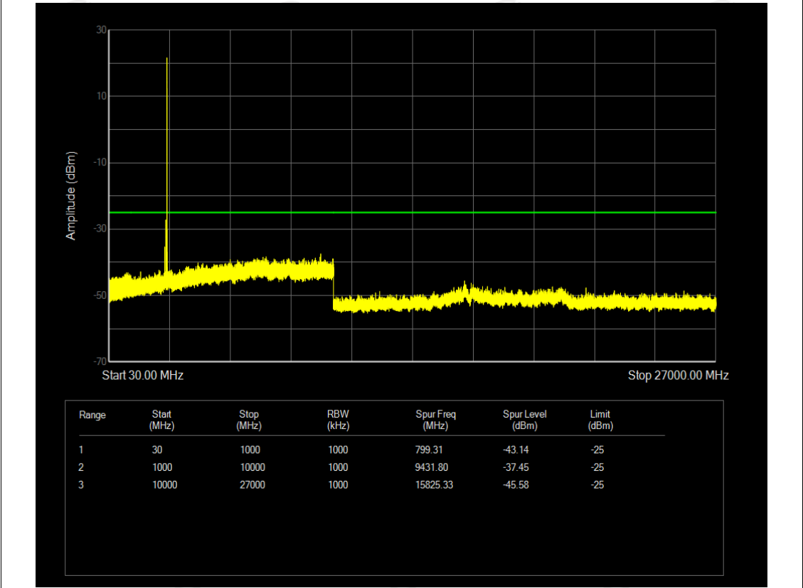
n41 SCS=30kHz DFT_BPSK BW=100MHz Channel=509202 RB=1@272
