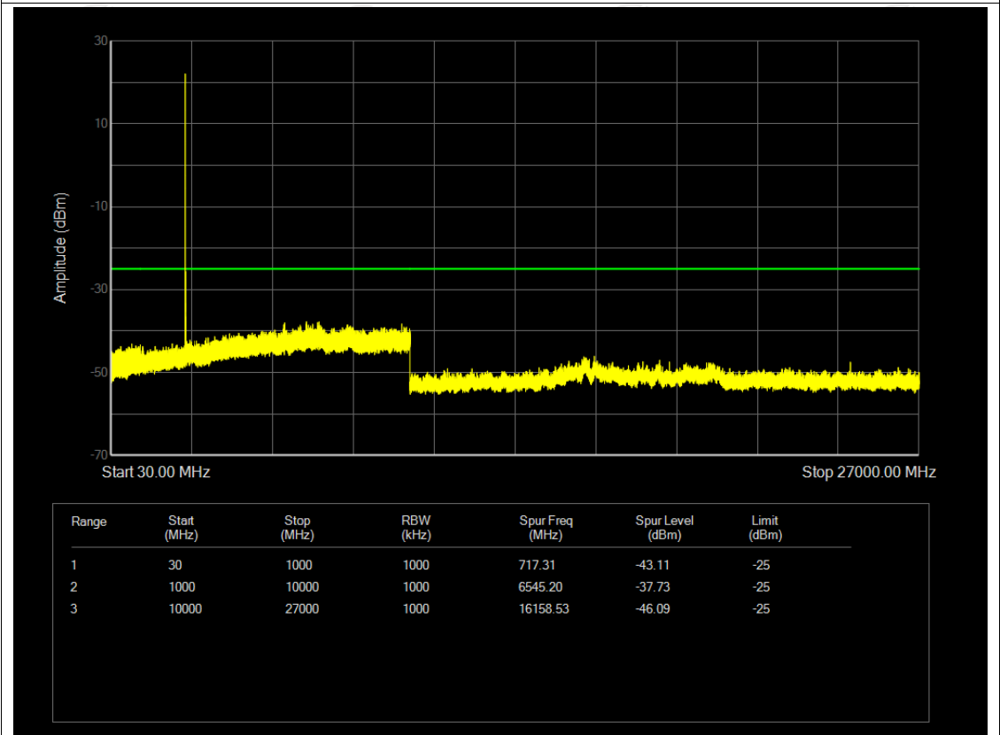
n41 SCS=30kHz DFT_BPSK BW=100MHz Channel=518598 RB=1@0
