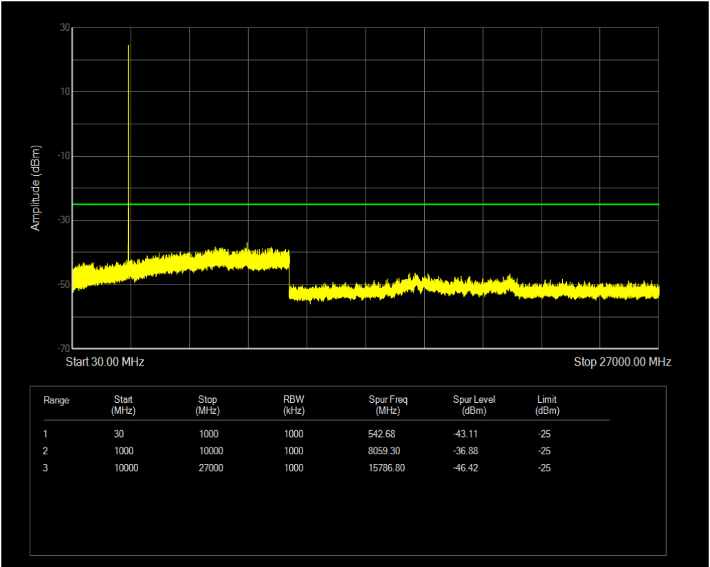
n41 SCS=30kHz DFT_BPSK BW=20MHz Channel=518598 RB=1@50
