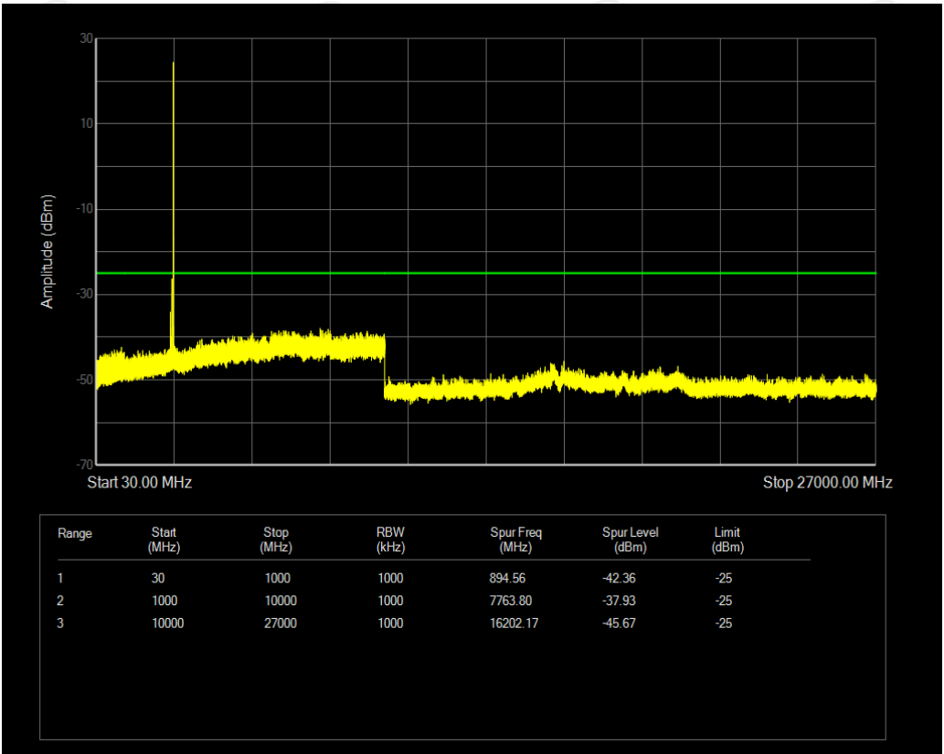
n41 SCS=30kHz DFT_BPSK BW=100MHz Channel=528000 RB=1@272
