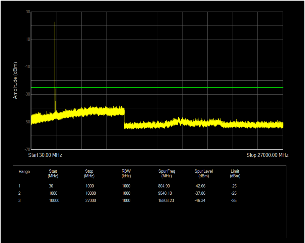
n41 SCS=30kHz DFT_BPSK BW=60MHz Channel=518598 RB=1@0
