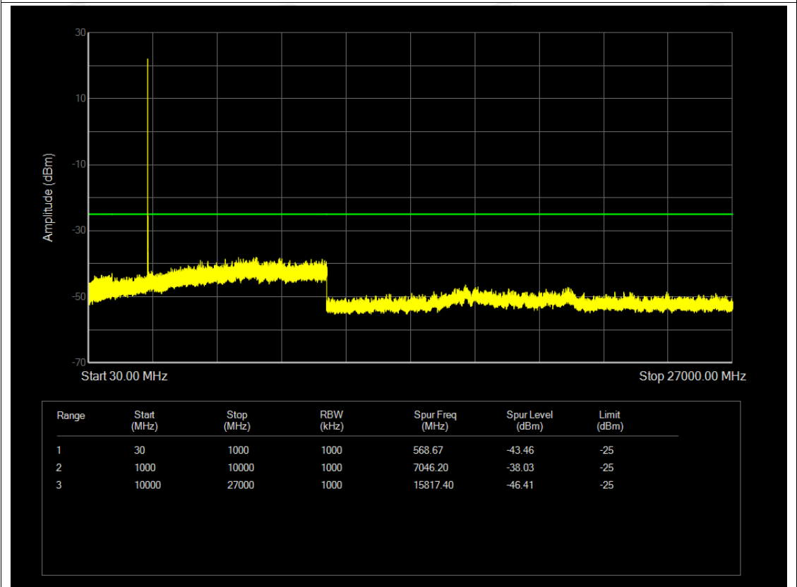
n41 SCS=30kHz DFT_BPSK BW=20MHz Channel=501204 RB=1@50
