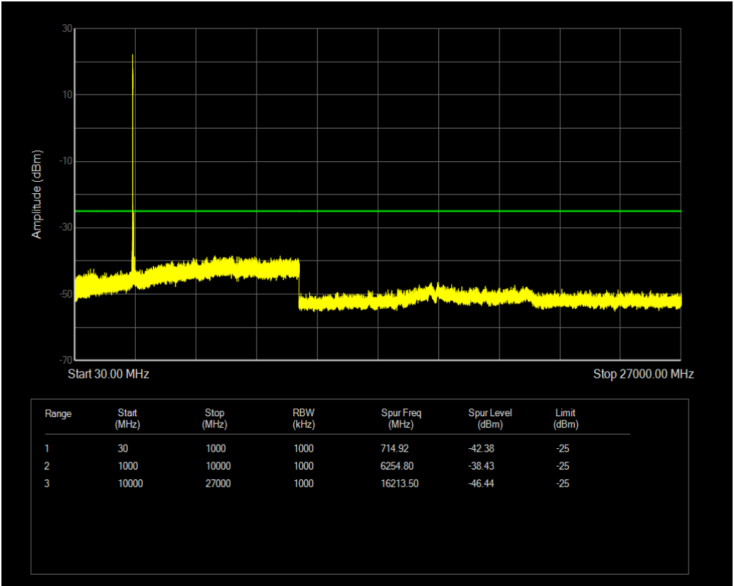
n41 SCS=30kHz DFT_BPSK BW=100MHz Channel=528000 RB=1@0
