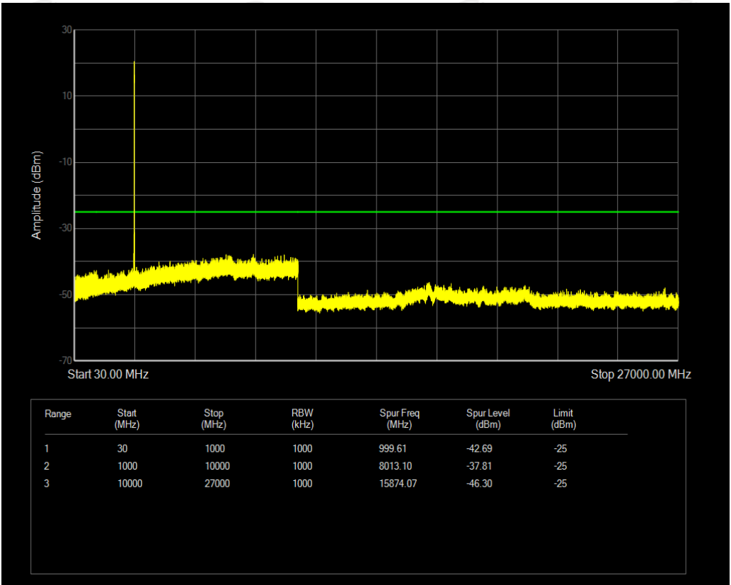
n41 SCS=30kHz DFT_BPSK BW=20MHz Channel=535998 RB=1@50
