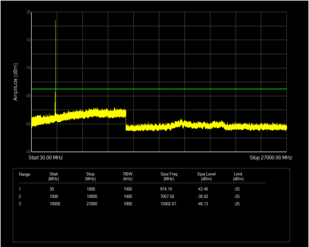
n41 SCS=30kHz DFT_BPSK BW=60MHz Channel=505200 RB=1@161
