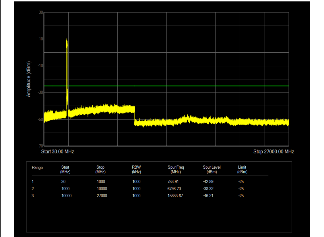
n41 SCS=30kHz DFT_BPSK BW=100MHz Channel=509202 RB=270@0
