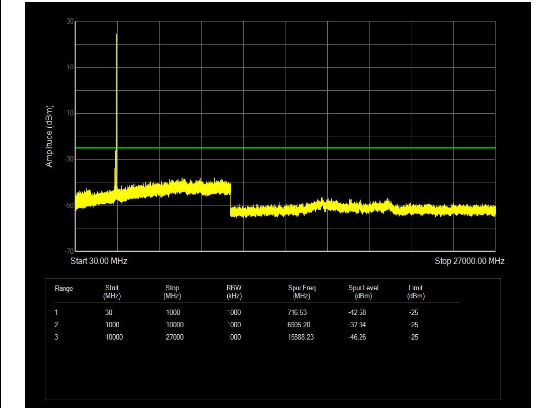
n41 SCS=30kHz DFT_BPSK BW=100MHz Channel=518598 RB=1@272
