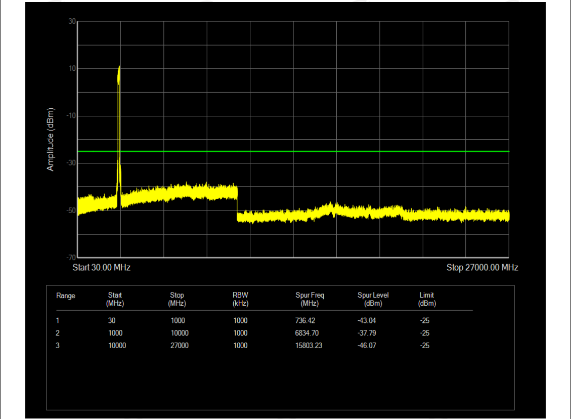
n41 SCS=30kHz DFT_BPSK BW=100MHz Channel=518598 RB=270@0
