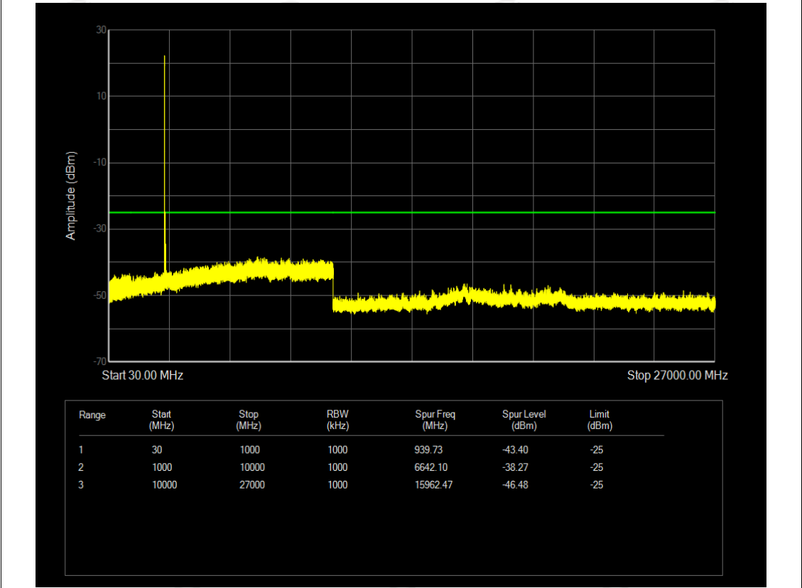
n41 SCS=30kHz DFT_BPSK BW=60MHz Channel=505200 RB=1@0
