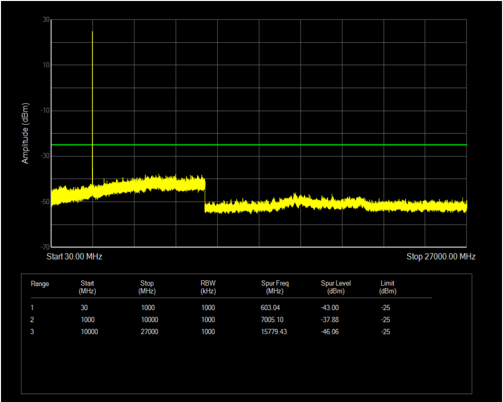
n41 SCS=30kHz DFT_BPSK BW=60MHz Channel=531996 RB=1@161
