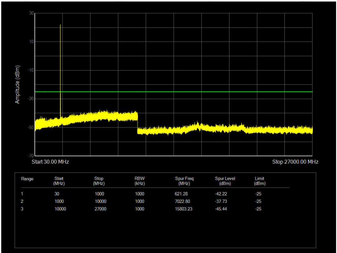
n41 SCS=30kHz DFT_BPSK BW=60MHz Channel=531996 RB=1@0
