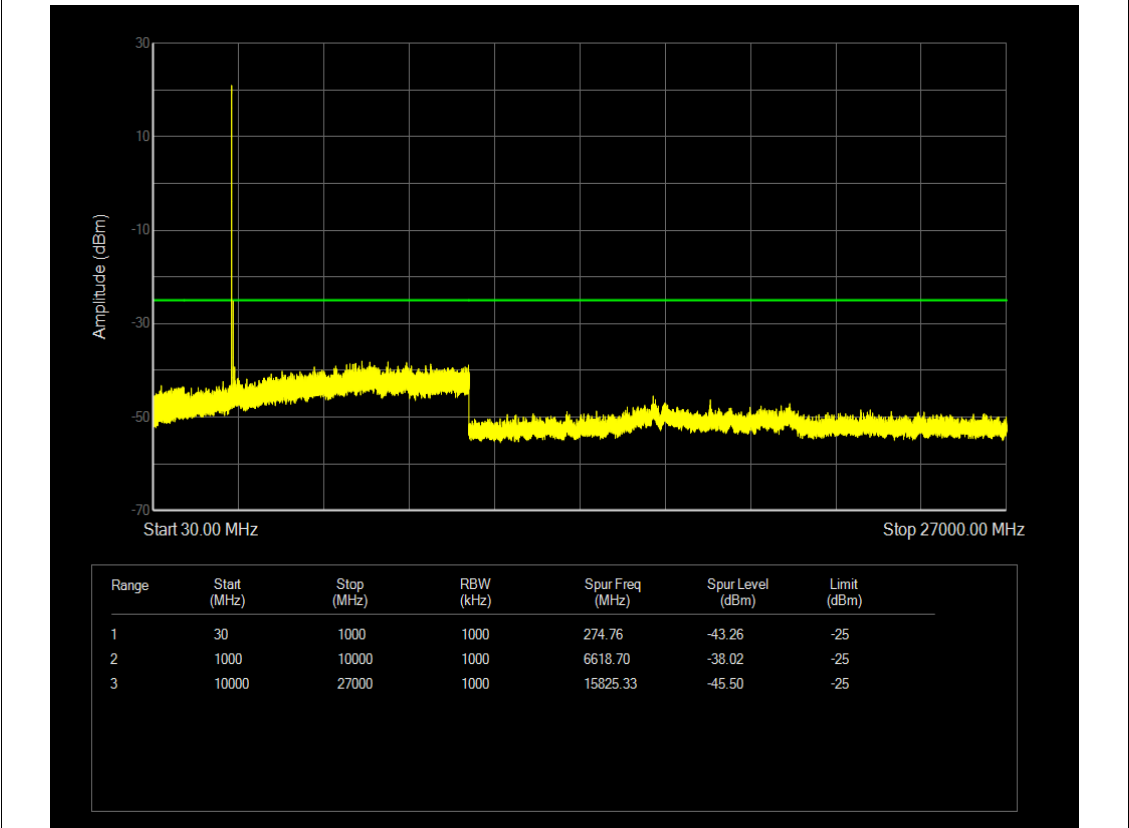
n41 SCS=30kHz DFT_BPSK BW=100MHz Channel=509202 RB=1@0
