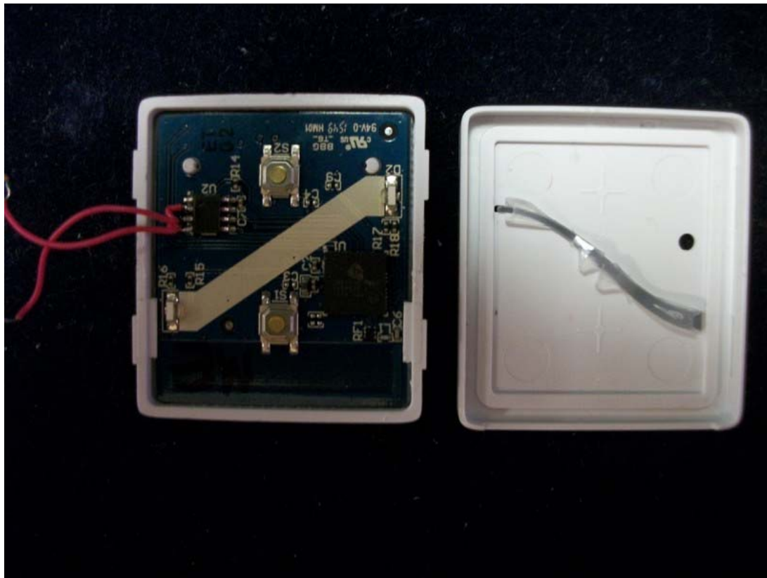
7.3 Inside View
