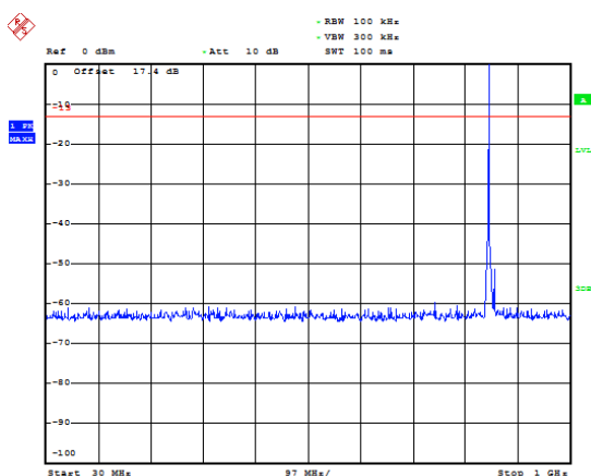
NB-IOT Band 5 CH-High 30MHz-1GHz
