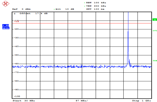
NB-IOT Band 5 CH-Middle 30MHz-1GHz
