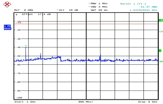
NB-IOT Band 5 CH-Low 1GHz-9GHz
