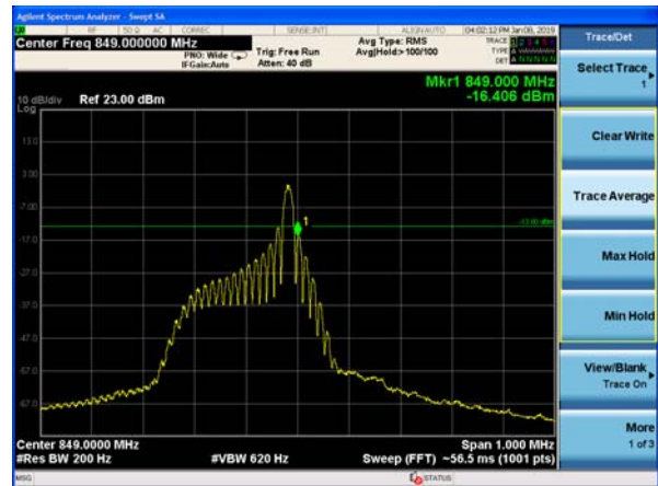
NB-IOT Band 5 QPSK 15kHz 12@0 CH-High
