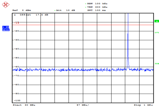
NB-IOT Band 5 CH-Low 30MHz-1GHz
