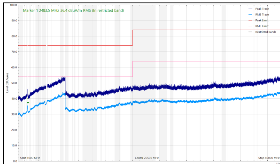
Figure 51 - 2442 MHz (CH7), HT20, Core 1 and 5204 MHz, DH5, ePA, Core 0, 1 GHz to 40 GHz, Horizontal
