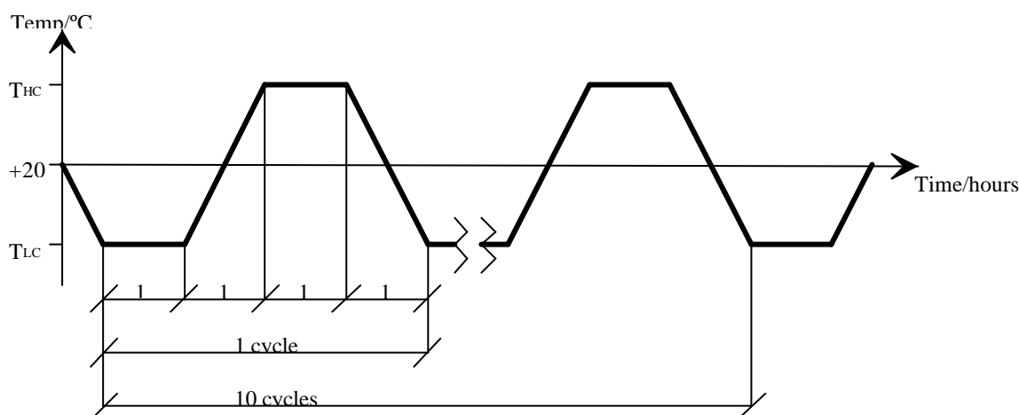
Figure 4-1: Temperature Cycling
