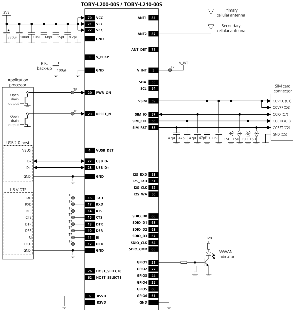
Figure 73: Example of schematic diagram to integrate a TOBY-L200-00S or TOBY-L210-00S in an application, using all interfaces
