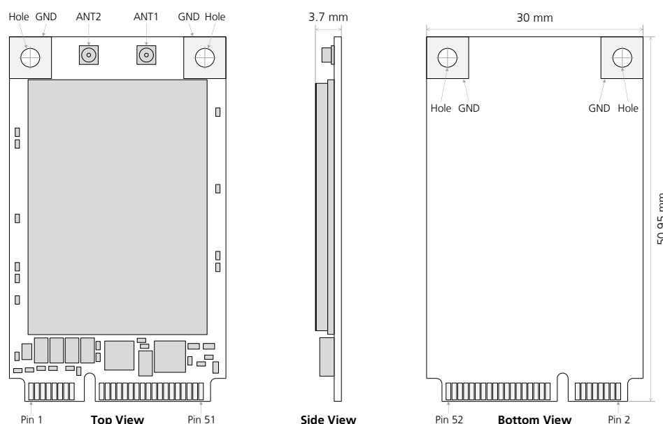
Figure 70: MPCPI-L2 series mechanical description (top, side and bottom views)
