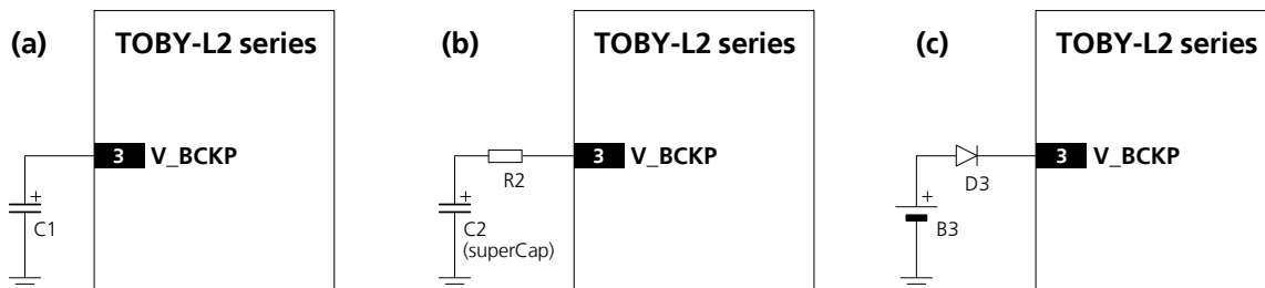
Figure 41: Real time clock supply (V_BCKP) application circuits: (a) using a 100 μF capacitor to let the RTC run for ~80 s after VCC removal; (b) using a 70 mF capacitor to let RTC run for ~15 hours after VCC removal; (c) using a non-rechargeable battery
