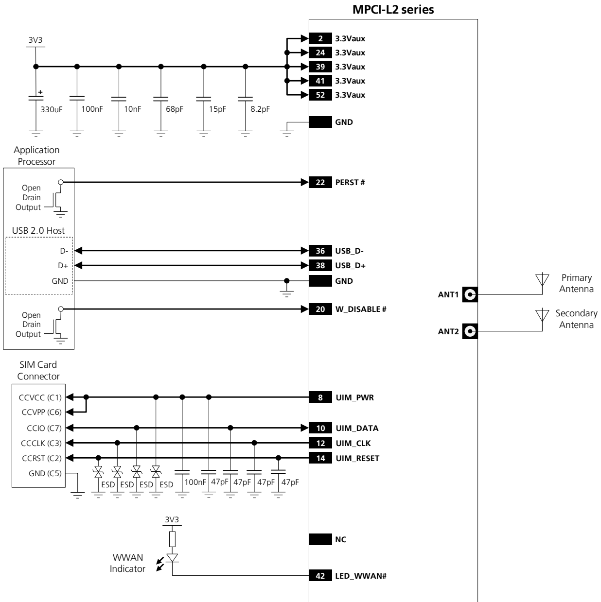
Figure 76: Example of schematic diagram to integrate a MPC-I-L2 series module in an application board, using all the interfaces
