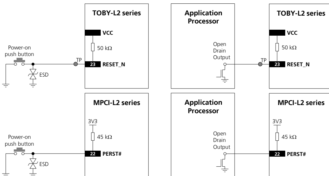
Figure 43: RESET_N and PERST# application circuits using a push button and an open drain output of an application processor
