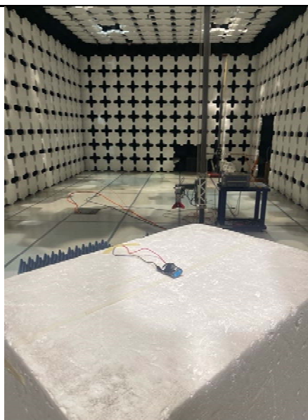
Radiated Emission Test Above 1GHz Rear View
