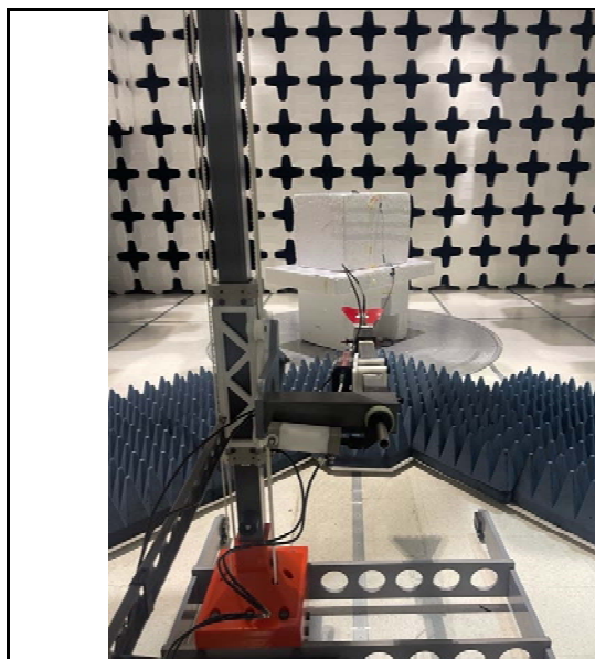
Radiated Emission Test Above 1GHz Front View
