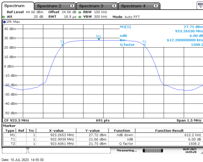
Figure 7.5-1: 6 dB bandwidth on low channel
