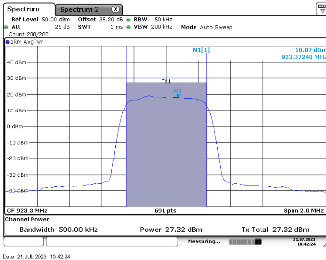
Figure 7.6-1: Output power on low channel
