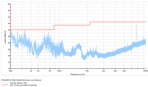
Figure 7.7-6: Radiated spurious emissions on low channel [30-850 MHz]
