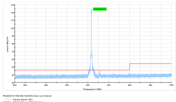
Figure 7.7-7: Radiated spurious emissions on low channel [850-1000 MHz]
