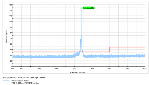
Figure 7.7-9: Radiated spurious emissions on high channel [850-1000 MHz]
