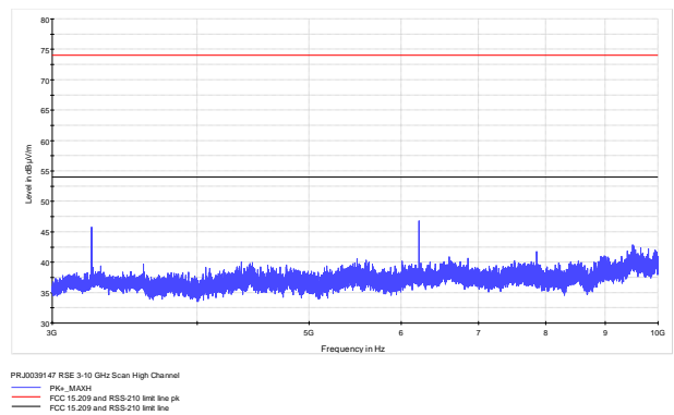
Figure 7.7-13: Radiated spurious emissions on high channel [3-10 GHz]
