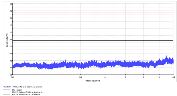
Figure 7.7-11: Radiated spurious emissions on low channel [3-10 GHz]
