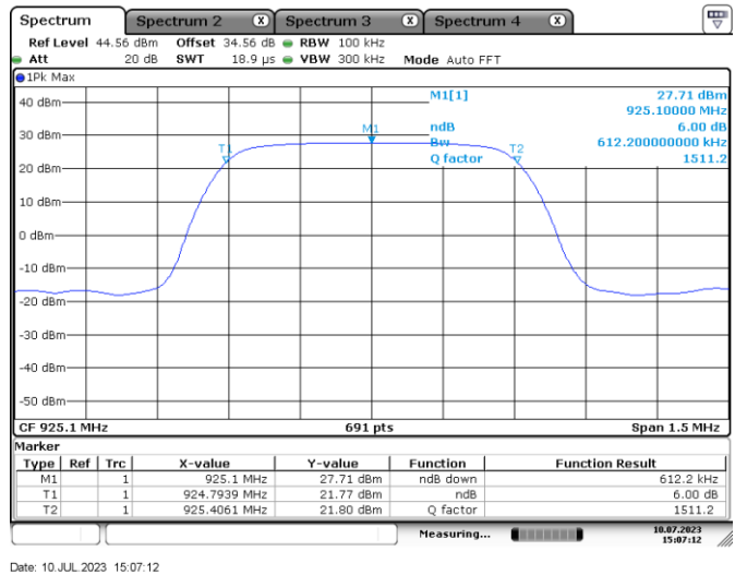
Figure 7.5-2: 6 dB bandwidth on mid channel
