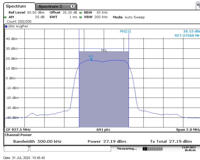
Figure 7.6-3: Output power on high channel
