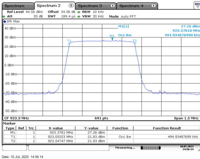
Figure 7.5-4: 99% occupied bandwidth on low channel
