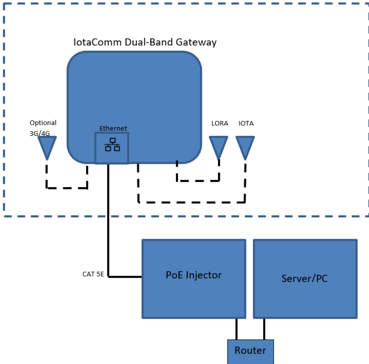
Figure 4.5-1: Block diagram
