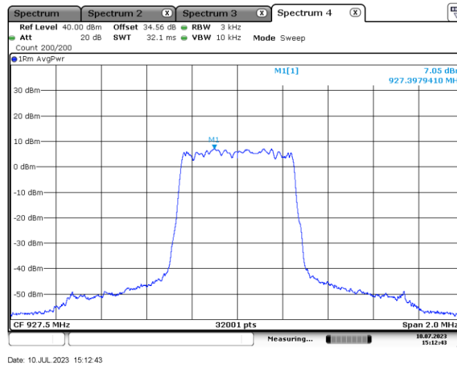
Figure 7.8-3: PSD on high channel
