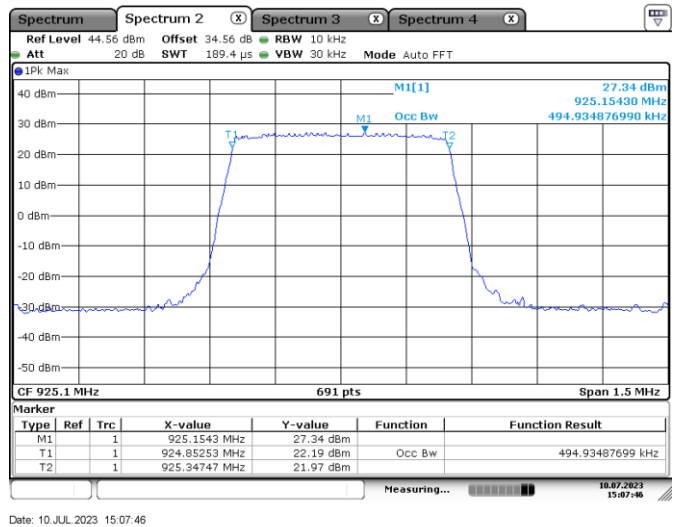
Figure 7.5-5: 99% occupied bandwidth on mid channel
