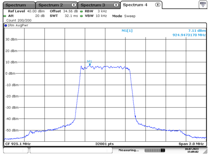
Figure 7.8-2: PSD on mid channel
