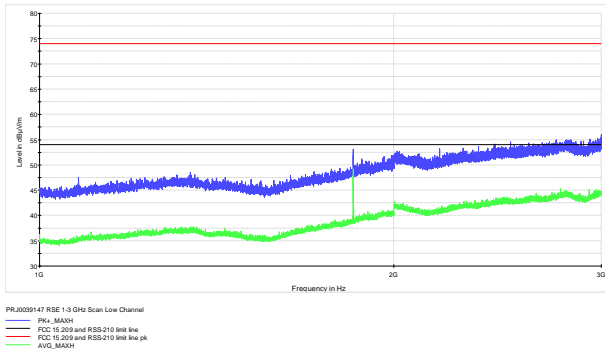
Figure 7.7-10: Radiated spurious emissions on low channel [1-3 GHz]
