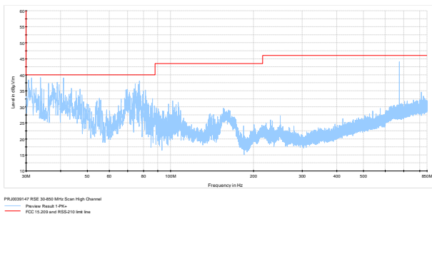
Figure 7.7-8: Radiated spurious emissions on high channel [30-850 MHz]
