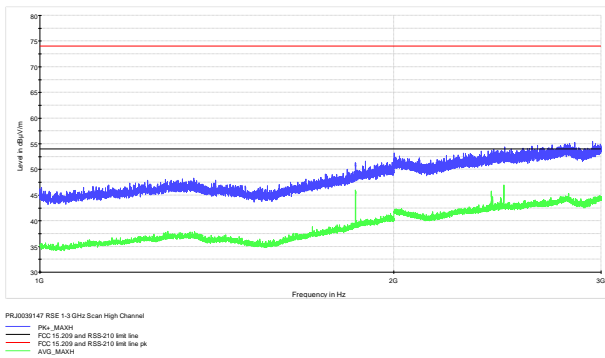
Figure 7.7-12: Radiated spurious emissions on high channel [1-3 GHz]
