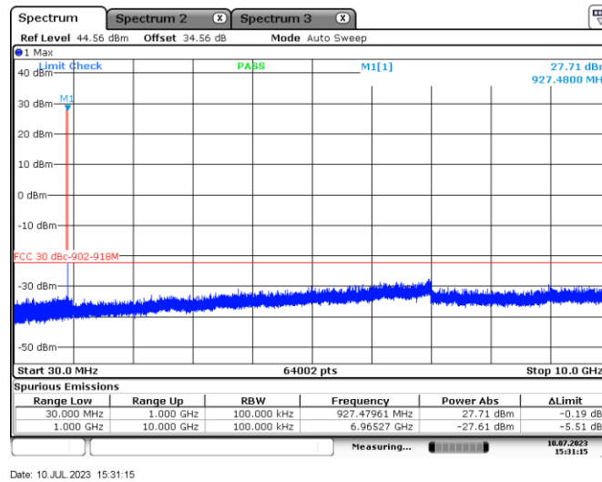
Figure 7.7-5: Conducted spurious emissions on high channel
