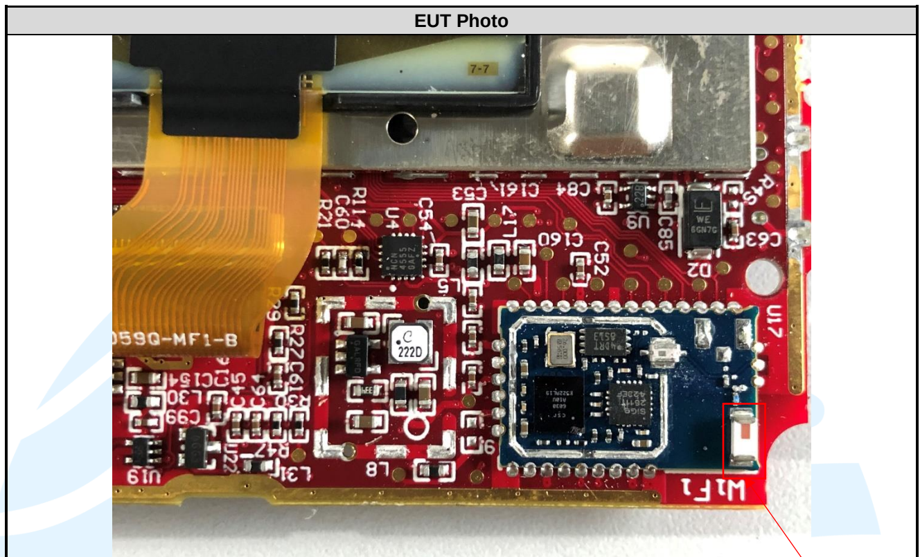
WIFI Antenna
