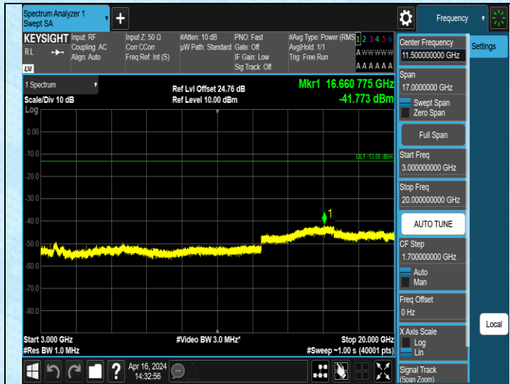
Band4_3MHz_QPSK_20175_1RB#0_3000~20000_3000~20000
