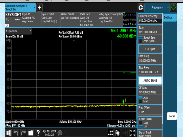
Band4_3MHz_QPSK_20385_1RB#0_30~1000_30~1000
