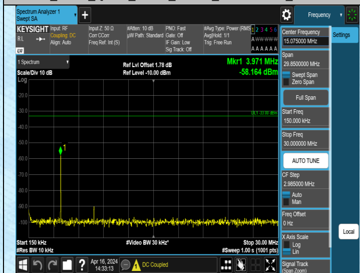
Band4_3MHz_QPSK_20385_1RB#0_0.15~30_0.15~30
