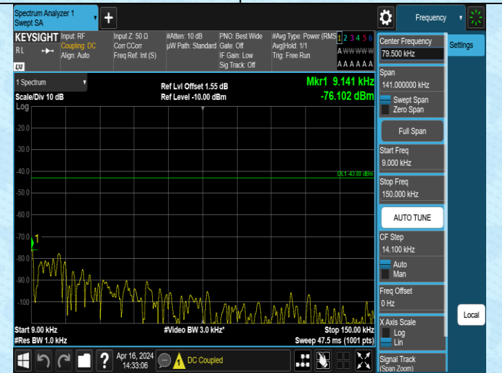
Band4_3MHz_QPSK_20385_1RB#0_0.009~0.15_0.009~0.15
