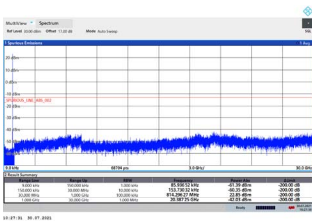
LTE Band 26 1.4MHz CH Middle 9kHz~30GHz
