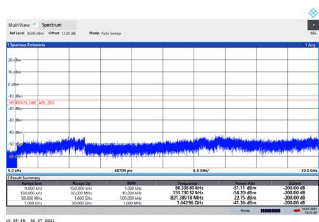
LTE Band 26 3MHz CH High 9kHz~30GHz
