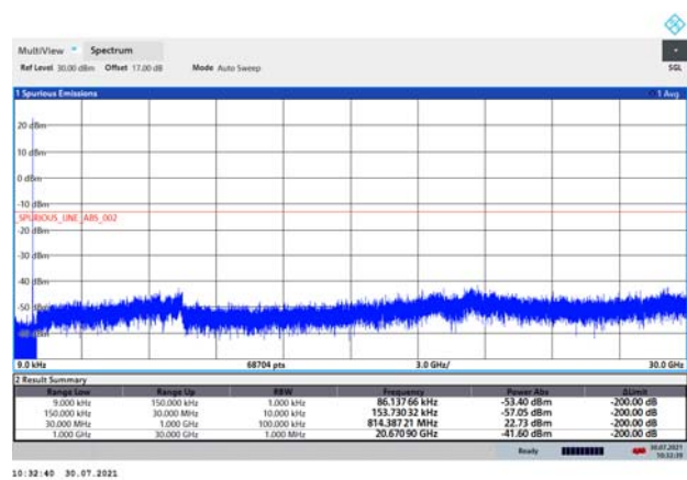
LTE Band 26 3MHz CH Middle 9kHz~30GHz
