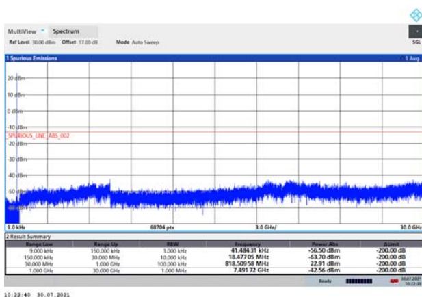
LTE Band 26 1.4MHz CH High 9kHz~30GHz
