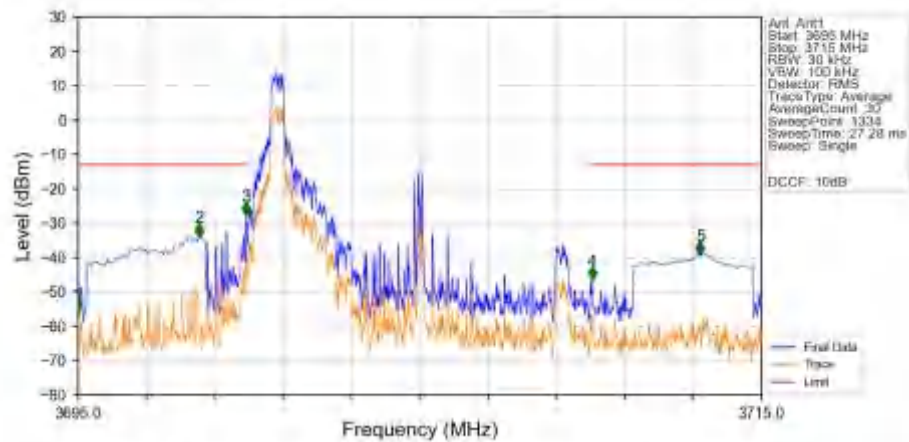
n78a_30kHz_SISO_NTNV_10MHz_CP-OFDM_QPSK_3705MHz_Edge_1RB_Left_Ant1
