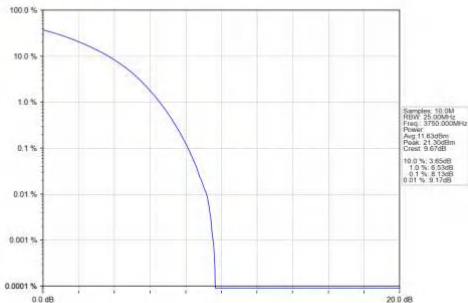
n78a_30kHz_SISO_NTNV_100MHz_CP-OFDM 256 QAM_3750MHz_Outer_Full_Ant1
