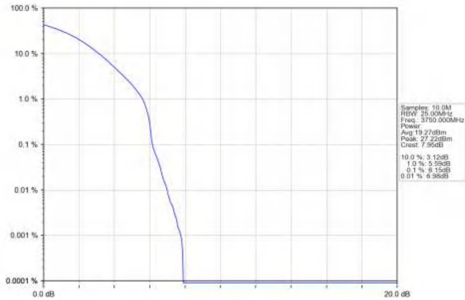
n78a_30kHz_SISO_NTNV_20MHz_DFT-s-OFDM_256_QAM_3750MHz_Outer_Full_Ant1
