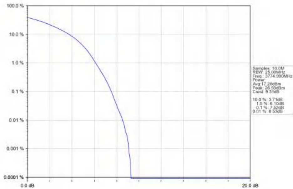
n78a_30kHz_SISO_NTNV_50MHz_DFT-s-OFDM_16_QAM_3774.99MHz_Outer_Full_Ant1
