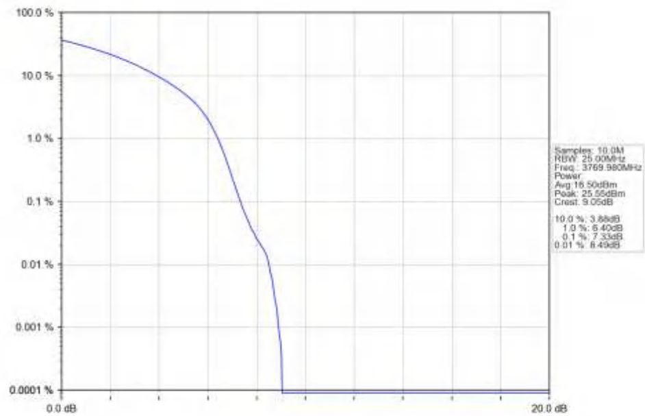
n78a_30kHz_SISO_NTNV_60MHz_DFT-s-OFDM_16_QAM_3769.98MHz_Outer_Full_Ant1
