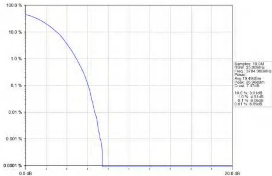
n78a_30kHz_SISO_NTNV_30MHz_DFT-s-OFDM_16_QAM_3784.98MHz_Outer_Full_Ant1
