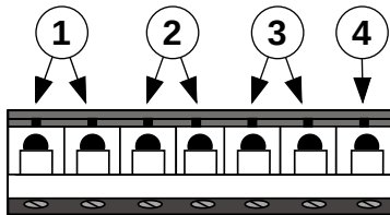
Figure 5: DS840LSN Terminals
