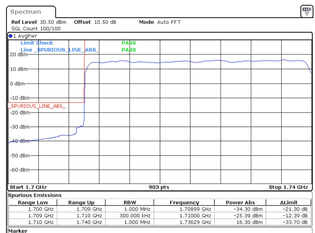
30MHz_15kHz_1725MHz_DFT-s-OFDM QPSK_RB160@0&amp;-25.39 dBm
