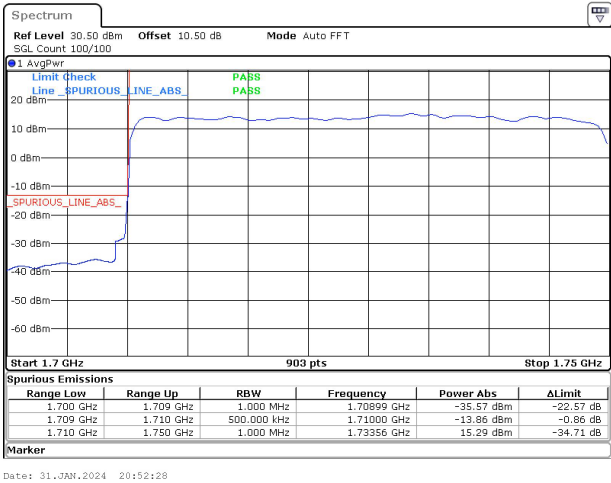
40MHz_15kHz_1730MHz_DFT-s-OFDM QPSK_RB216@0&-13.86 dBm
