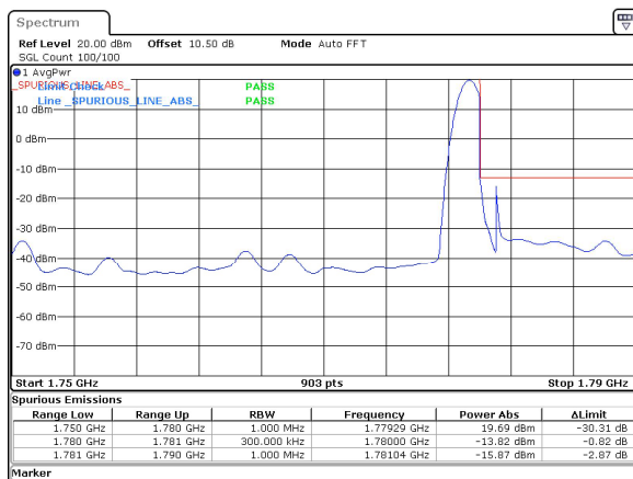
30MHz_15kHz_1765MHz_DFT-s-OFDM QPSK_RB1@159&amp;-13.82 dBm
