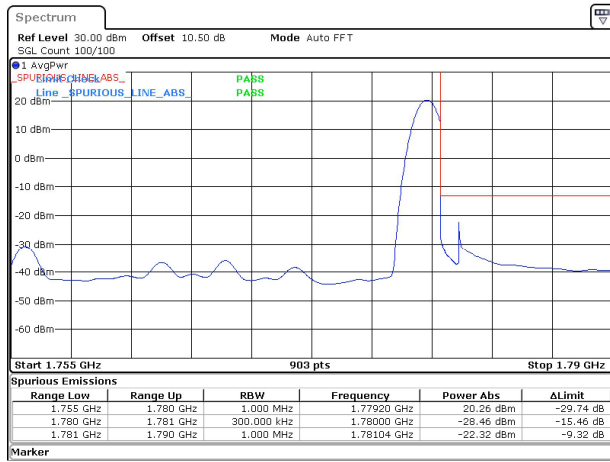
25MHz_15kHz_1767.5MHz_DFT-s-OFDM QPSK_RB1@132&amp;-22.32 dBm
