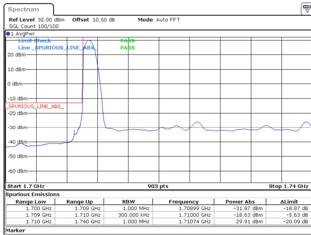
30MHz_15kHz_1725MHz_DFT-s-OFDM QPSK_RB1@0&amp;-18.63 dBm
