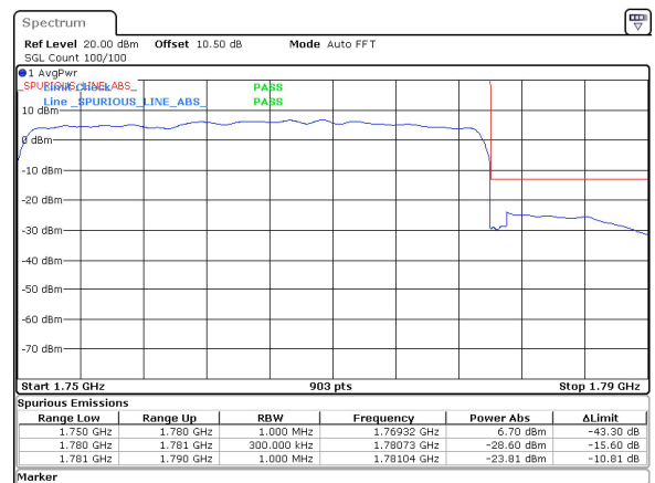
30MHz_15kHz_1765MHz_DFT-s-OFDM QPSK_RB160@0&amp;-23.81 dBm
