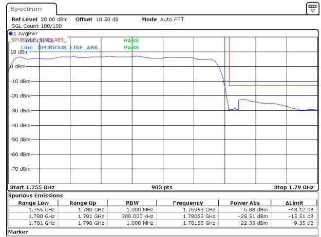
25MHz_15kHz_1767.5MHz_DFT-s-OFDM QPSK_RB128@0&amp;-22.35 dBm
