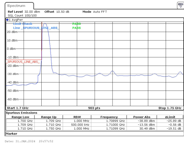
40MHz_15kHz_1730MHz_DFT-s-OFDM QPSK_RB1@0&-13.56 dBm
