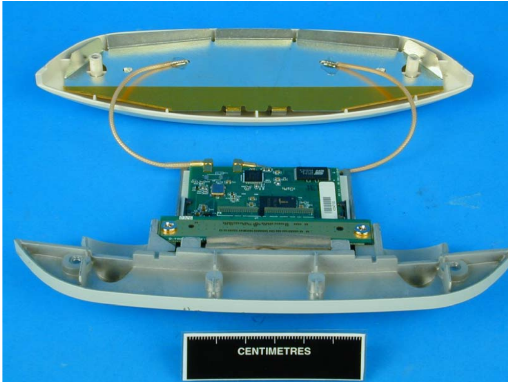
Internal of Integral Antenna
