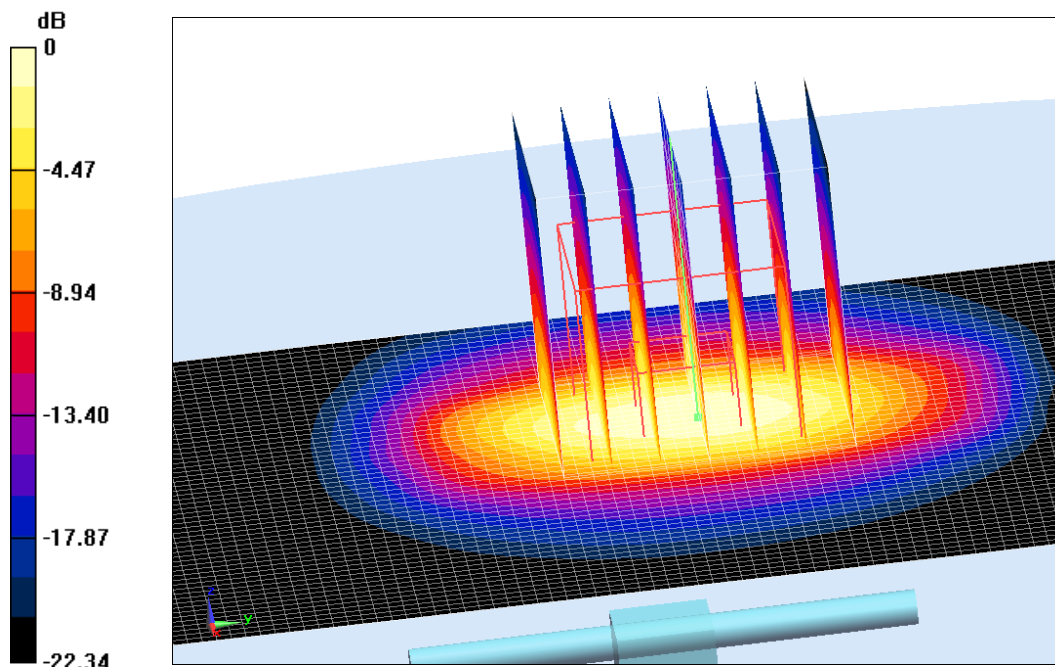
Fig.B.2 validation 2450 MHz 250mW
