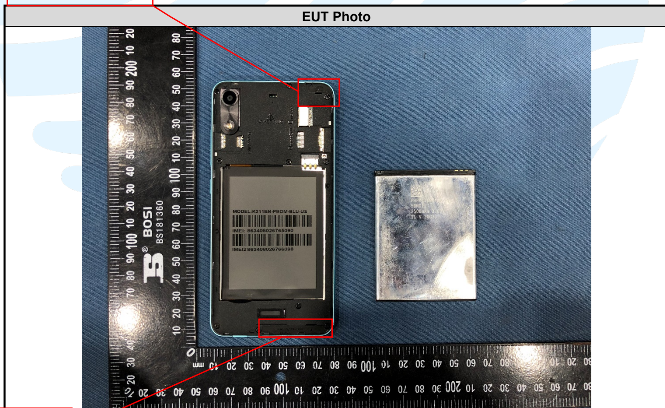
2G/3G Antenna
