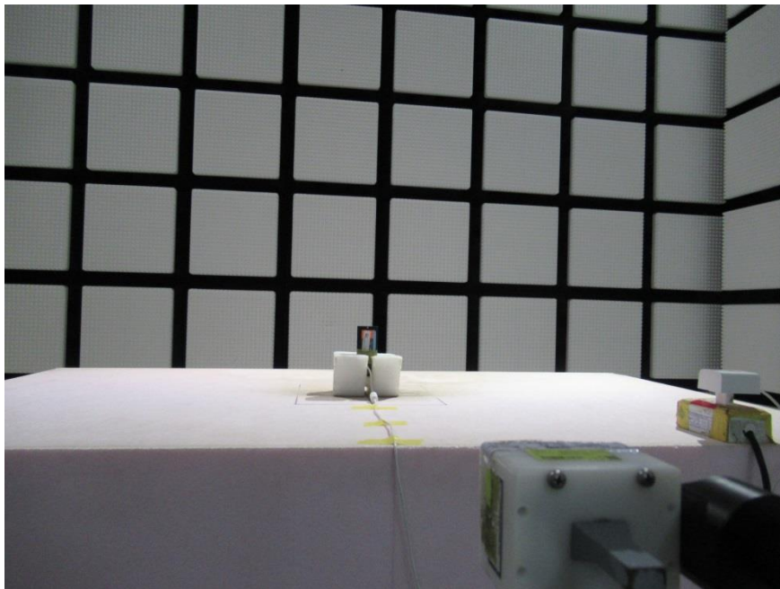
40GHz~60GHz
