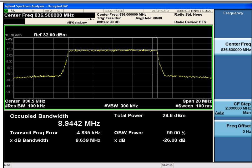
Band5-10MHz-16QAM-20525-50RB#0-8.9442
