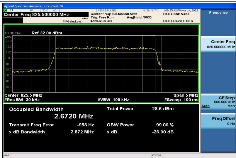
Band5-3MHz-16QAM-20415-15RB#0-2.6720
