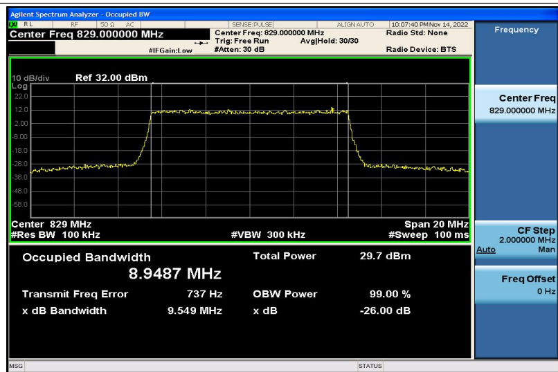
Band5-10MHz-16QAM-20450-50RB#0-8.9487
