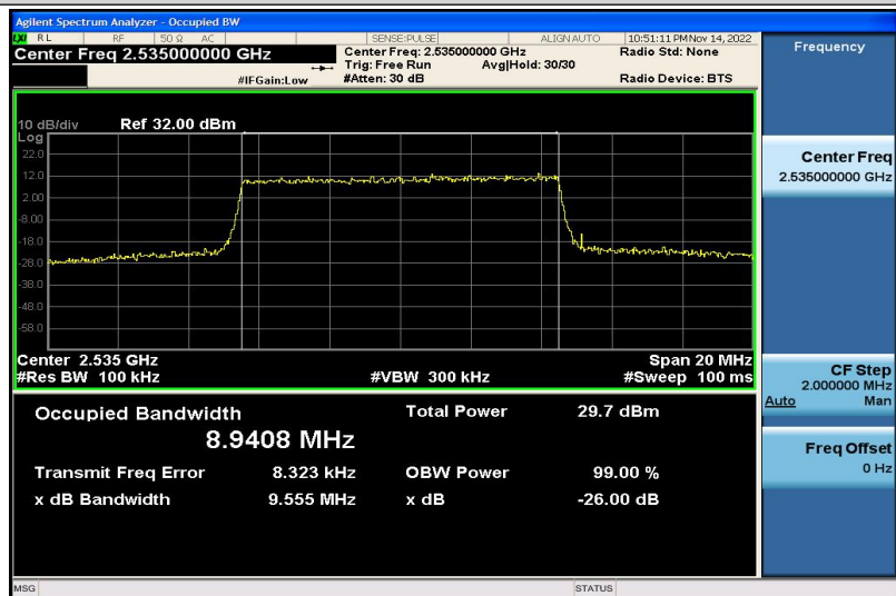
Band7-10MHz-QPSK-21100-50RB#0-8.9408
