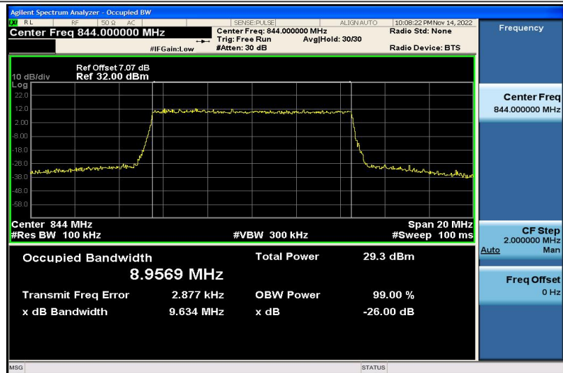
Band5-10MHz-16QAM-20600-50RB#0-8.9569
