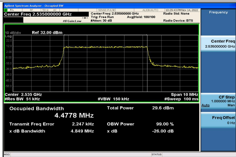
Band7-5MHz-QPSK-21100-25RB#0-4.4778
