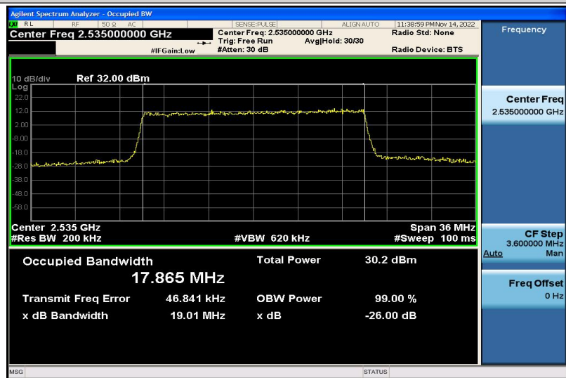
Band7-20MHz-QPSK-21100-100RB#0-17.865
