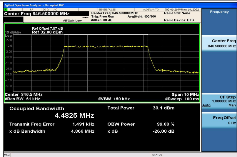
Band5-5MHz-QPSK-20625-25RB#0-4.4825
