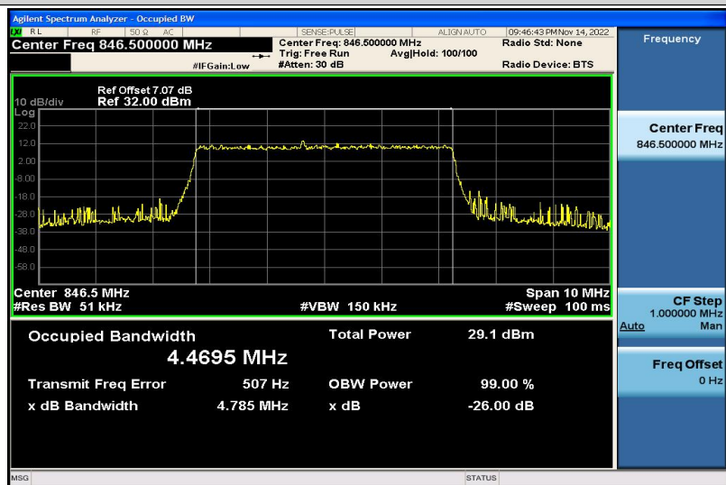
Band5-5MHz-16QAM-20625-25RB#0-4.4695
