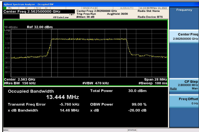
Band7-15MHz-QPSK-21375-75RB#0-13.444
