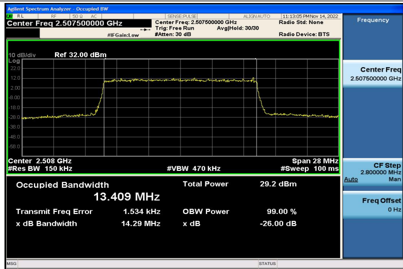
Band7-15MHz-16QAM-20825-75RB#0-13.409
