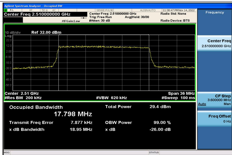
Band7-20MHz-16QAM-20850-100RB#0-17.798
