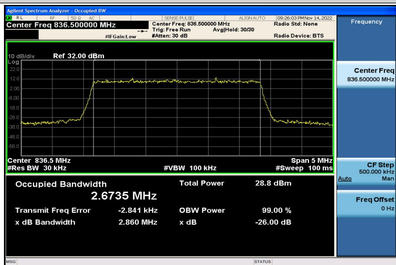
Band5-3MHz-16QAM-20525-15RB#0-2.6735
