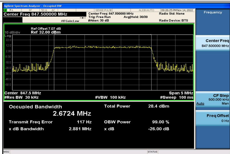
Band5-3MHz-16QAM-20635-15RB#0-2.6724
