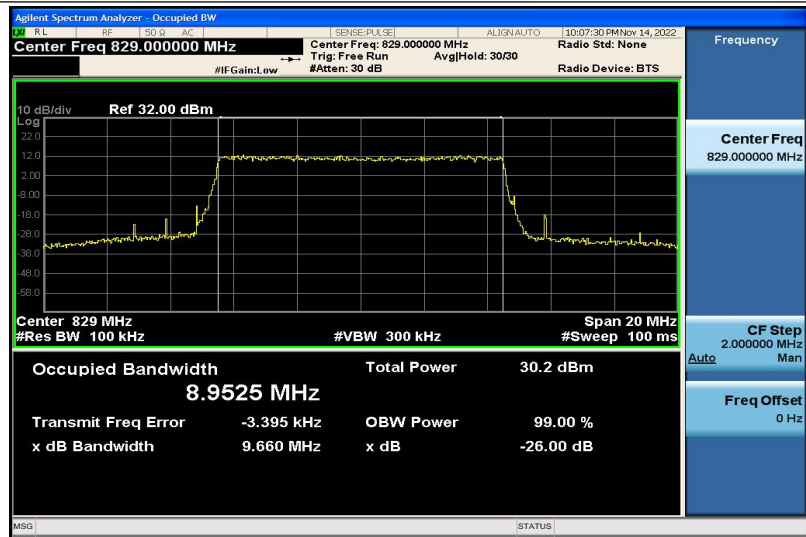
Band5-10MHz-QPSK-20450-50RB#0-8.9525
