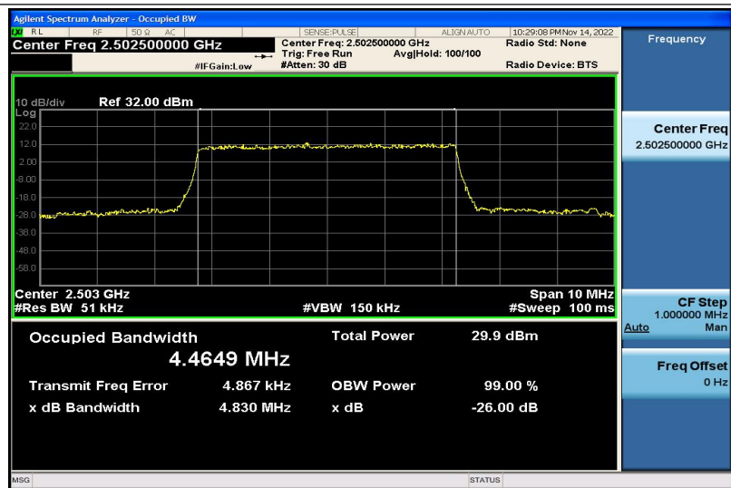
Band7-5MHz-QPSK-20775-25RB#0-4.4649
