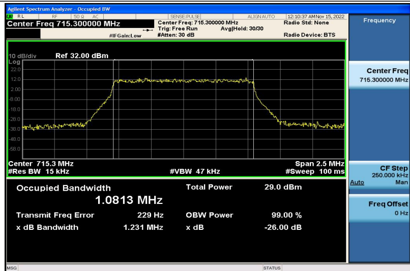
Band12-1.4MHz-QPSK-23173-6RB#0-1.0813
