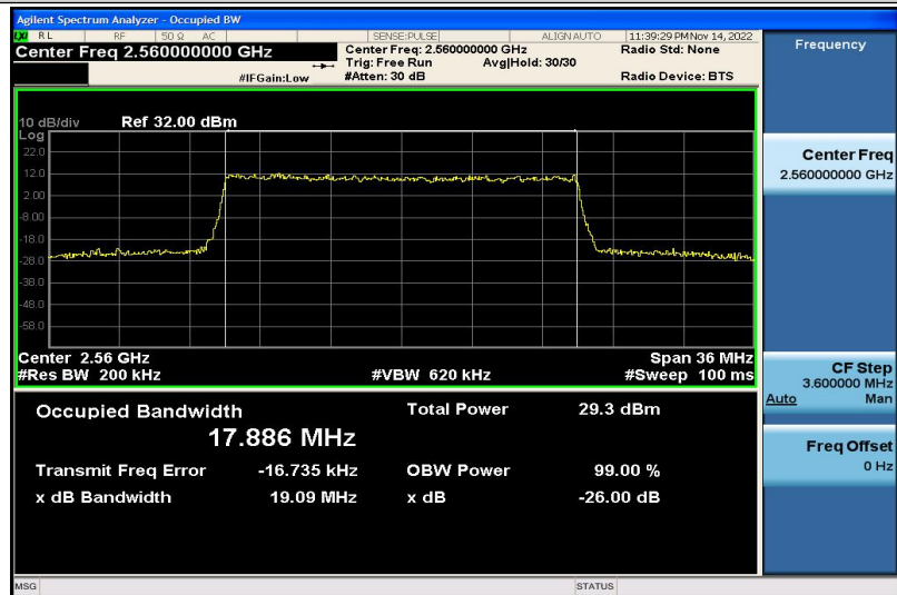
Band7-20MHz-16QAM-21350-100RB#0-17.886
