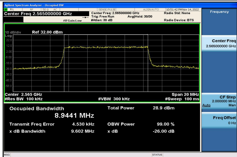
Band7-10MHz-16QAM-21400-50RB#0-8.9441
