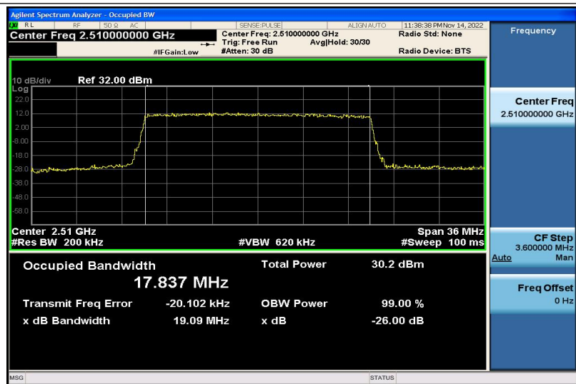
Band7-20MHz-QPSK-20850-100RB#0-17.837
