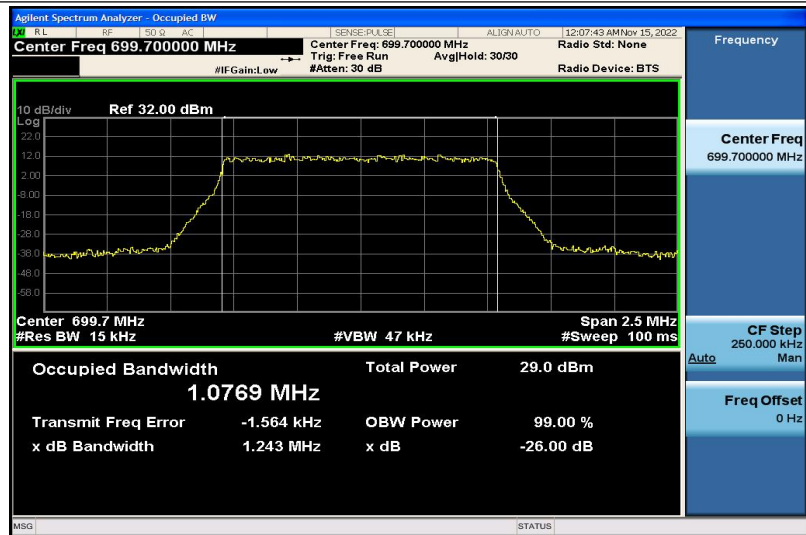
Band12-1.4MHz-QPSK-23017-6RB#0-1.0769
