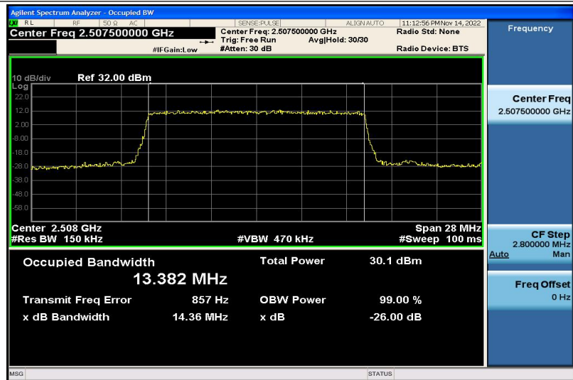
Band7-15MHz-QPSK-20825-75RB#0-13.382
