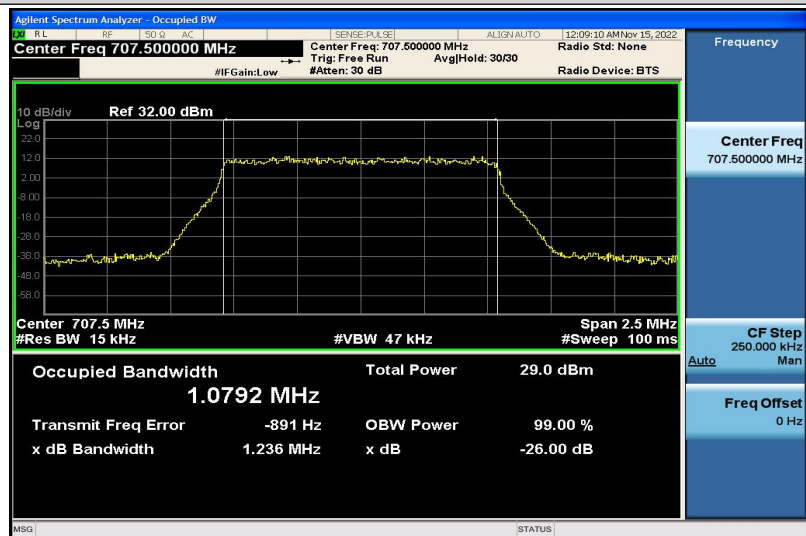
Band12-1.4MHz-QPSK-23095-6RB#0-1.0792
