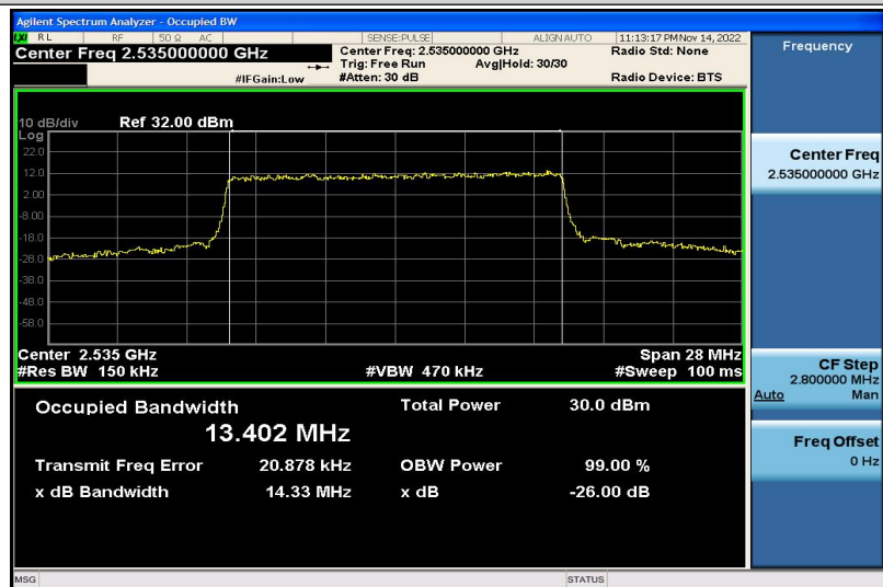
Band7-15MHz-QPSK-21100-75RB#0-13.402
