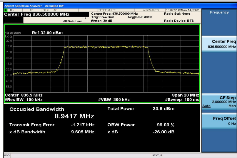
Band5-10MHz-QPSK-20525-50RB#0-8.9417
