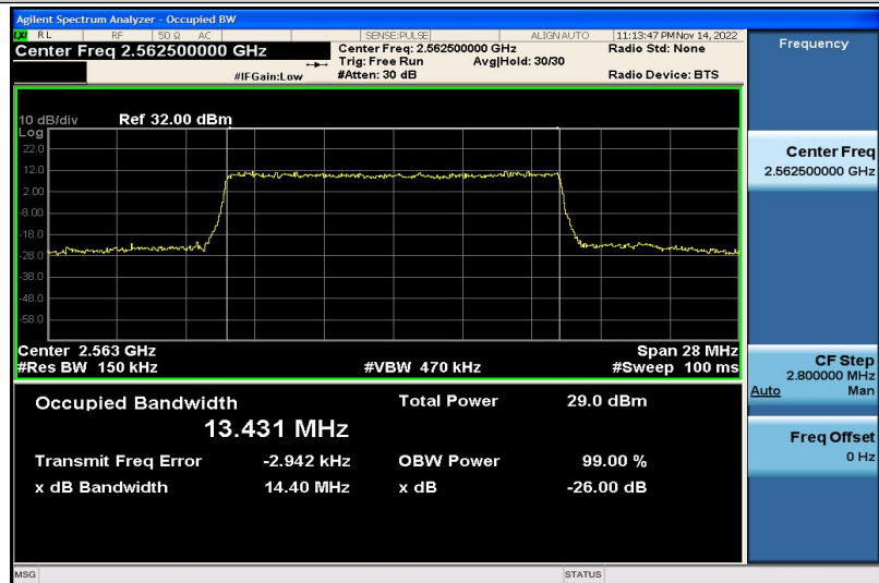
Band7-15MHz-16QAM-21375-75RB#0-13.431
