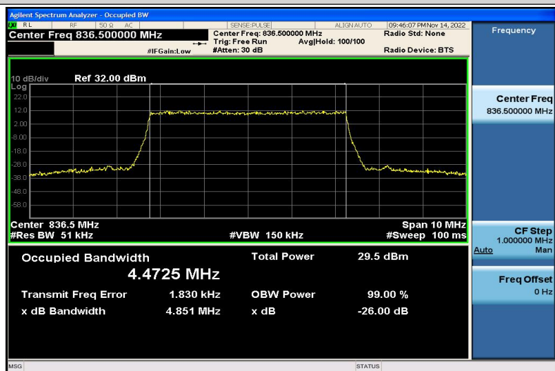
Band5-5MHz-16QAM-20525-25RB#0-4.4725
