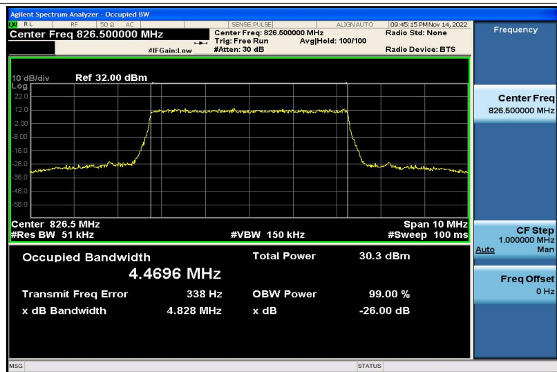
Band5-5MHz-QPSK-20425-25RB#0-4.4696
