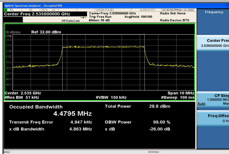
Band7-5MHz-16QAM-21100-25RB#0-4.4795
