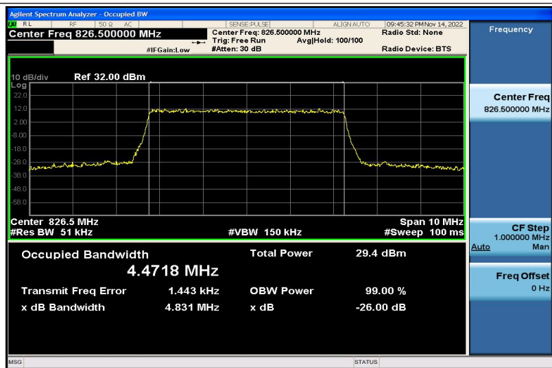
Band5-5MHz-16QAM-20425-25RB#0-4.4718
