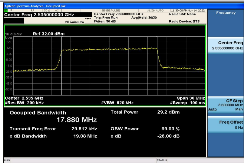
Band7-20MHz-16QAM-21100-100RB#0-17.880
