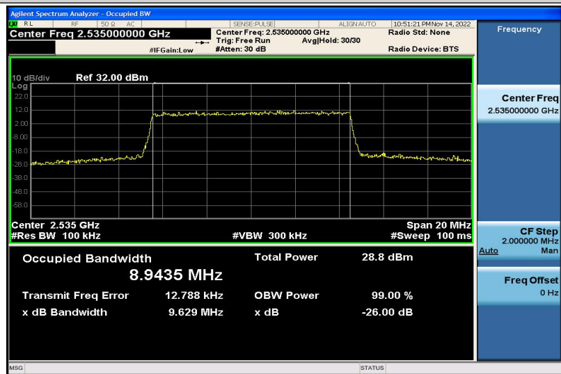
Band7-10MHz-16QAM-21100-50RB#0-8.9435
