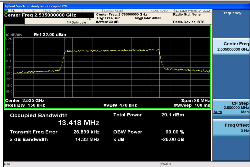
Band7-15MHz-16QAM-21100-75RB#0-13.418
