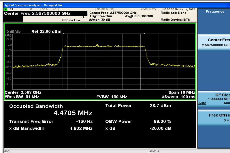
Band7-5MHz-16QAM-21425-25RB#0-4.4705
