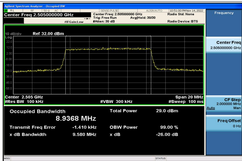
Band7-10MHz-16QAM-20800-50RB#0-8.9368
