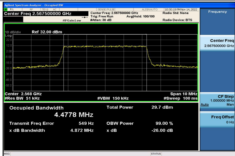
Band7-5MHz-QPSK-21425-25RB#0-4.4778
