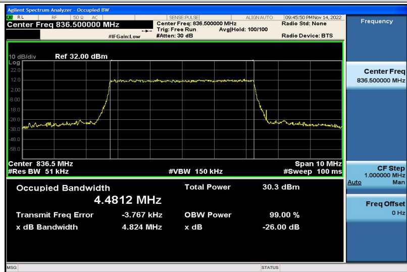
Band5-5MHz-QPSK-20525-25RB#0-4.4812
