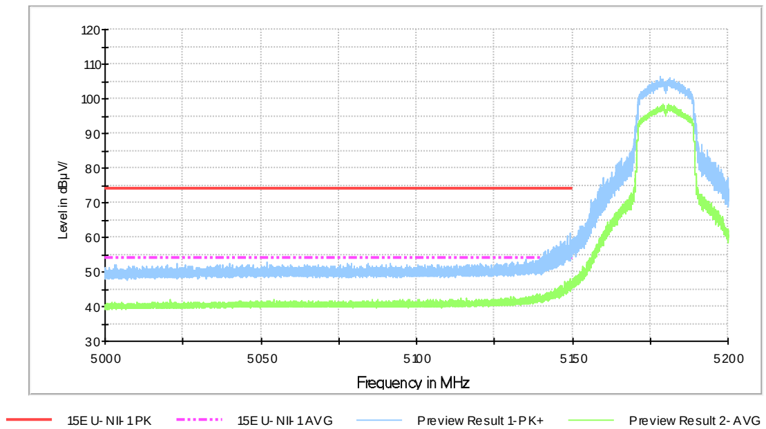
Fig.42 Band Edges (802.11ac-HT20, 5180MHz)
