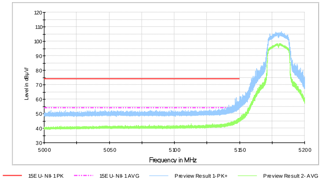
Fig.34 Band Edges (802.11a, 5180MHz)
