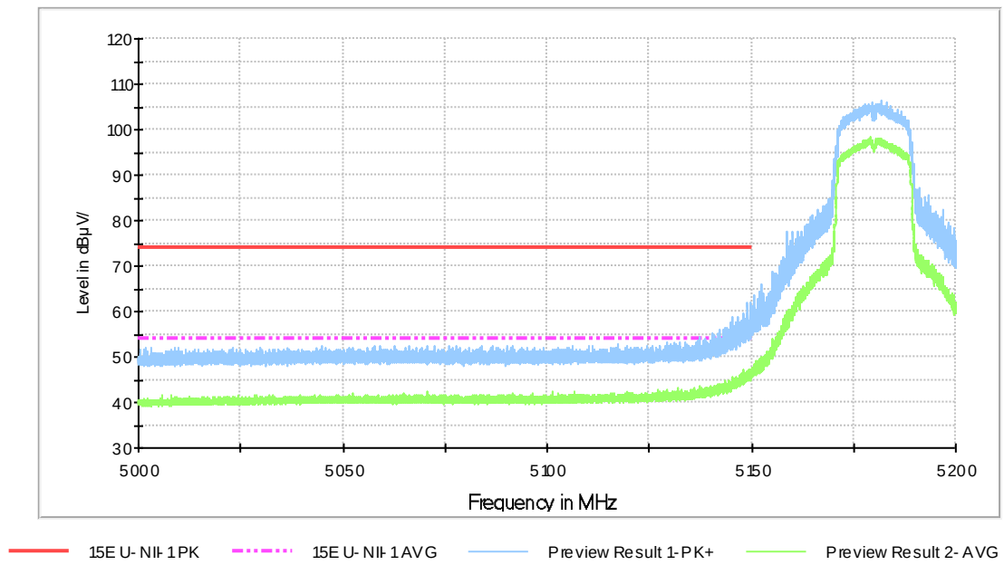
Fig.38 Band Edges (802.11n-HT20, 5180MHz)
