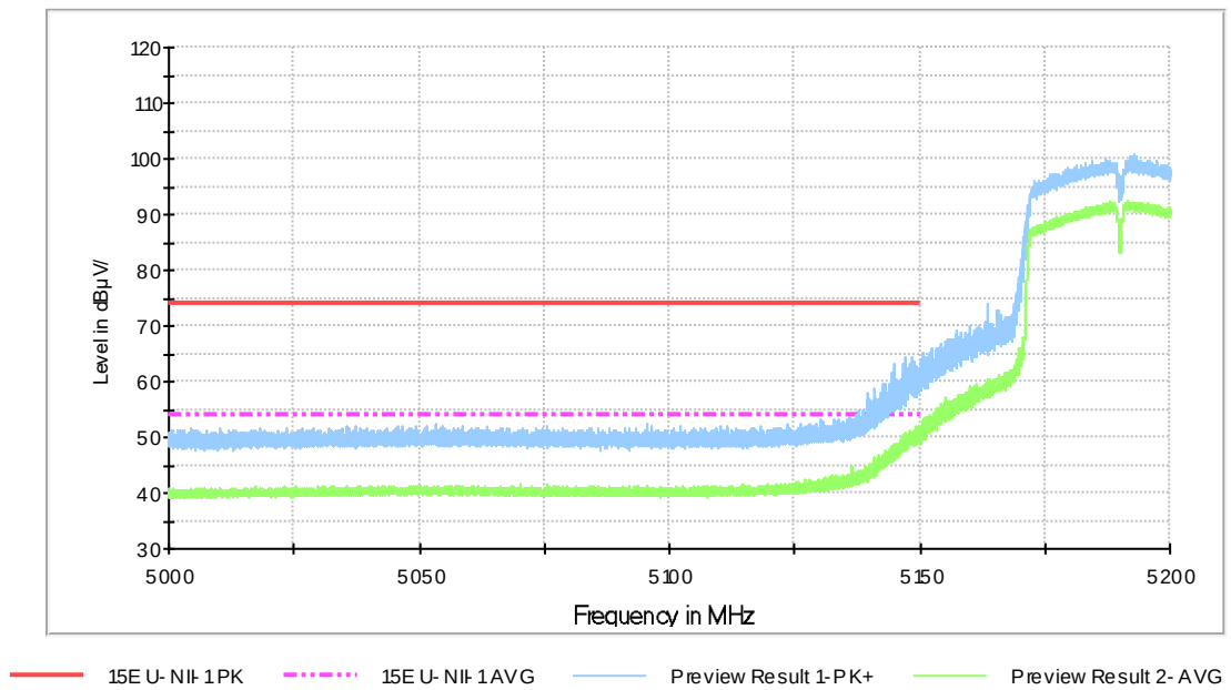
Fig.46 Band Edges (802.11n-HT40, 5190MHz)
