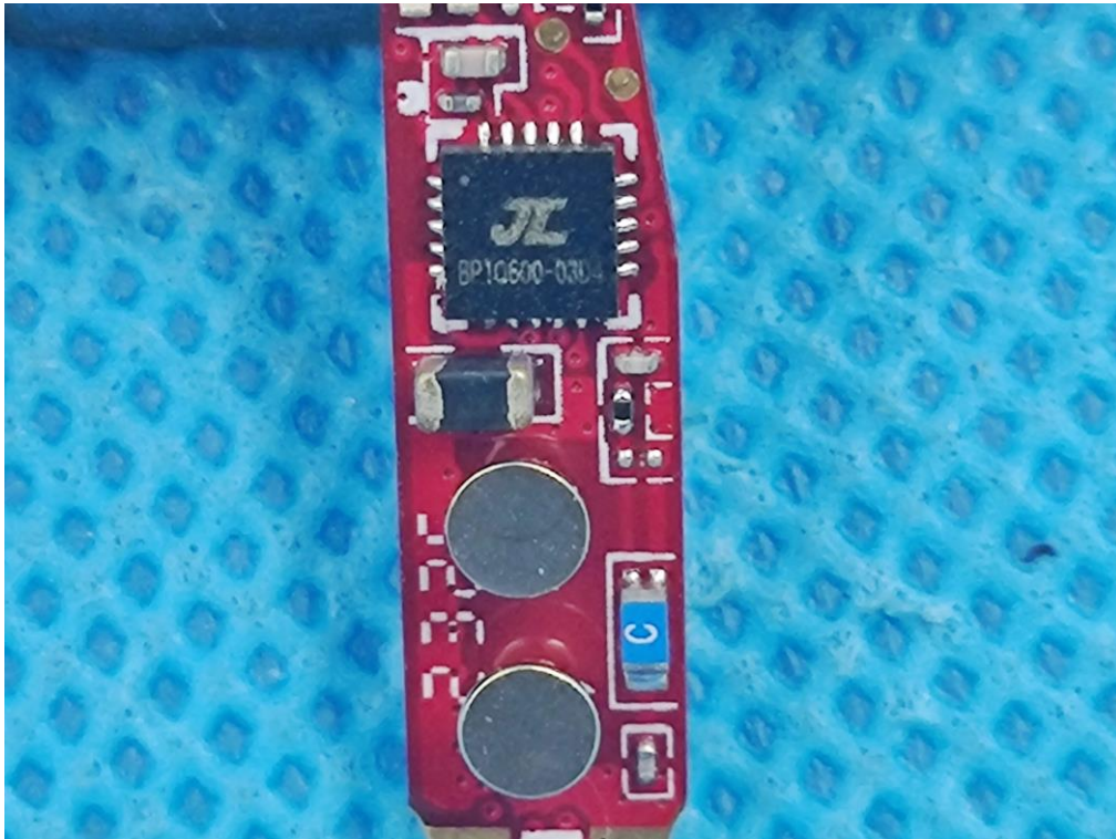
OPEN VIEW OF EUT (RIGHT HEADSET)
