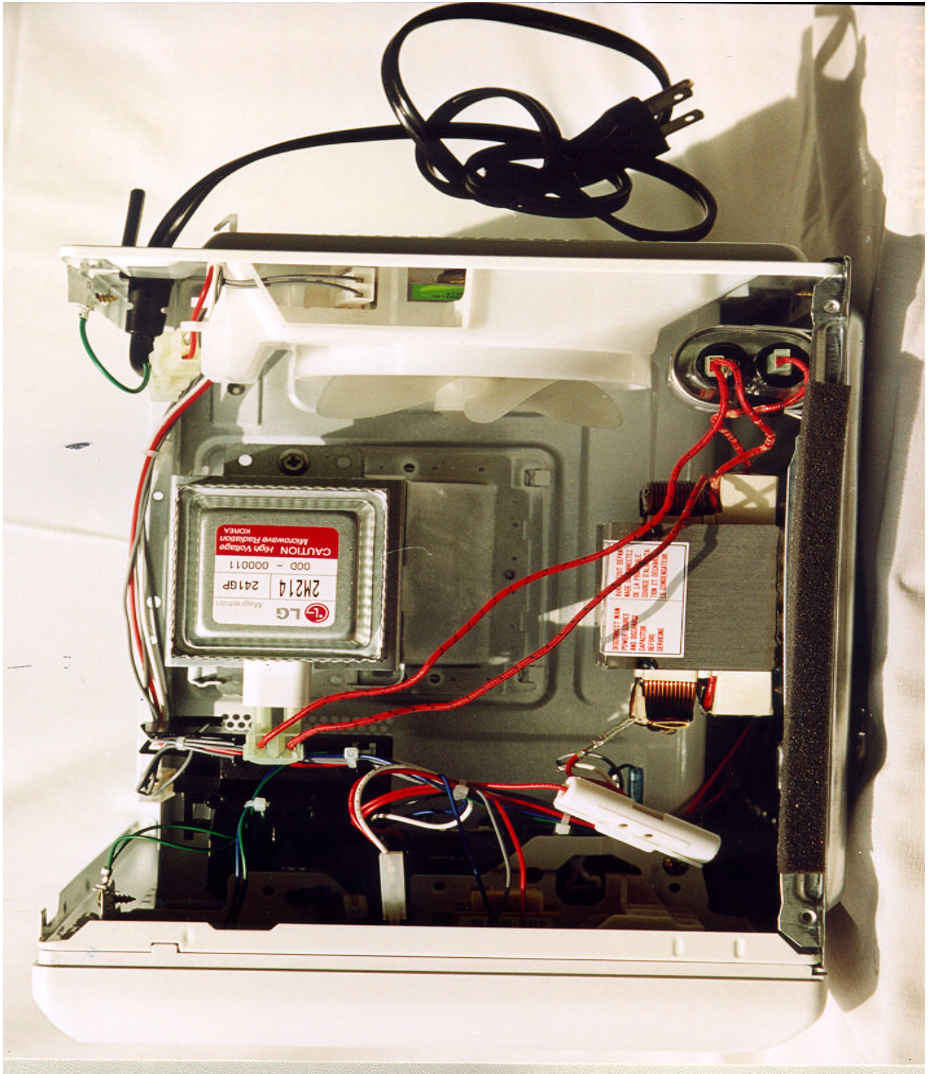
SIDE VIEW(RIGHT) – LG M.G.T.
