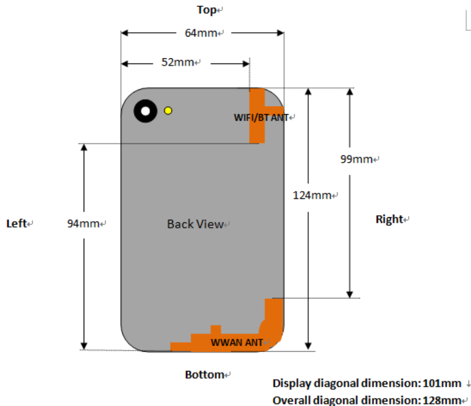
Fig.14.1 EUT Antenna Locations
