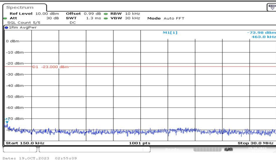
Band12-10MHz-QPSK-23060-1RB#0-Range2:0.15~30MHz-PASS
