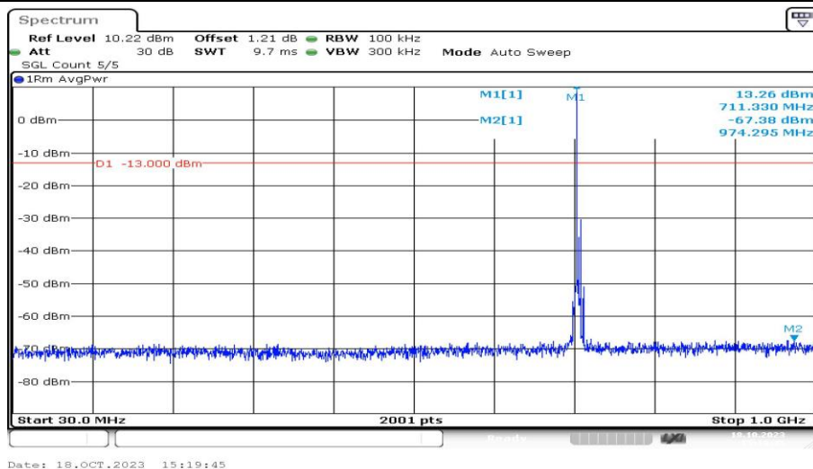
Band12-5MHz-QPSK-23155-1RB#0-Range3:30~1000MHz-PASS
