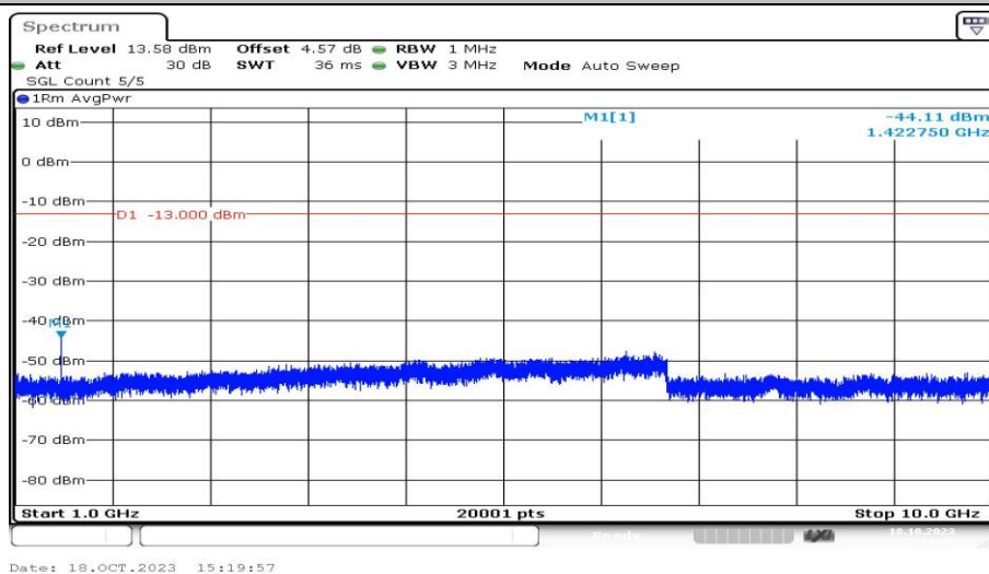
Band12-5MHz-QPSK-23155-1RB#0-Range4:1000~10000MHz-PASS
