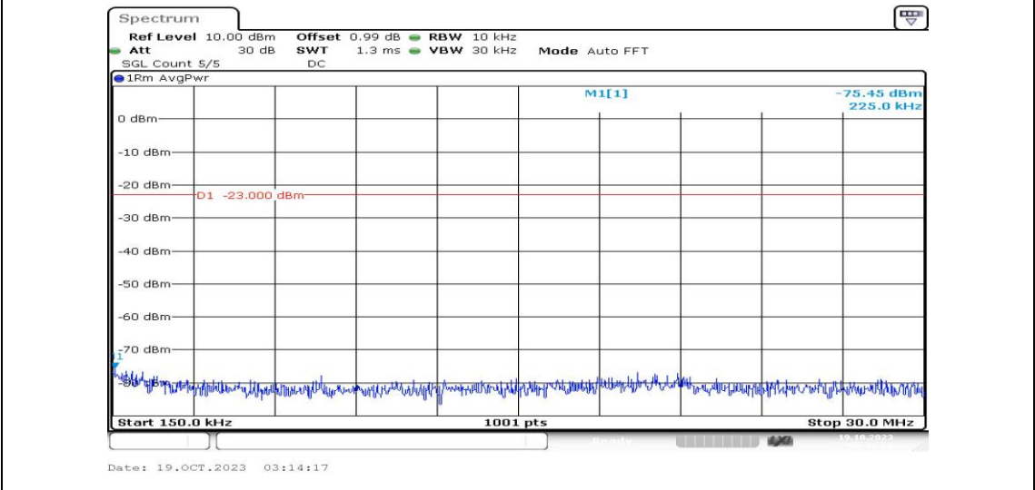
Band12-10MHz-16QAM-23130-1RB#0-Range2:0.15~30MHz-PASS
