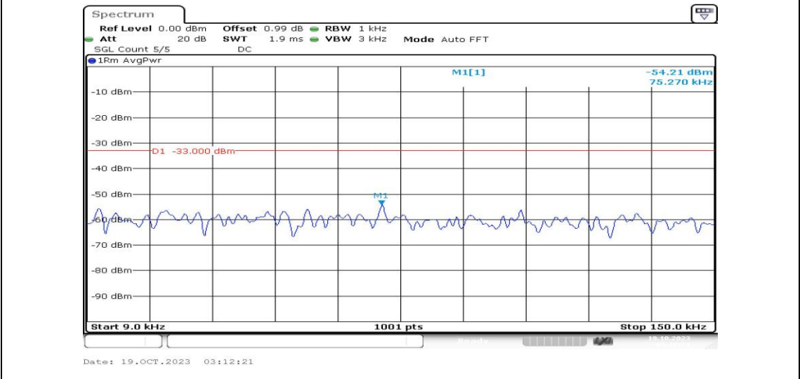
Band12-10MHz-16QAM-23060-1RB#0-Range1:0.009~0.15MHz-PASS
