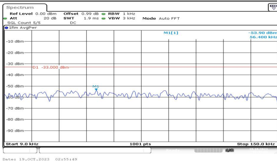
Band12-10MHz-QPSK-23095-1RB#0-Range1:0.009~0.15MHz-PASS
