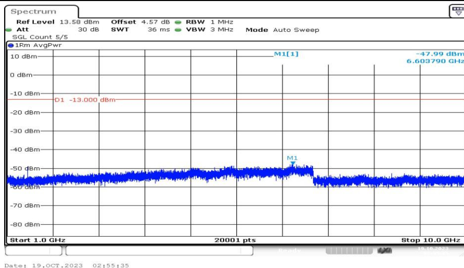
Band12-10MHz-QPSK-23060-1RB#0-Range4:1000~10000MHz-PASS
