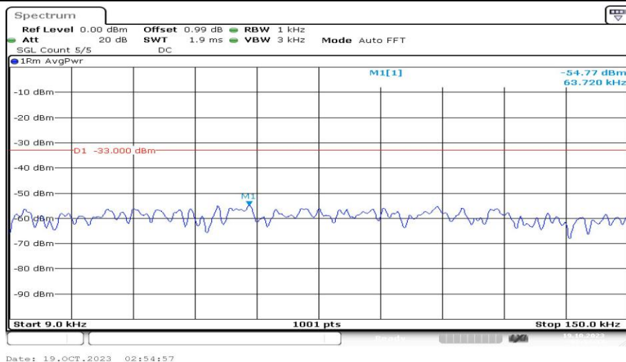
Band12-10MHz-QPSK-23060-1RB#0-Range1:0.009~0.15MHz-PASS
