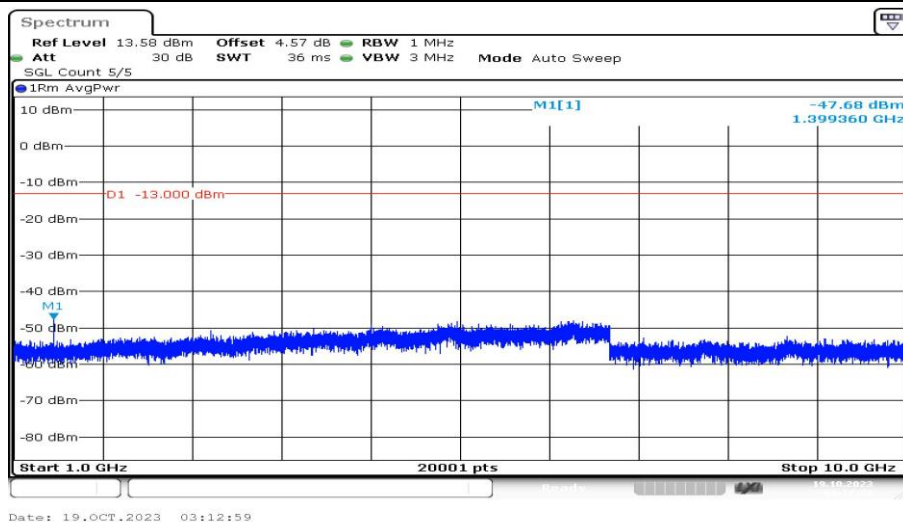
Band12-10MHz-16QAM-23060-1RB#0-Range4:1000~10000MHz-PASS
