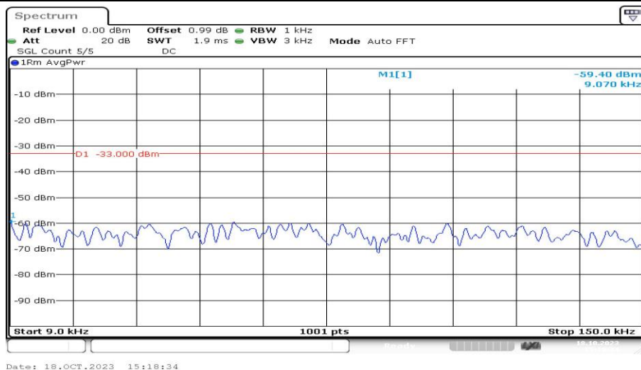
Band12-5MHz-16QAM-23095-1RB#0-Range1:0.009~0.15MHz-PASS
