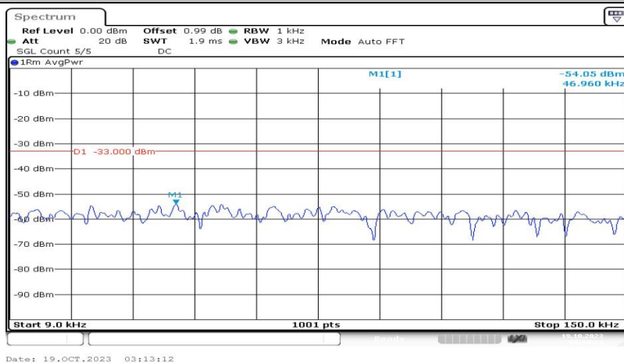
Band12-10MHz-16QAM-23095-1RB#0-Range1:0.009~0.15MHz-PASS
