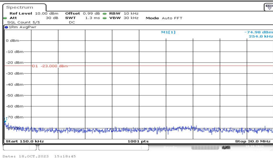
Band12-5MHz-16QAM-23095-1RB#0-Range2:0.15~30MHz-PASS
