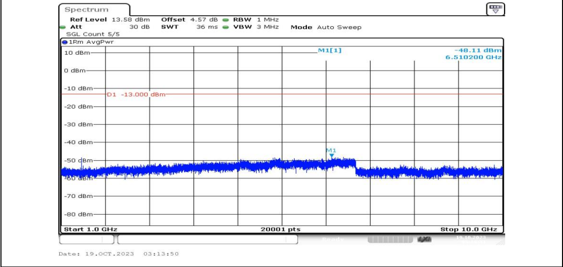
Band12-10MHz-16QAM-23095-1RB#0-Range4:1000~10000MHz-PASS
