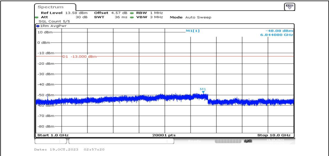
Band12-10MHz-QPSK-23130-1RB#0-Range4:1000~10000MHz-PASS
