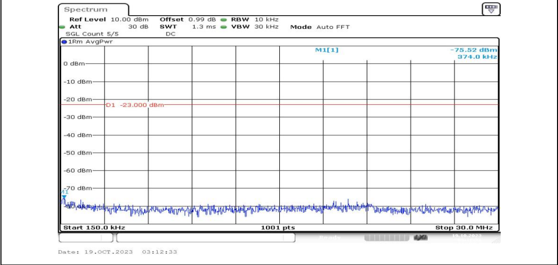
Band12-10MHz-16QAM-23060-1RB#0-Range2:0.15~30MHz-PASS
