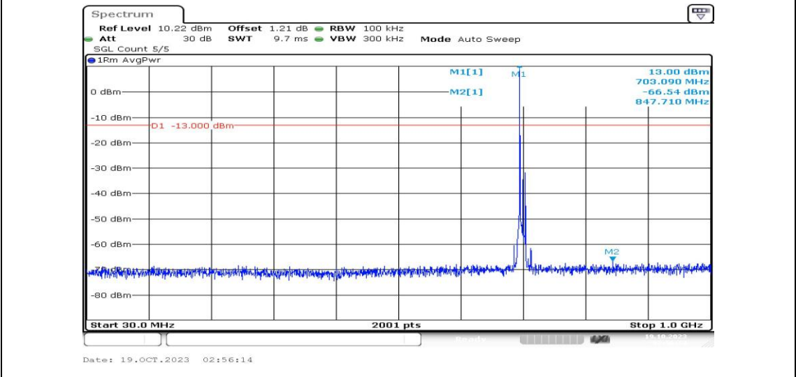
Band12-10MHz-QPSK-23095-1RB#0-Range3:30~1000MHz-PASS
