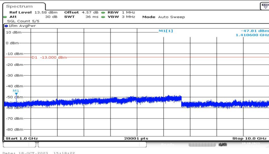
Band12-5MHz-QPSK-23095-1RB#0-Range4:1000~10000MHz-PASS
