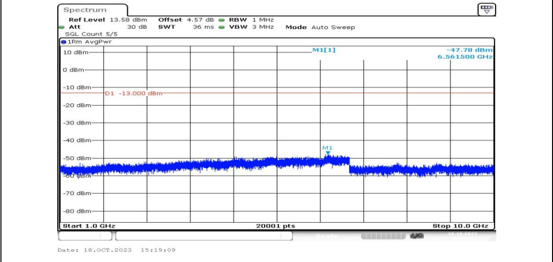
Band12-5MHz-16QAM-23095-1RB#0-Range4:1000~10000MHz-PASS
