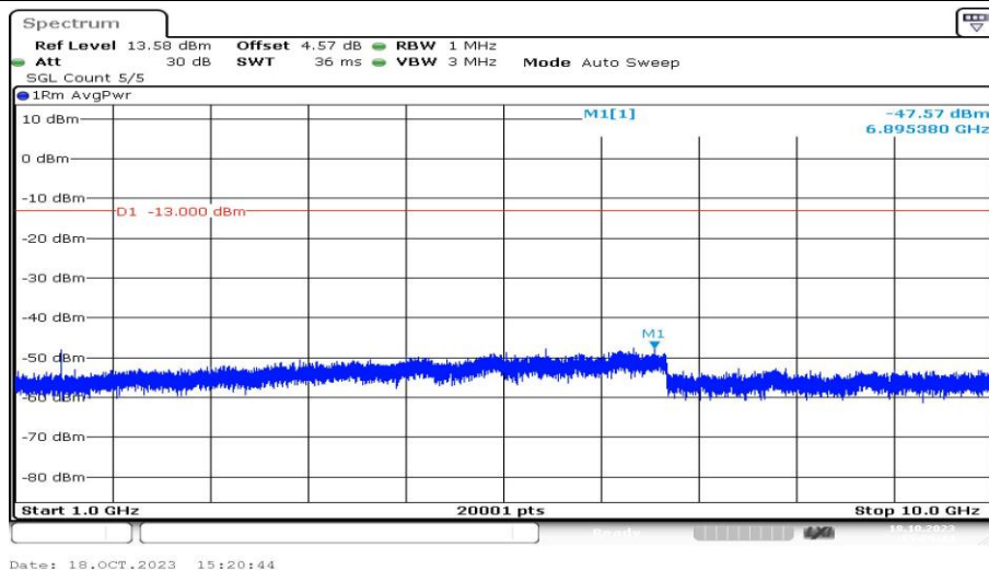
Band12-5MHz-16QAM-23155-1RB#0-Range4:1000~10000MHz-PASS
