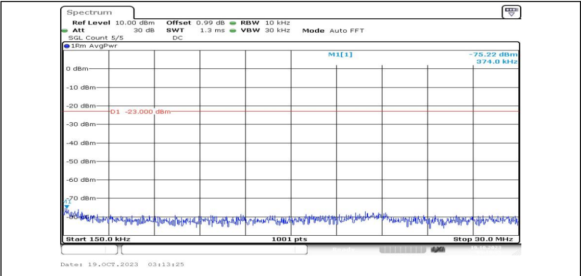
Band12-10MHz-16QAM-23095-1RB#0-Range2:0.15~30MHz-PASS
