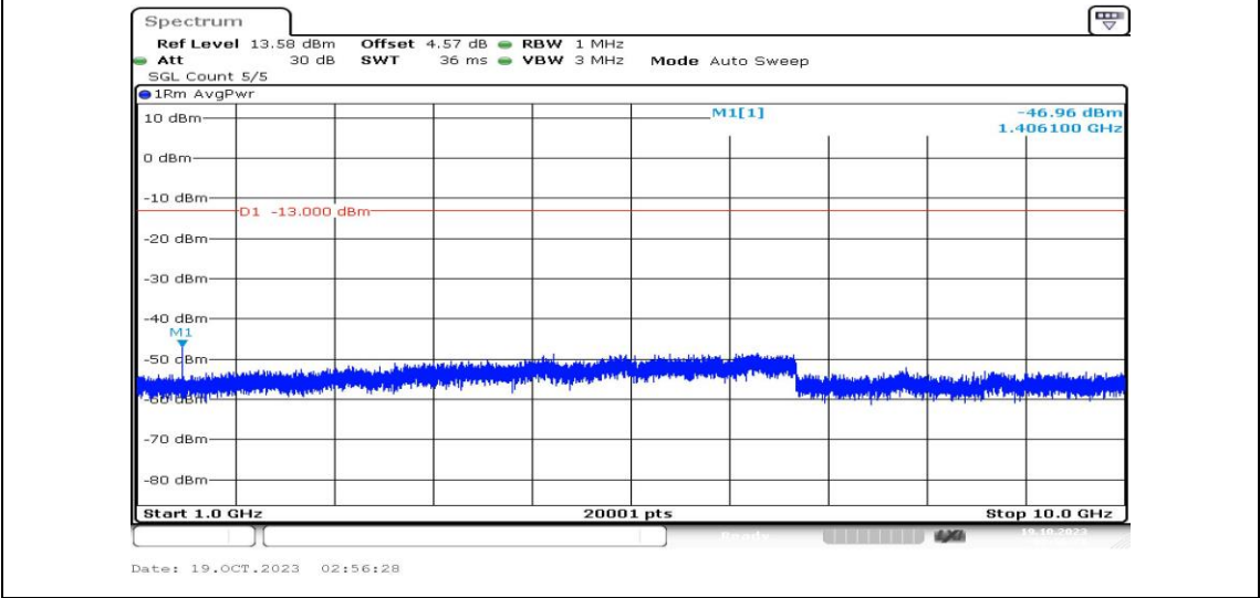
Band12-10MHz-QPSK-23095-1RB#0-Range4:1000~10000MHz-PASS
