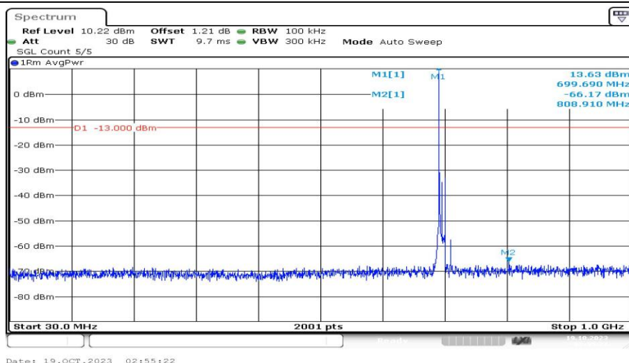
Band12-10MHz-QPSK-23060-1RB#0-Range3:30~1000MHz-PASS
