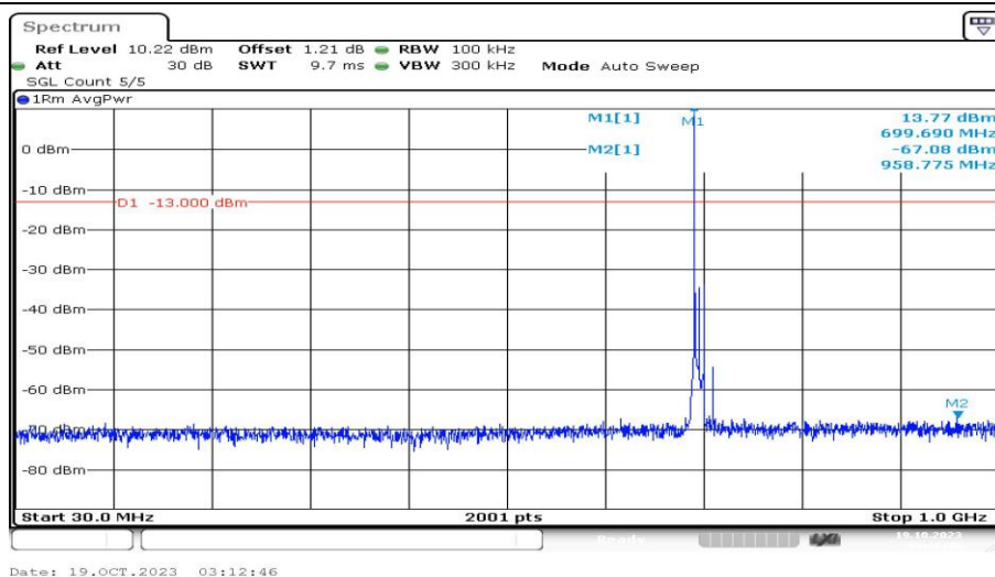
Band12-10MHz-16QAM-23060-1RB#0-Range3:30~1000MHz-PASS
