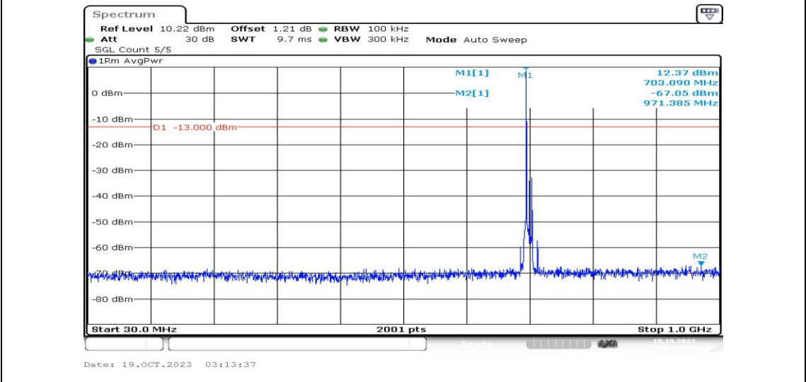
Band12-10MHz-16QAM-23095-1RB#0-Range3:30~1000MHz-PASS
