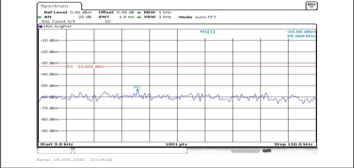
Band12-5MHz-QPSK-23155-1RB#0-Range1:0.009~0.15MHz-PASS
