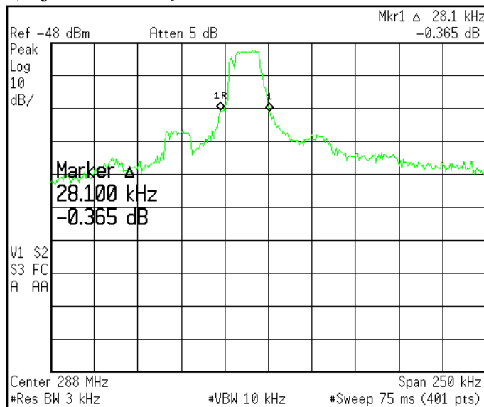
Measuring Occupied Bandwidth
