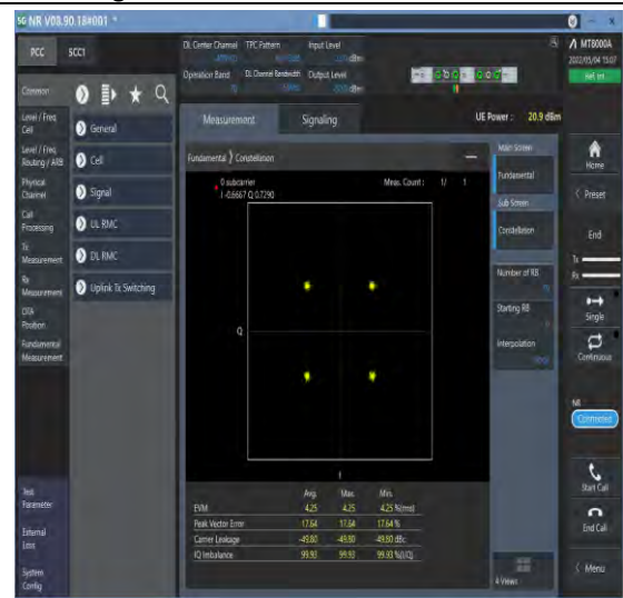
1-N70-PC3-15-15-M-6-CP-QPSK-Outer_Full-79@0- Ant1-see graph-PASS
