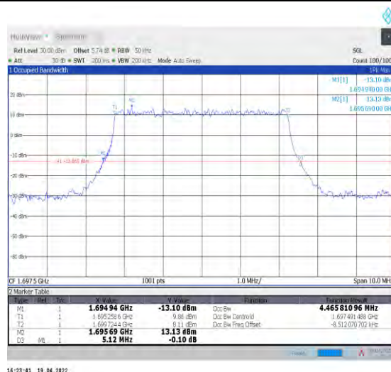
1-N70--15-5-L-2-DFT-PI2BPSK-Outer_Full-25@0-An t1-4.466-5.120-≤5-PASS
