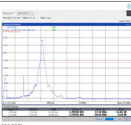
1-N70--15-5-H-2-DFT-PI2BPSK-Edge_1RB_Right-1@24-Ant1-seegraph-PASS-see graph
