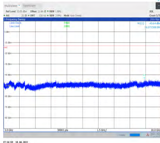
1-N70--15-15-M-1-DFT-PI2BPSK-Inner_1RB_Left-1 @1-3000-18000-Ant1--43.64--13-PASS
