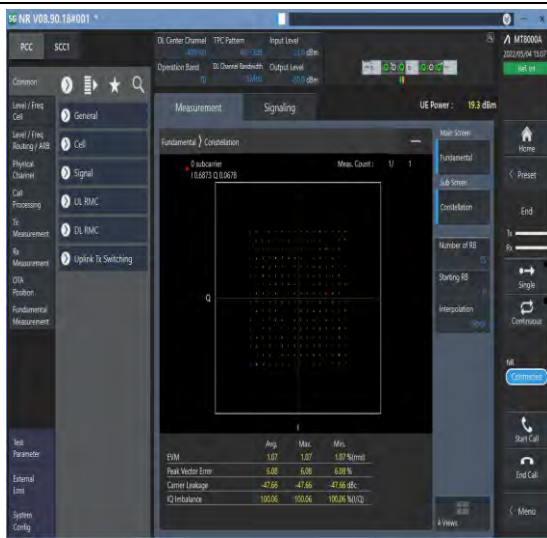
1-N70-PC3-15-15-M-5-DFT-256QAM-Outer_Full-75 @0-Ant1-see graph-PASS
