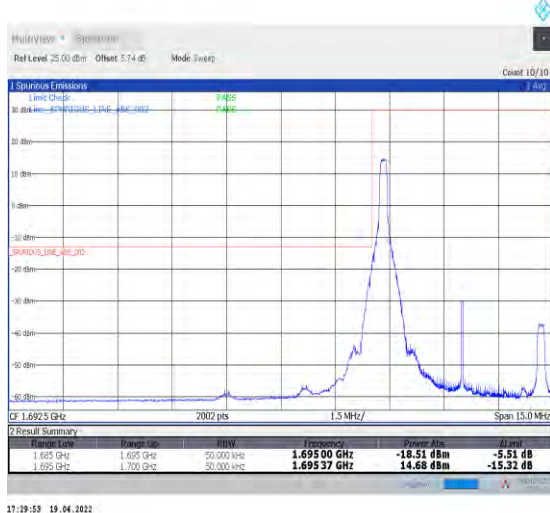
1-N70--15-5-L-4-CP-QPSK-Edge_1RB_Left-1@0-Ant1-seegraph-PASS-see graph
