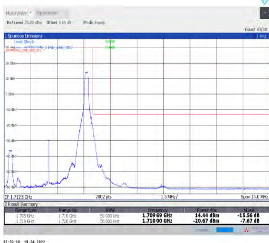
1-N70--15-5-H-5-CP-QPSK-Edge_1RB_Right-1@24-Ant1-seegraph-PASS-see graph
