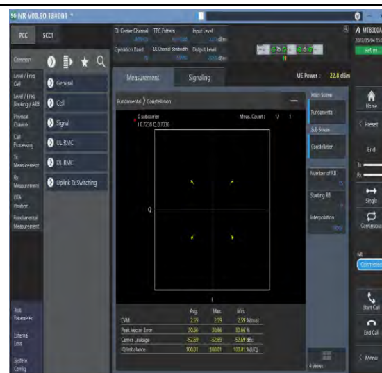
1-N70-PC3-15-15-M-2-DFT-QPSK-Outer_Full-75@ 0-Ant1-see graph-PASS
