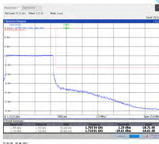
1-N70--15-5-H-6-CP-QPSK-Outer_Full-25@0-Ant1-seegraph-PASS-see graph
