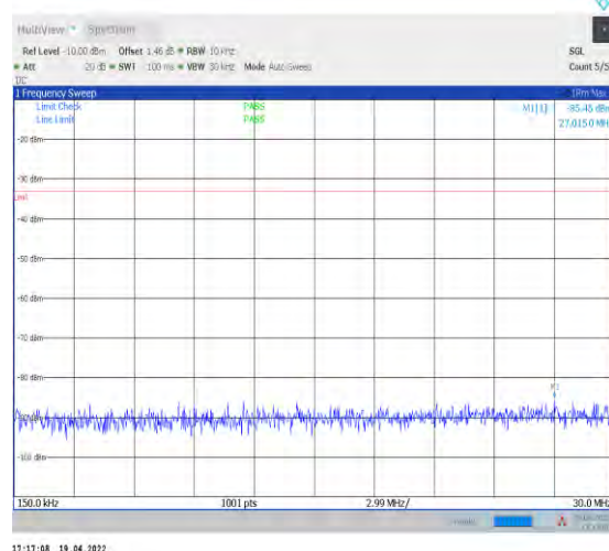
1-N70--15-15-H-1-DFT-PI2BPSK-Inner_1RB_Left-1 @1-0.15-30-Ant1--85.45--33-PASS
