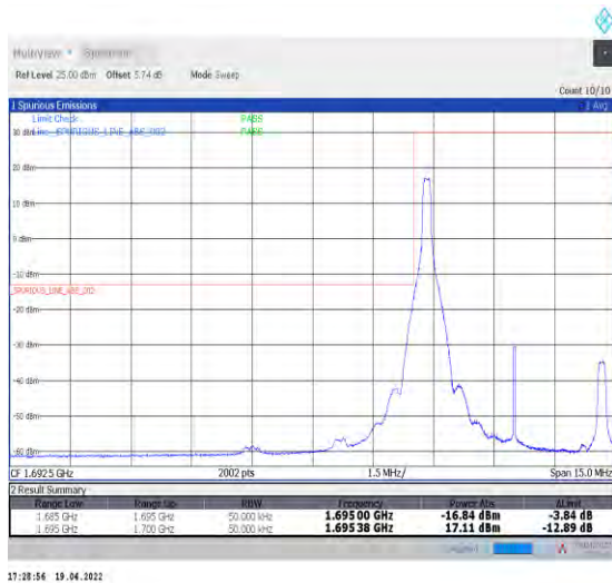
1-N70--15-5-L-1-DFT-PI2BPSK-Edge_1RB_Left-1@0-Ant1-seegraph-PASS-see graph
