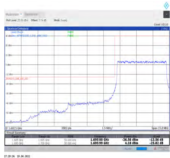
1-N70--15-5-L-3-DFT-PI2BPSK-Outer_Full-25@0-Ant1-seegraph-PASS-see graph
