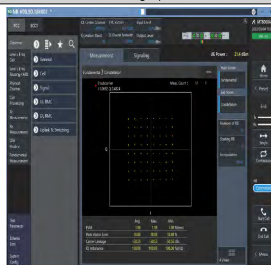
1-N70-PC3-15-15-M-4-DFT-64QAM-Outer_Full-75 @0-Ant1-see graph-PASS
