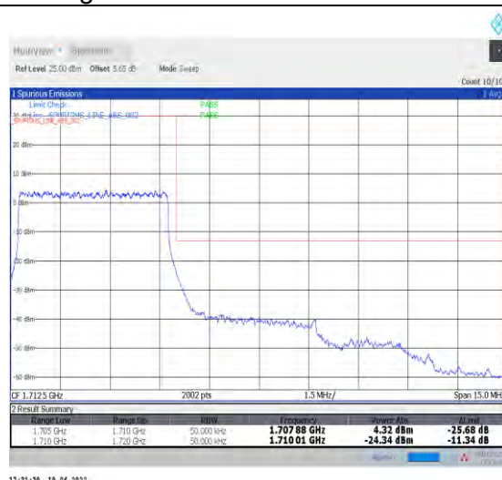
1-N70--15-5-H-3-DFT-PI2BPSK-Outer_Full-25@0-Ant1-seegraph-PASS-see graph
