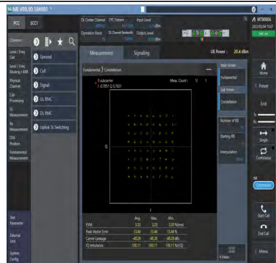
1-N70-PC3-15-15-M-8-CP-64QAM-Outer_Full-79@ 0-Ant1-see graph-PASS
