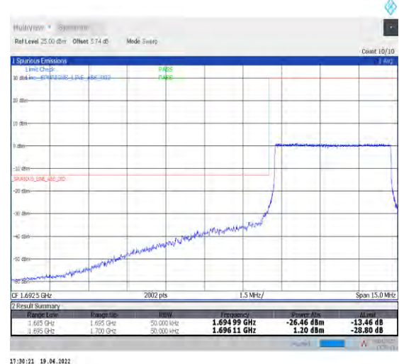
1-N70--15-5-L-6-CP-QPSK-Outer_Full-25@0-Ant1-seegraph-PASS-see graph
