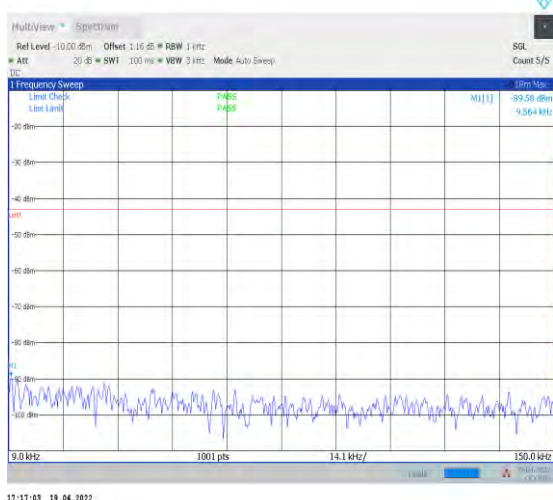
1-N70--15-15-H-1-DFT-PI2BPSK-Inner_1RB_Left-1 @1-0.009-0.15-Ant1--89.58--43-PASS
