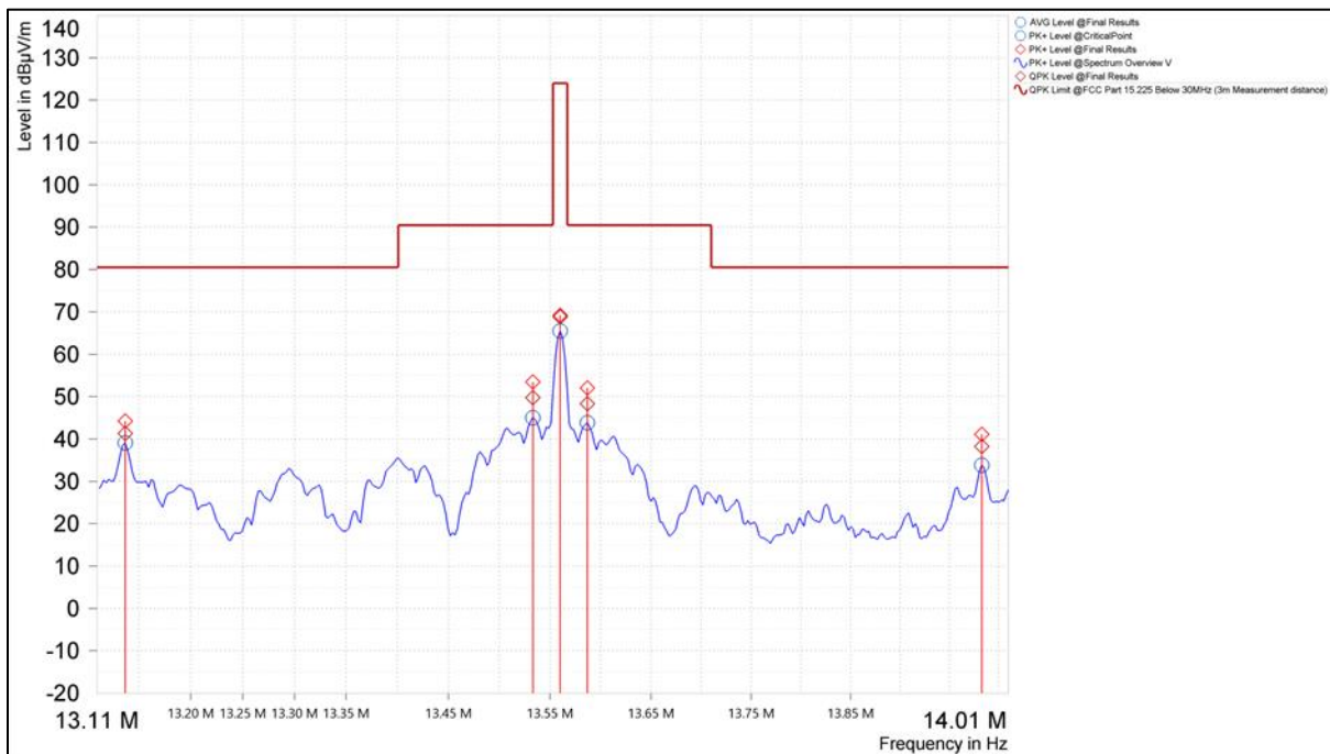
Figure 16. In-Band Emission Mask (Coaxial Loop, Small HF Antenna)
