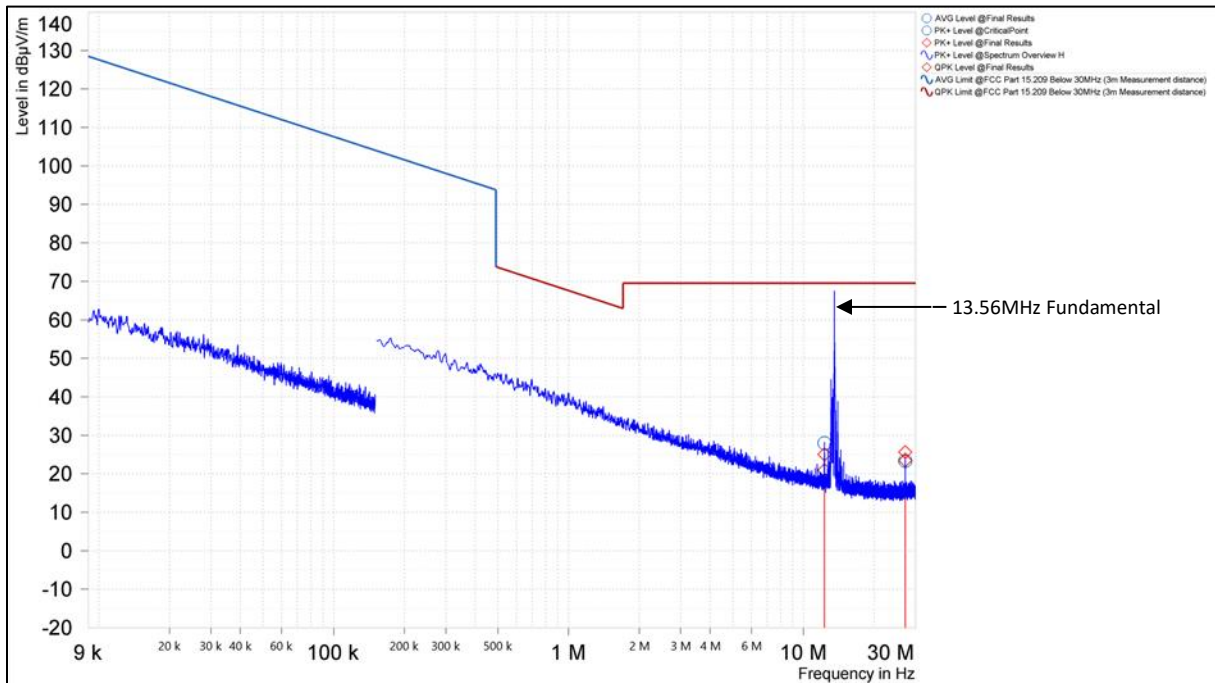
Figure 17. Out of Band Emissions Below 30MHz (Coplanar Loop, Small HF Antenna)
