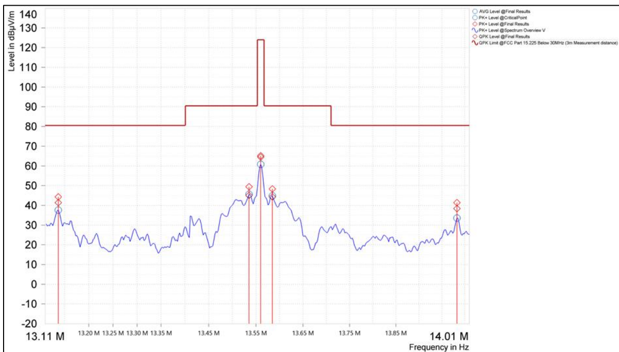
Figure 28. In-Band Emission Mask (Coaxial Loop, Combined HF Antenna)
