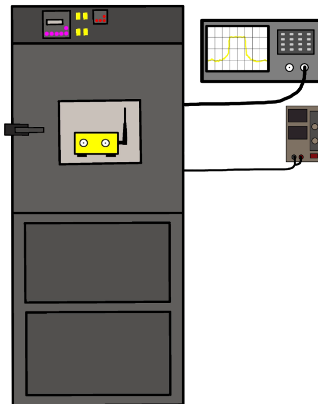
Figure 33. Temperature Stability Test Setup
