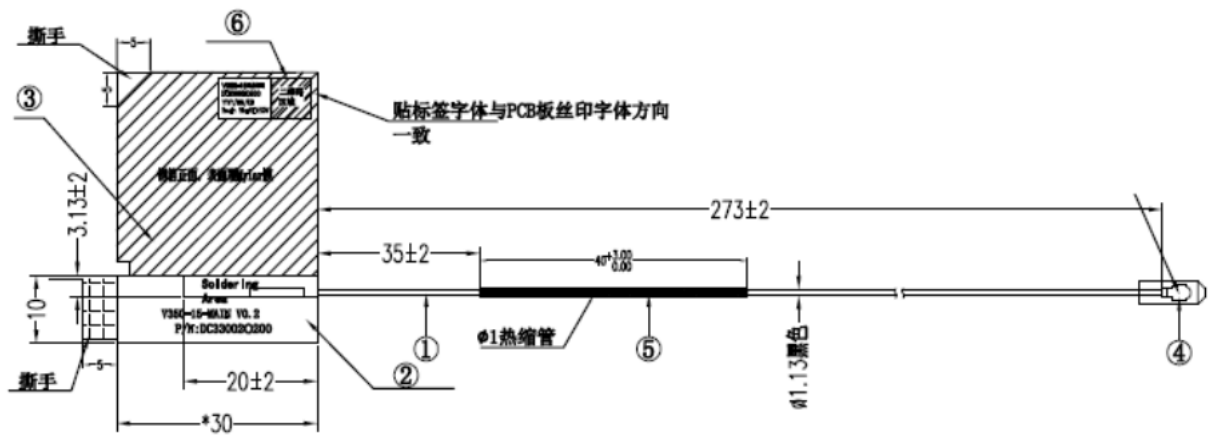
Main Antenna Drawing:
