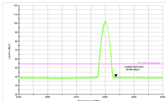
3DH5-Channel 78: Average
