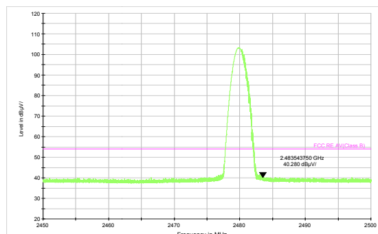
DH5-Channel 78: Average
